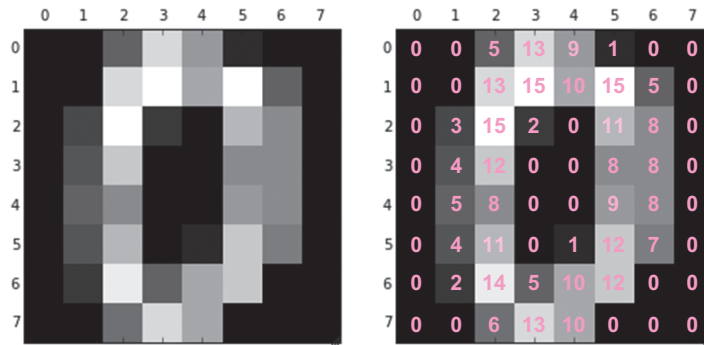
Figure 3.5 We'll turn an image into something usable by the Naïve Bayes classifier by getting the grayscale value for each of its pixels (shown on the right) and putting those values in a list.
