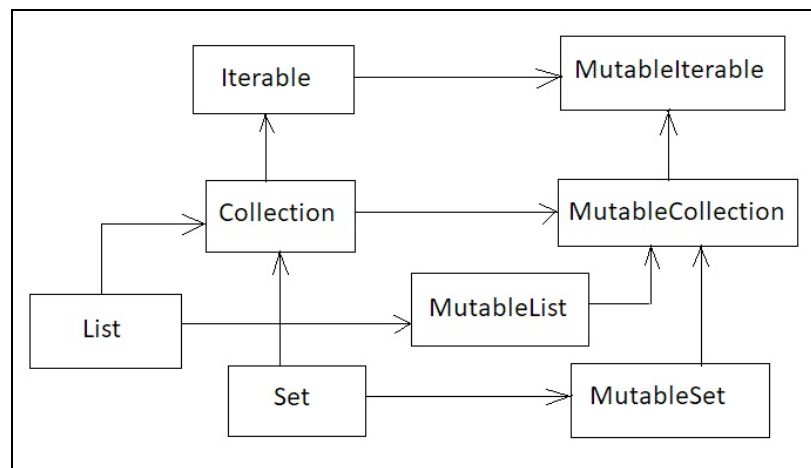
Kotlin collection interfaces hierarchy
