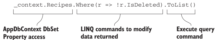
Figure 12.13 The three parts of an EF Core database query.
