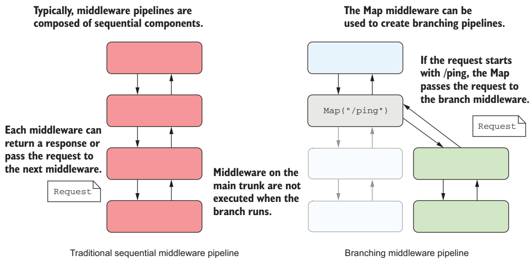
Figure 19.1 A sequential middleware pipeline compared to a branching pipeline created with the Map extension. In branching middleware, requests only pass through one of the branches at a time. Middleware on the other branch never see the request and aren't executed.
