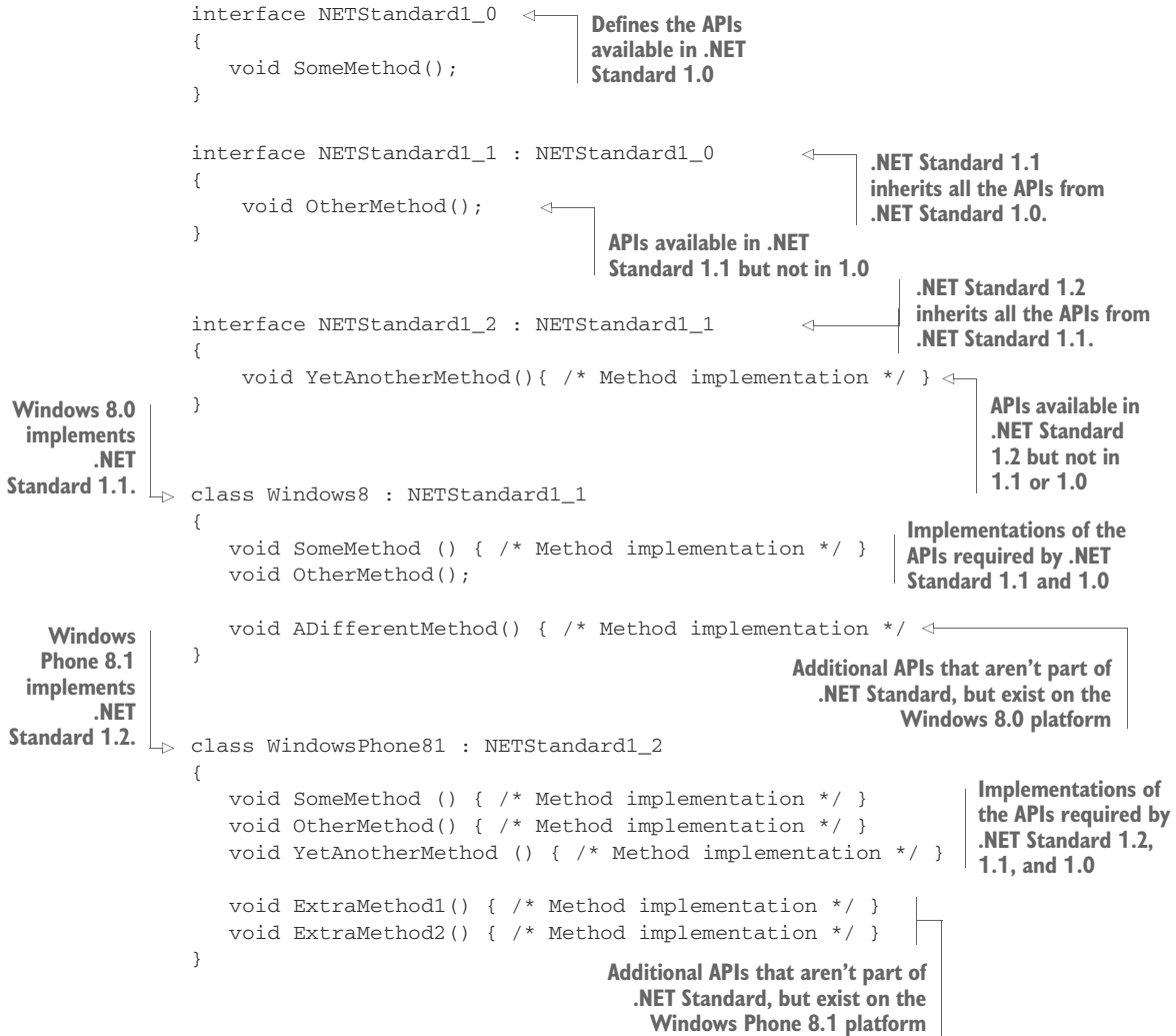
Listing A.1 An interpretation of .NET Standard in C#
