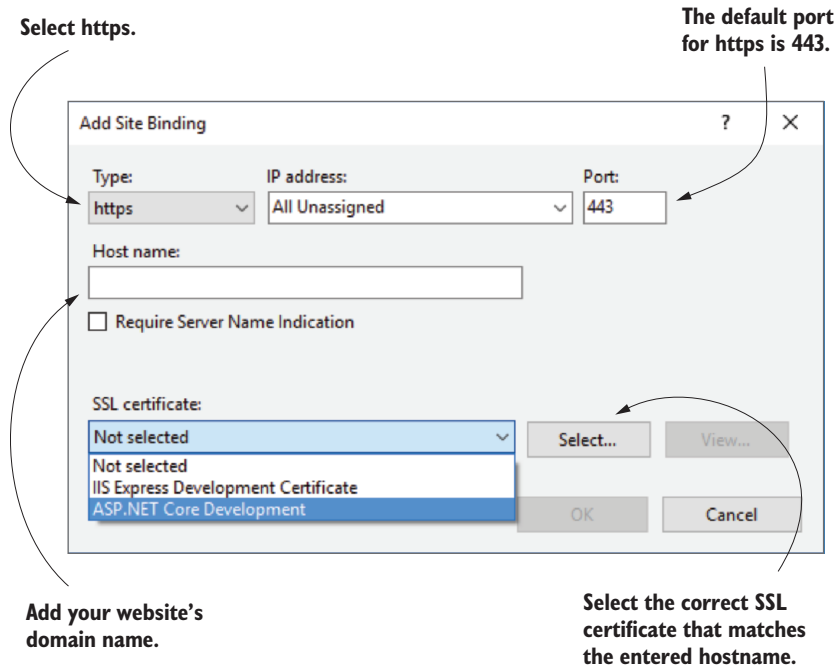
Figure 18.4 The Add Site Binding screen in IIS. When you select an HTTPS binding, IIS terminates the SSL for your app, serving your app over HTTPS without having to change any app code.
