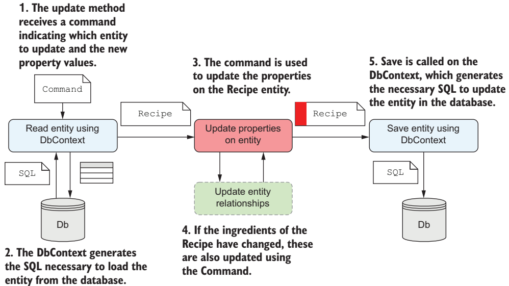
Figure 12.14 Updating an entity involves three steps: read the entity using EF Core, update the properties of the entity, and call SaveChanges() on the DbContext to generate the SQL to update the correct rows in the database.
