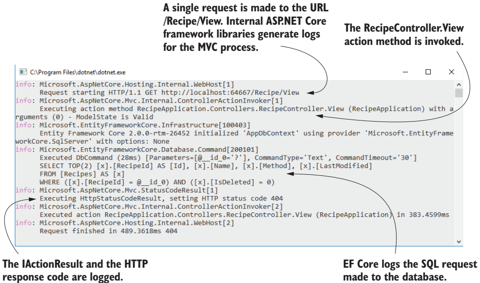
Figure 17.1 The ASP.NET Core Framework libraries use logging throughout. A single request generates multiple log messages that describe the flow of the request through your application.
