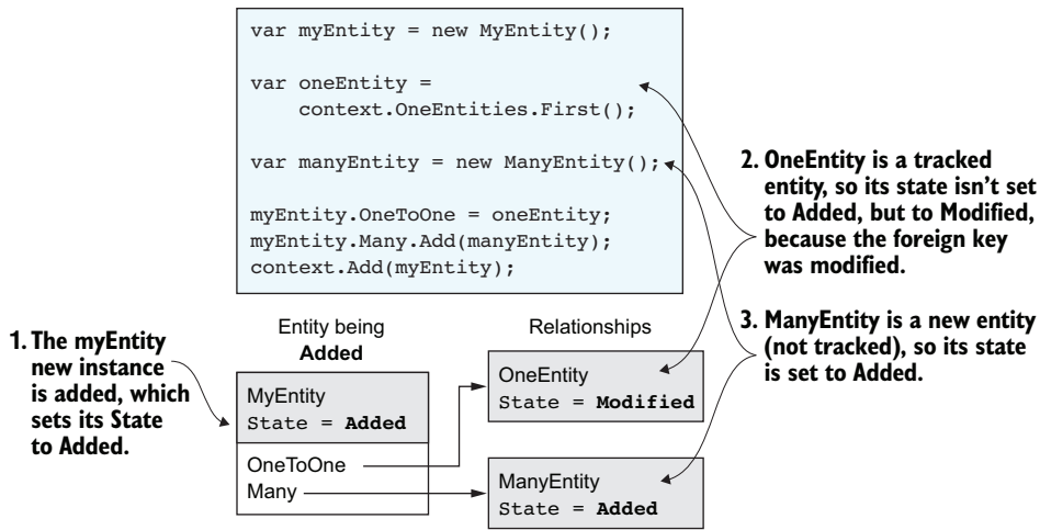
Figure 9.3 Adding an entity with both an is tracked and a not tracked relationship. The is tracked case is shown in step 2: a tracked OneEntity instance is set to Modified because a foreign key in that entity was set. The not tracked case is shown in step 3: a new ManyEntity entity instance is added to the myEntity 's entity instance Many collection navigational property.
