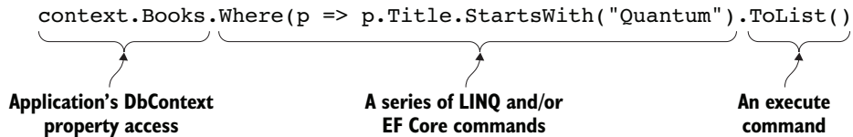
Figure 2.7 The three parts of an EF Core database query, with example code
