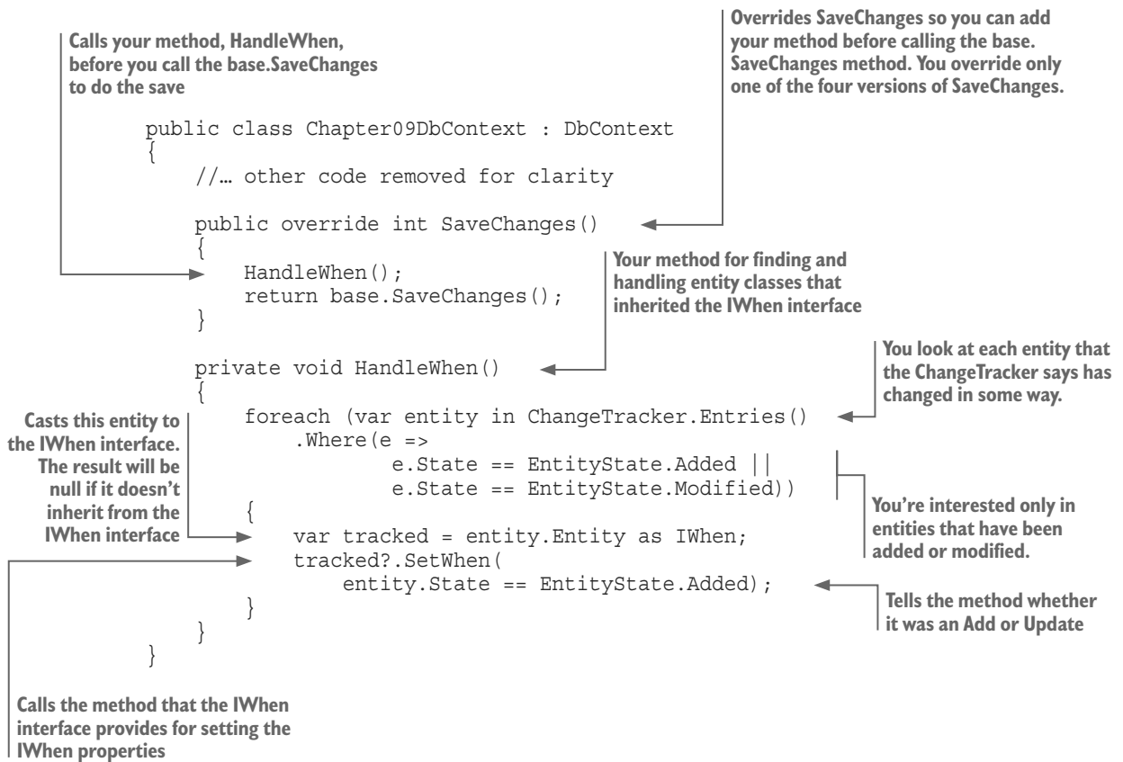
Listing 9.8 Your DbContext looks for added or modified IWhen entities
