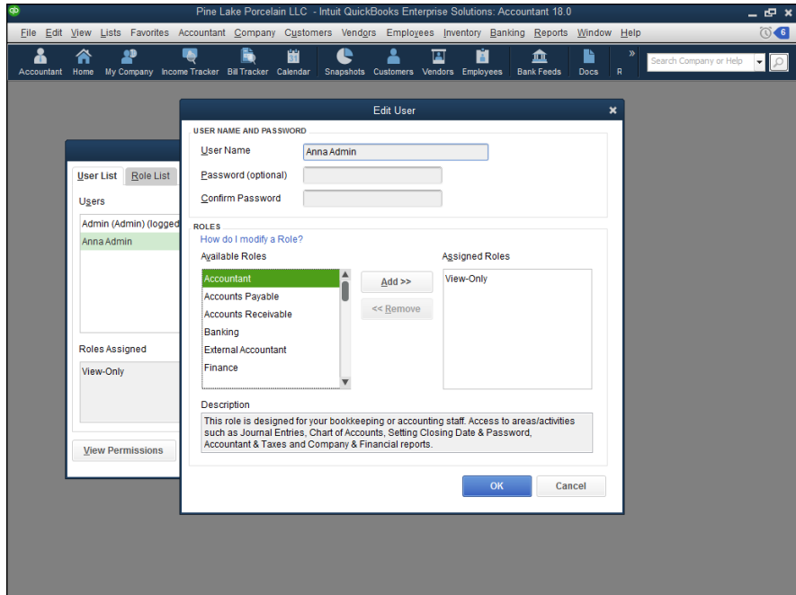
FIGURE 1-7: The Edit User dialog box.
