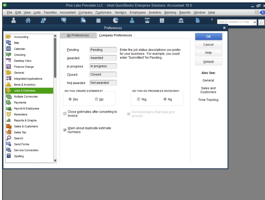
FIGURE 3-12: The Company Preferences tab of the Jobs & Estimates Preferences dialog box.
