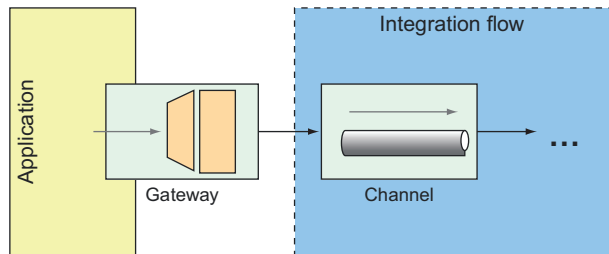
Figure 9.8 Service gateways are interfaces through which an application can submit messages to an integration flow.
