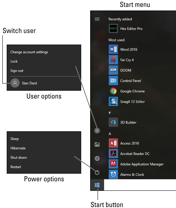
FIGURE 9-1: Power options.
