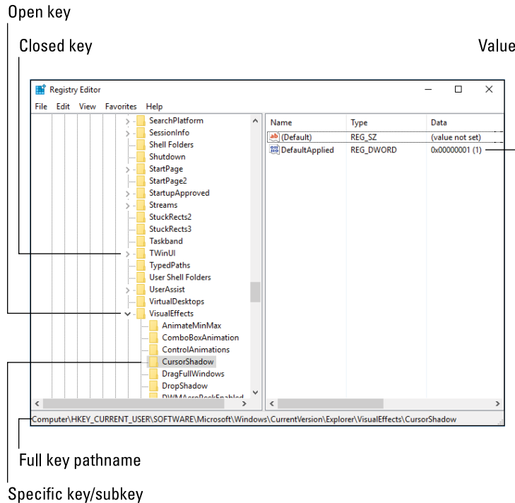
FIGURE 7-1: The Registry Editor.
