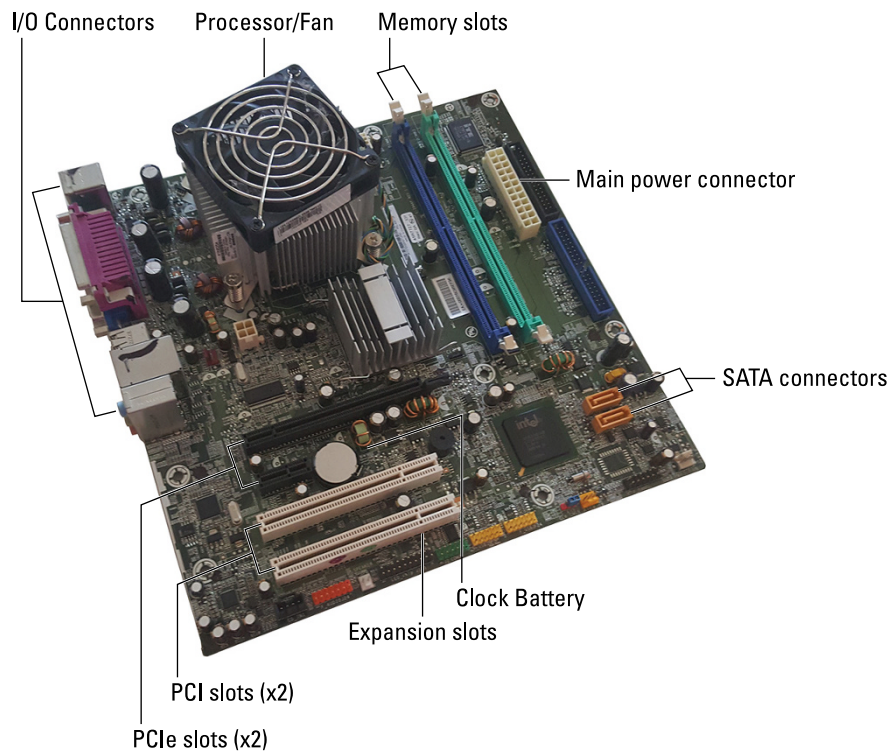
FIGURE 4-2: A typical motherboard.
