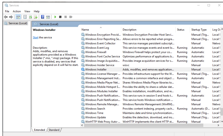
FIGURE 6-4: The Services console.
