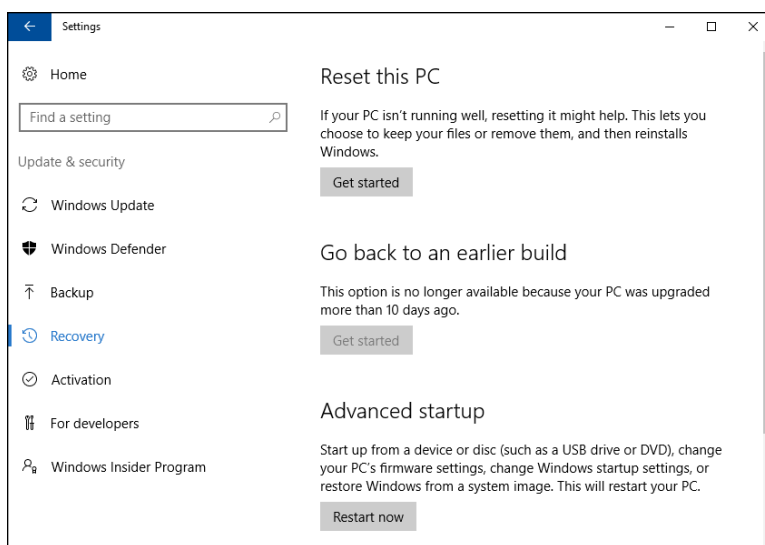
FIGURE 1-1: Windows Recovery Environment options.
