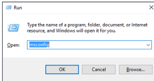
FIGURE 3-1: The Run dialog box.
