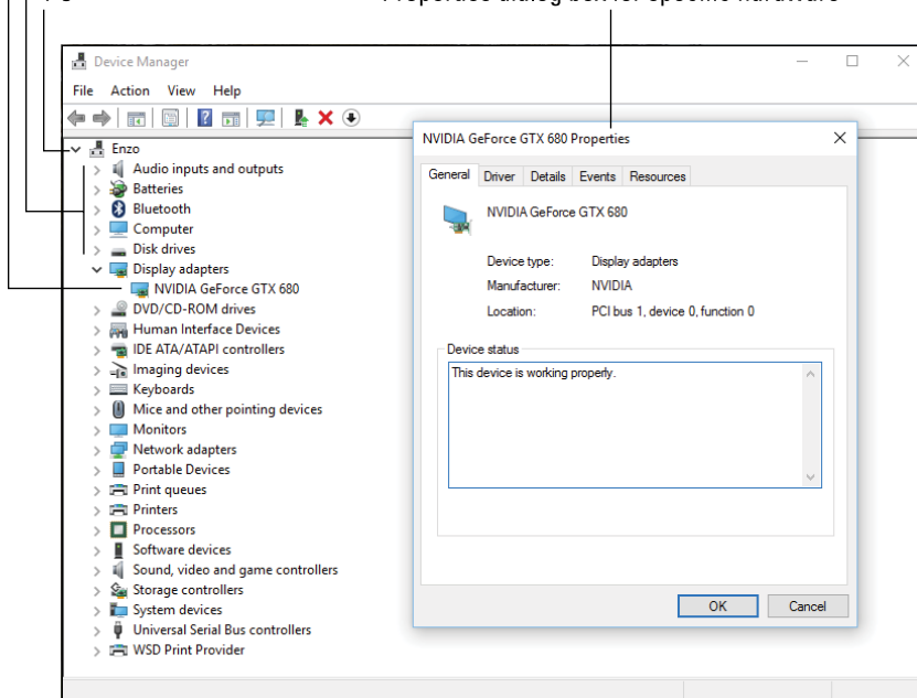
FIGURE 2-1: The Device Manager.
