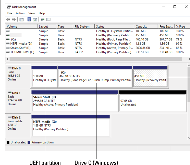
FIGURE 1-2: The Disk Management console.
