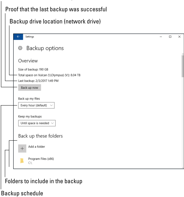
FIGURE 3-1: The Backup Options screen.
