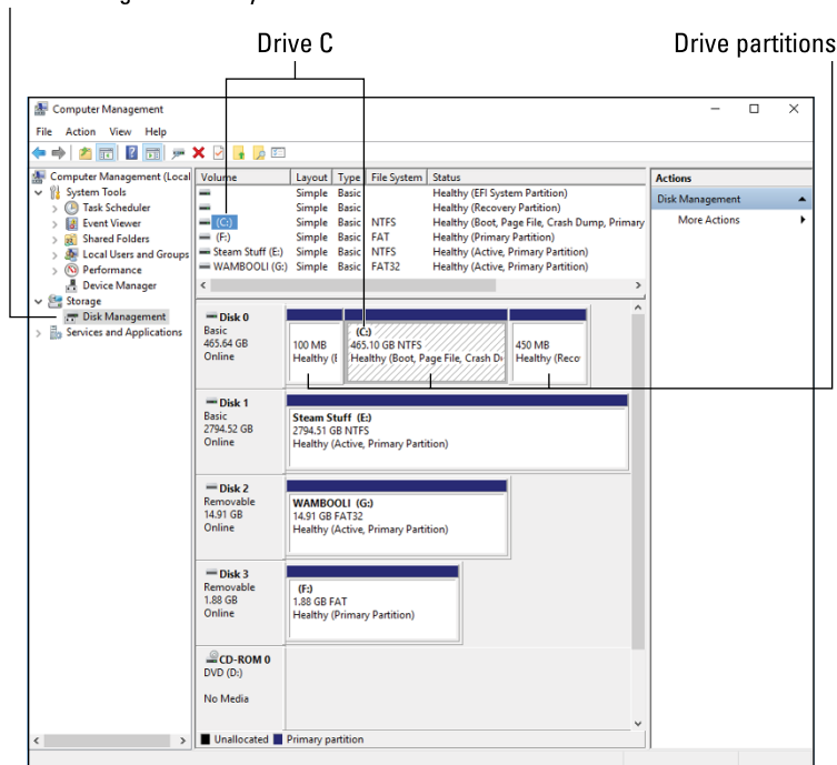
FIGURE 2-6: The Disk Management console.
