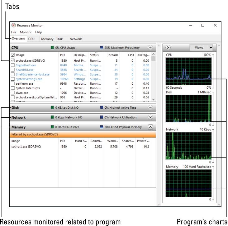
FIGURE 1-3: The Resource Monitor.
