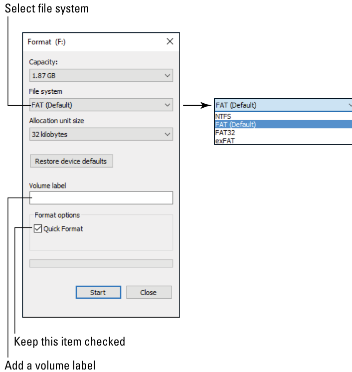
FIGURE 2-11: The Format dialog box.
