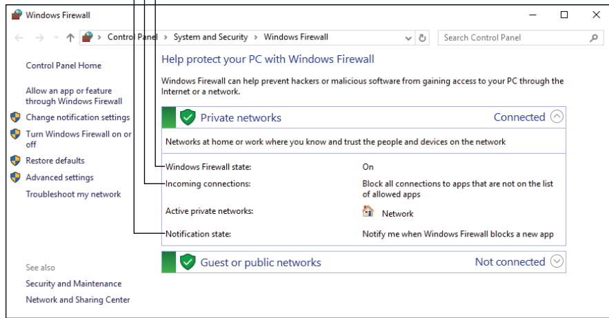
FIGURE 2-3: Windows Firewall.
