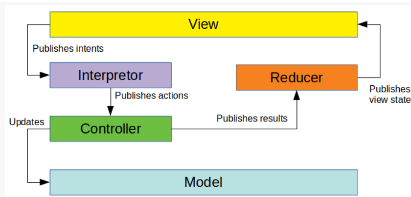
Figure 8: Model-View-Intent, With Actual Intents
