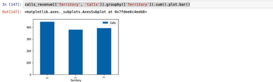
Figure 24.3 Bar plot of a pandas data frame in Jupyter notebook
