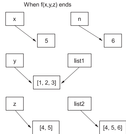
Figure 9.2 At the end of function f() , y ( list1 inside the function) has changed internally, whereas n and list2 refer to different objects.
