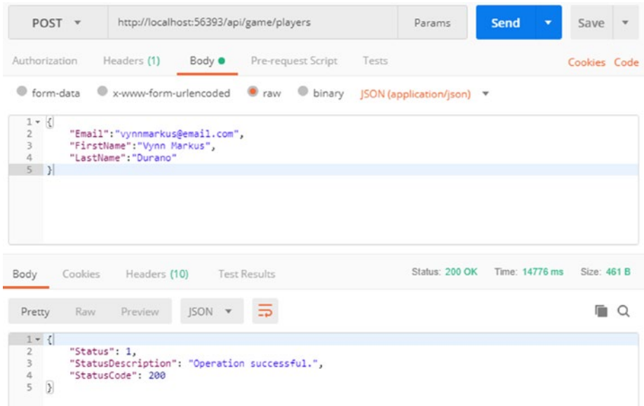
Figure 3-11. Testing an API with Postman
