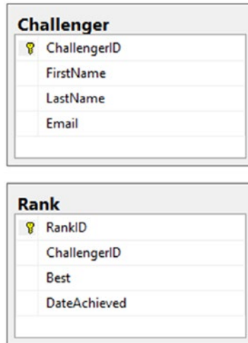
Figure 3-3. The database schema
