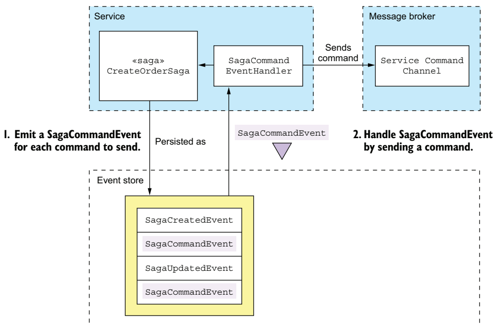
Figure 6.13 How an event sourcing-based saga orchestrator sends commands to saga participants
