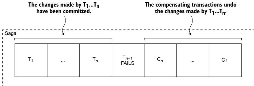
Figure 4.3 When a step of a saga fails because of a business rule violation, the saga must explicitly undo the updates made by previous steps by executing compensating transactions.
