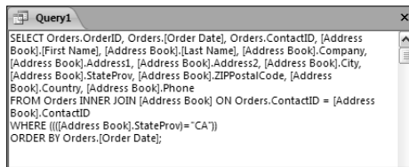
Figure 5-4: Sample SQL statement produced by a query.
