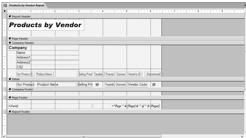
Figure 1-13: Report sections determine what prints at the beginning and end of the report, in each section of the report, and at the top and bottom of the page.
