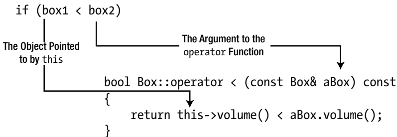
Figure 12-1. Overloading the less-than operator
