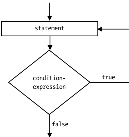
Figure 6-5. The flow diagram for a do-while statement
