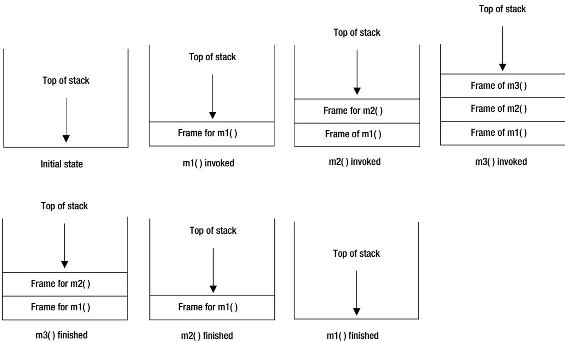
Figure 13-5. State of the stack of a thread when methods m1() , m2() , and m3() are called
