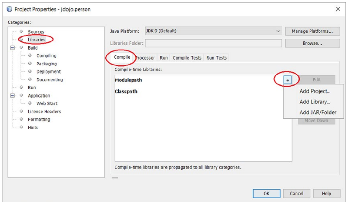
Figure 10-3. Setting the module path for a project in NetBeans
