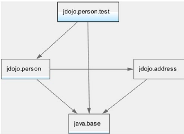
Figure 10-6. The module graph for the jdojo.person.test module
