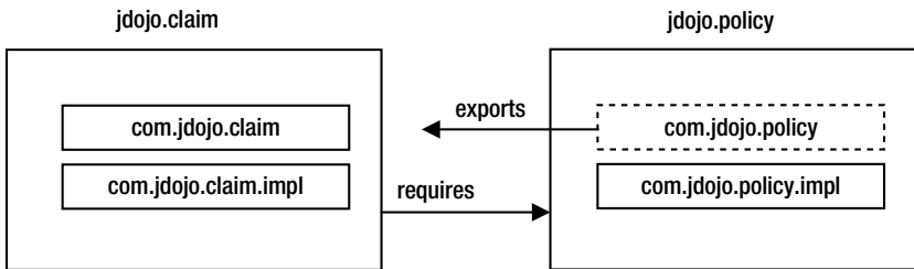
Figure 10-1. Declaring dependency between modules
