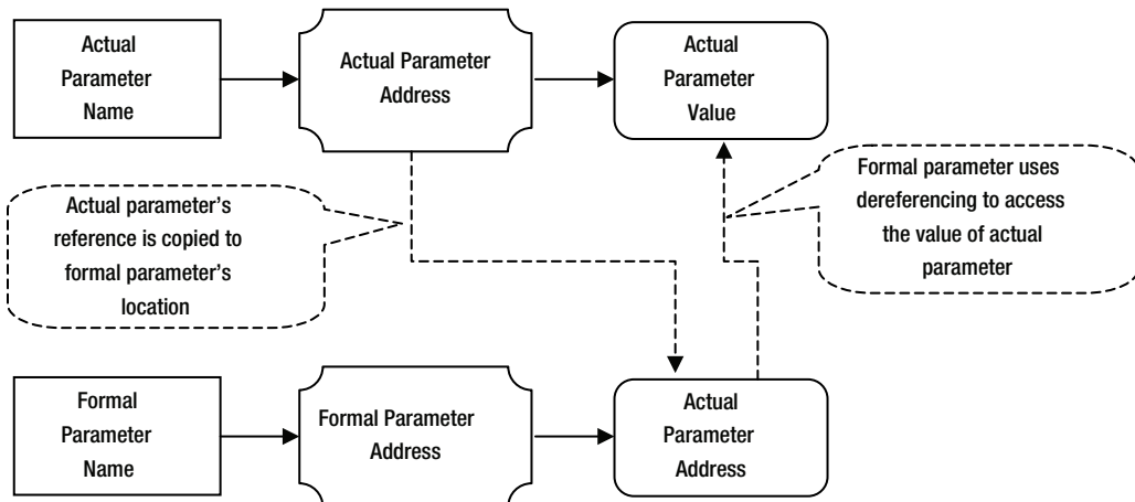
Figure 8-6. Memory states for actual and formal parameters when a method call is made using pass by reference value mechanism
