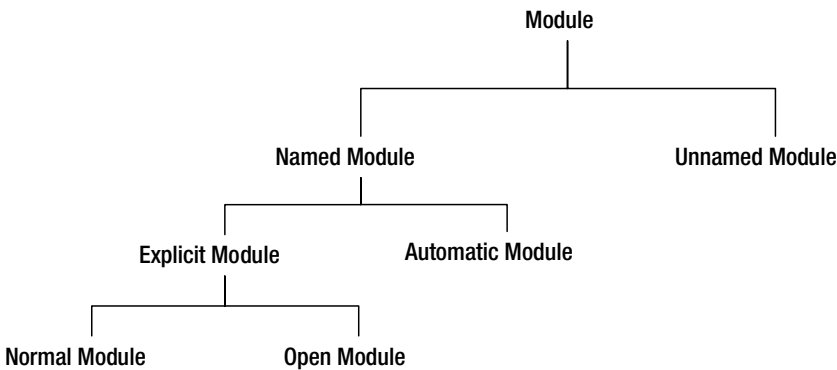
Figure 10-8. Types of modules
