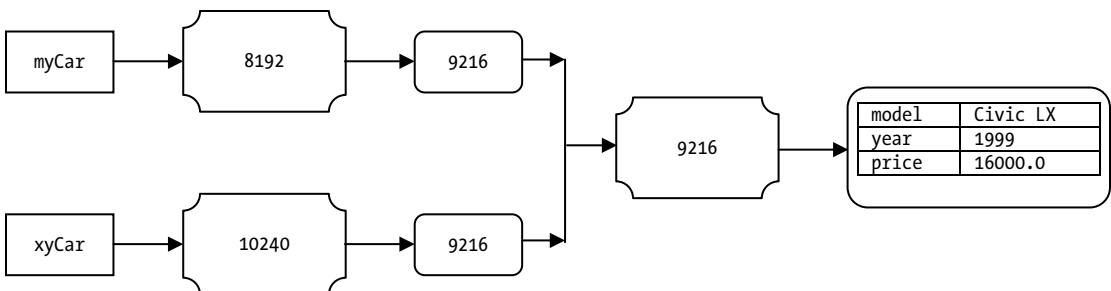
Figure 8-16. Memory state showing myCar and xyCar referencing the same Car object in memory after myCar and xyCar have been used to change the state of the Car object
