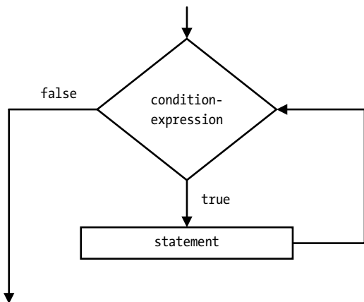
Figure 6-4. The flow diagram for a while statement
