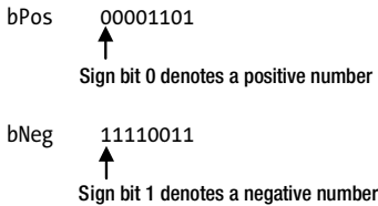
Figure 4-9. Storing the number 13 in 2's complement forms
