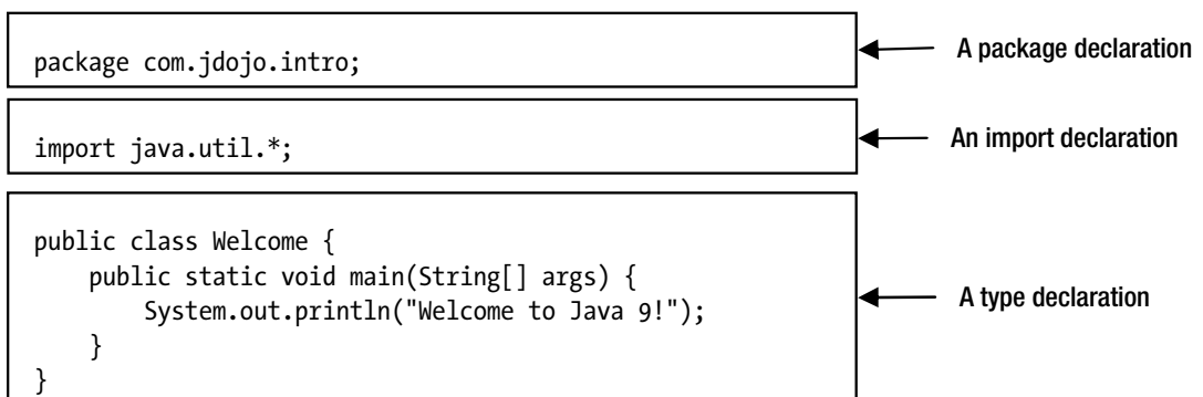
Figure 3-2. Parts of a compilation unit
