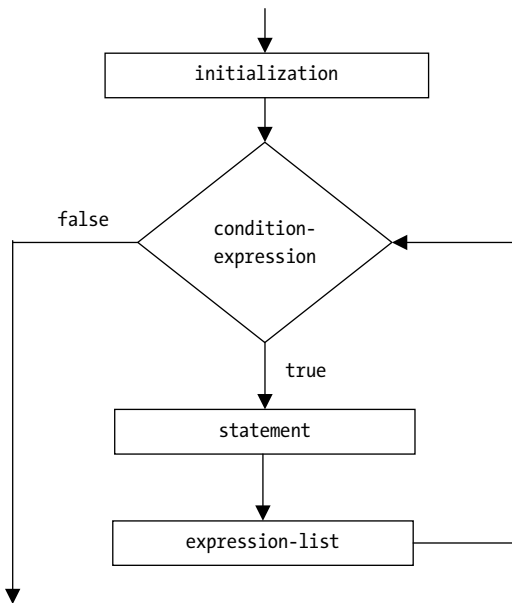
Figure 6-3. The flow diagram for a for-loop statement
