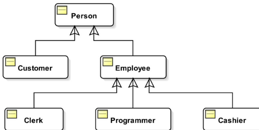
Figure 1-6. Inheritance hierarchy for the Person class
