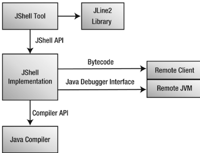
Figure 23-2. The JShell architecture
