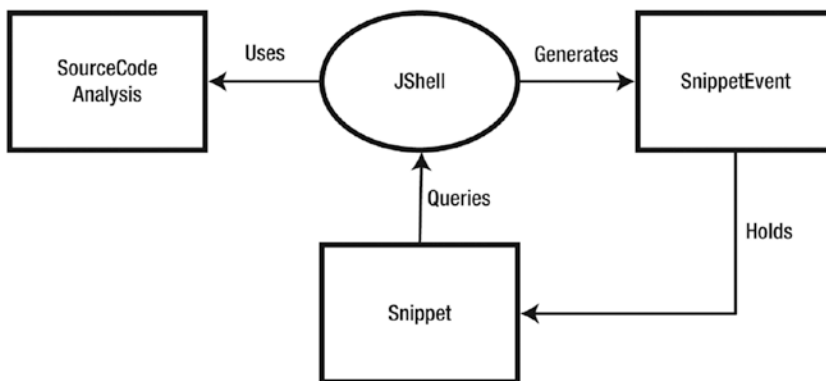
Figure 23-5. A use case diagram for the components of the JShell API
