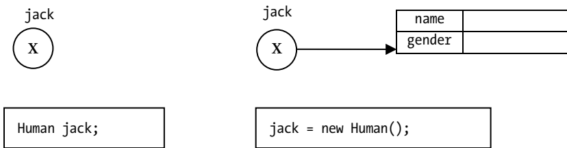
Figure 7-2. Memory states when a reference variable is declared and when a reference variable is assigned the reference of an instance of a class
