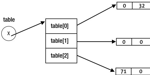
Figure 19-9. An array of arrays
