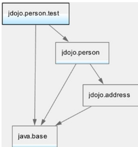
Figure 10-4. The module graph of the jdojo.person.test module
