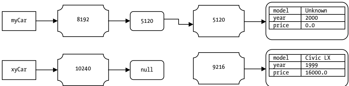
Figure 8-18. Memory state of reference variables myCar and xyCar and two Car objects after xyCar has been assigned a null reference
