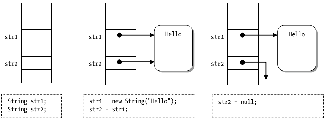
Figure 4-5. Memory states using null in the reference variables assignments
