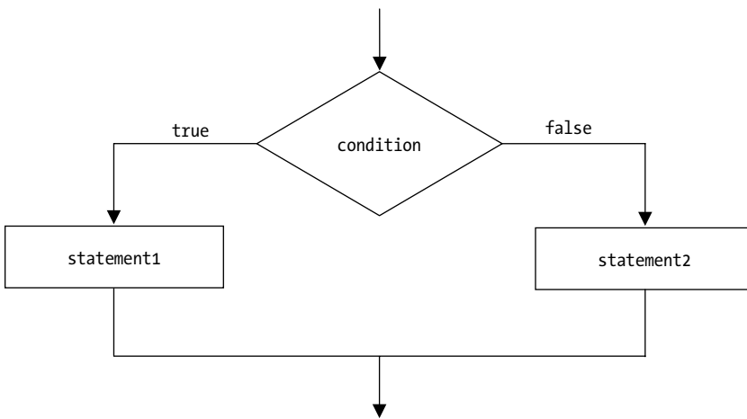
Figure 6-1. The flow diagram for an if-else statement
