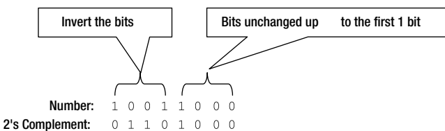
Figure 4-8. Computing 2's complement of a binary number
