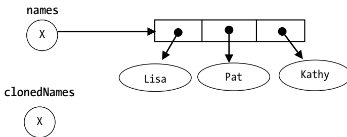
Figure 19-3. The ids array is cloned in the clonedIds array
