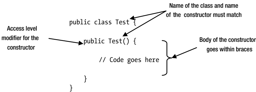
Figure 9-1. Anatomy of the constructor for the Test class
