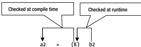
Figure 20-2. Runtime and compile-time checks made for downcasting
