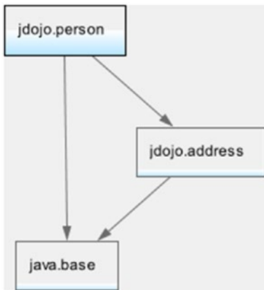
Figure 10-2. The module graph for the jdojo.person module
