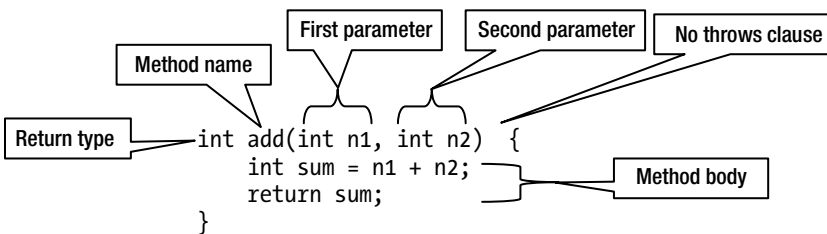
Figure 8-1. Parts of the add method
