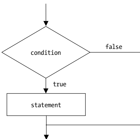
Figure 6-2. The flow diagram for an if statement
