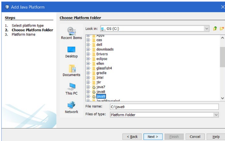
Figure 2-6. The Add Java Platform dialog box
