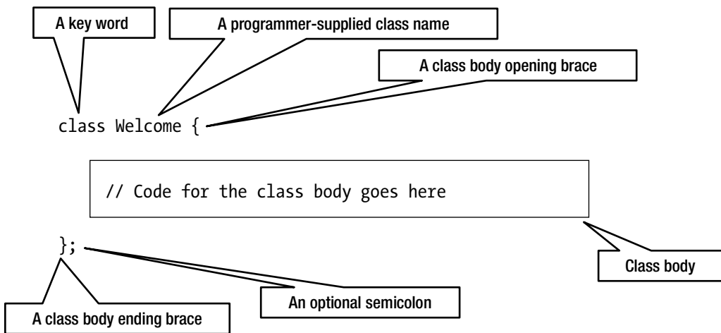
Figure 3-4. Parts of a class declaration in a compilation unit
