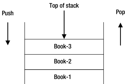
Figure 13-4. Memory arrangement in a stack
