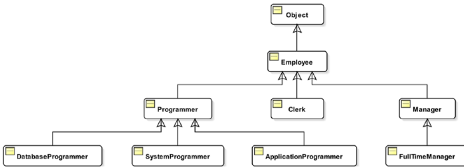
Figure 20-1. A sample inheritance class hierarchy
