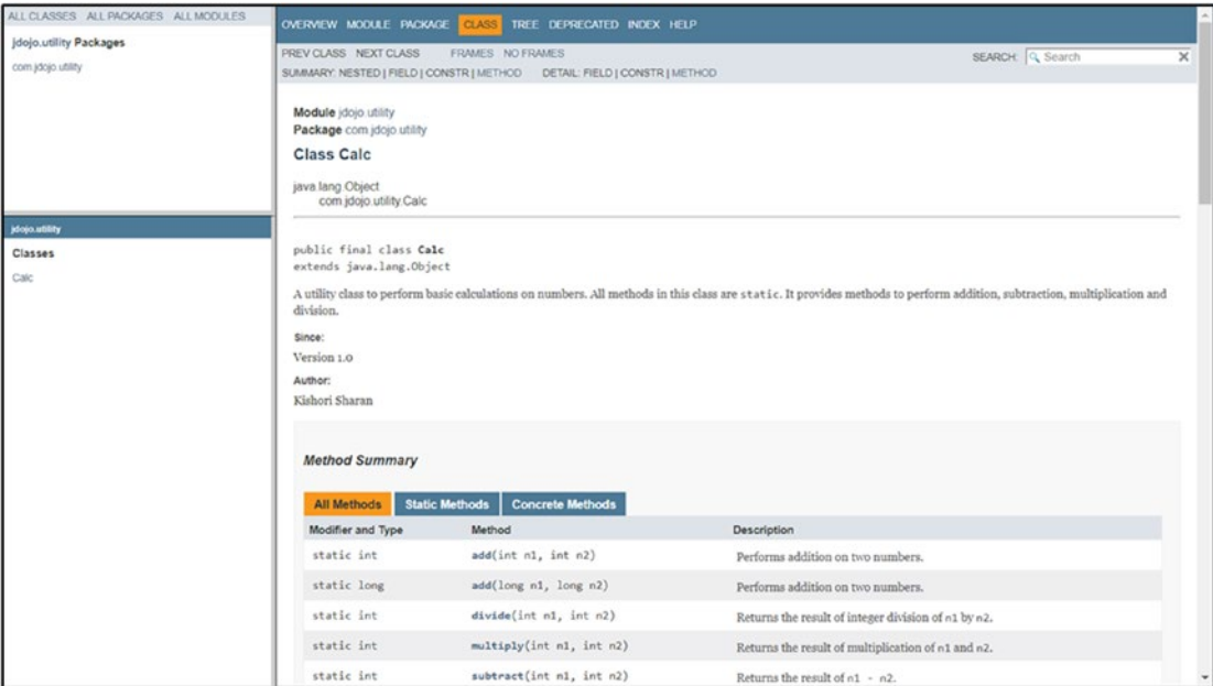
Figure B-2. The generated HTML page for the Calc class
