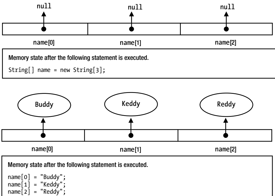
Figure 19-1. Reference type array initialization
