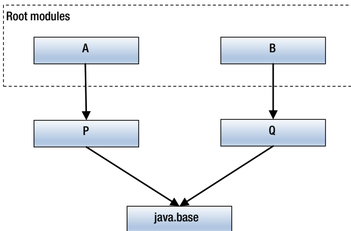
Figure 3-6. A module graph
