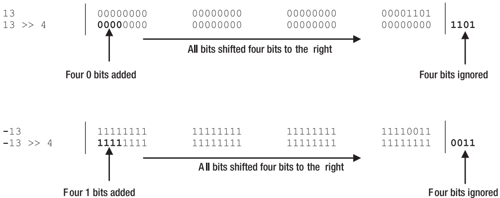
Figure 5-2. Computing 13 >> 4 and -13 >> 4
