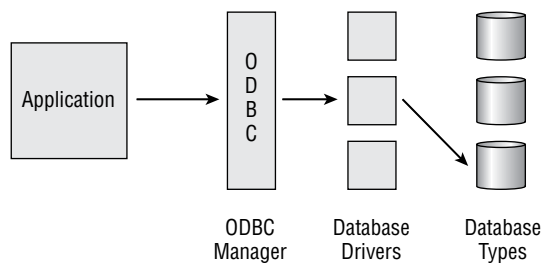
FIGURE 20.9 ODBC as the interface between applications and a backend database system
