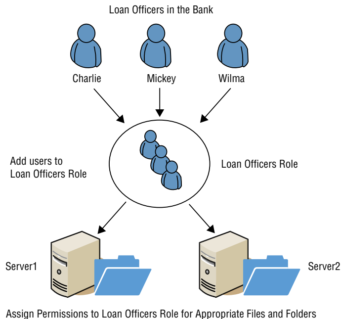
FIGURE 14.2 Role-based access controls
