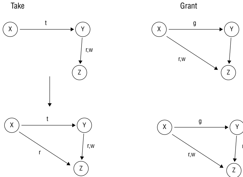
FIGURE 8.2 The Take Grant model's directed graph
