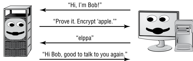
FIGURE 6.1 Challenge-response authentication protocol
