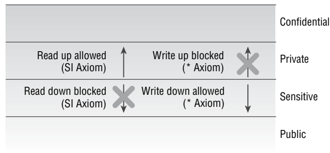
FIGURE 8.4 The Biba model
