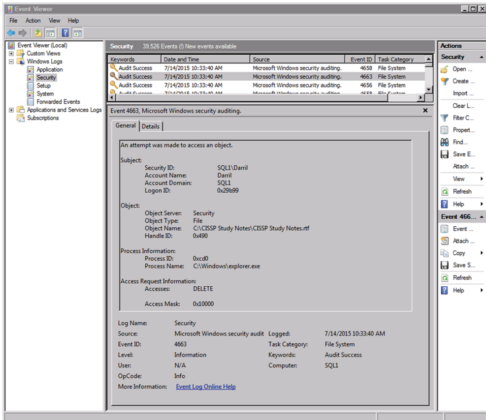
FIGURE 17.5 Viewing a log entry
