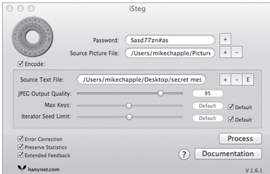
FIGURE 7.2 Steganography tool
