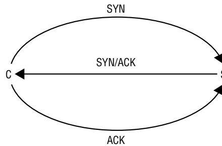
FIGURE 11.7 The TCP three-way handshake
