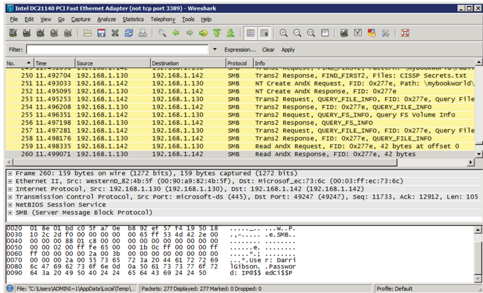
FIGURE 14.4 Wireshark capture
