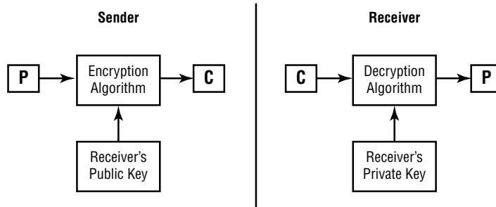
FIGURE 6.4 Asymmetric key cryptography
