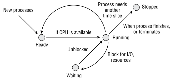
FIGURE 9.2 The process scheduler
