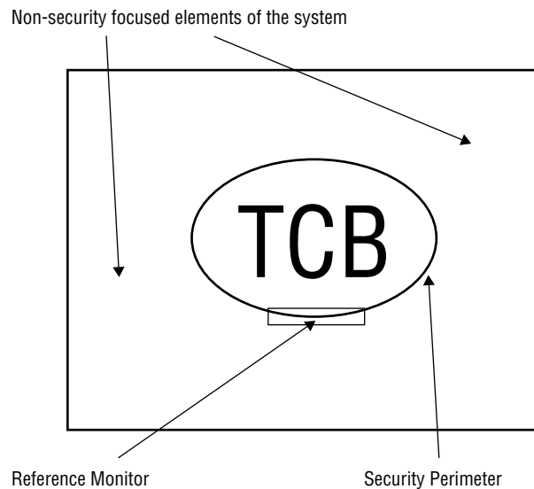
FIGURE 8.1 The TCB, security perimeter, and reference monitor
