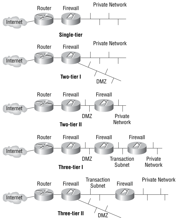
FIGURE 11.8 Single-, two-, and three-tier firewall deployment architectures
