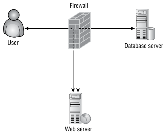
FIGURE 21.1 Typical database-driven website architecture
