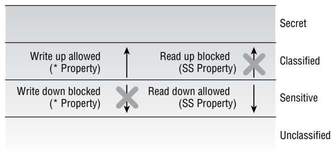
FIGURE 8.3 The Bell-LaPadula model
