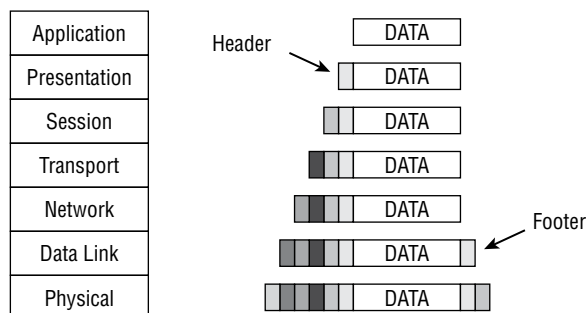
FIGURE 11.2 Representation of OSI model encapsulation
