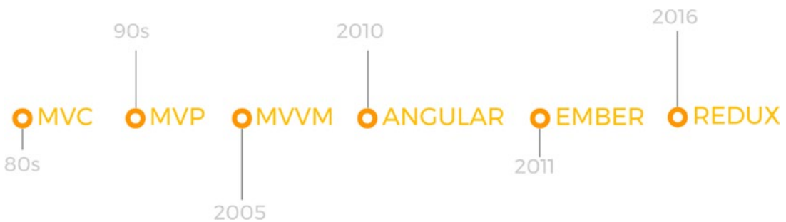
Figure 2-1. Architectures timeline
