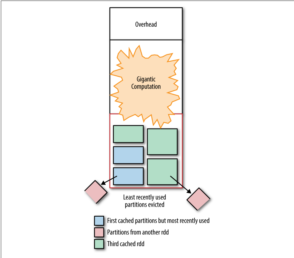
Figure A-3. A large computation may evict the cached partitions, if the storageFraction is full. The least recently used partitions are evicted first.
