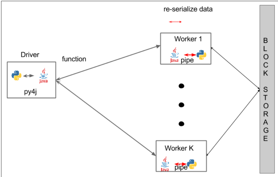
Figure 7-1. PySpark diagram
