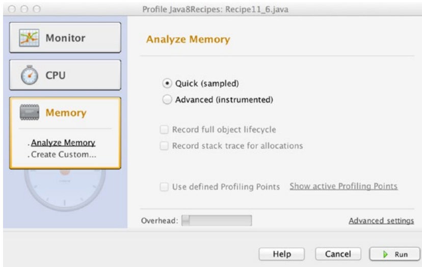
Figure 11-1. NetBeans Profiler
