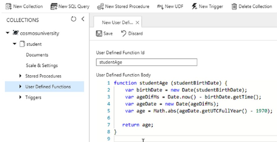
Figure 7-6. Creating the studentAge UDF
