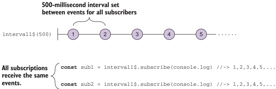
Figure 8.2 A cold observable is like an object factory, which can be used to create a family of subscriptions that will receive their own independent copy of all the events pushed through them.
