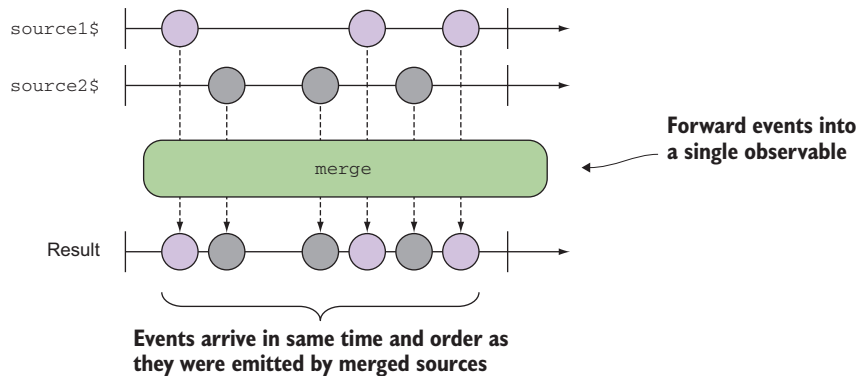
Figure 5.2 The merge() operator has no logic of its own, other than to combine events from multiple streams in the order in which they're emitted.
