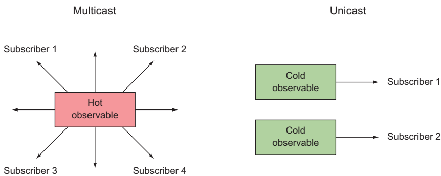
Figure 8.11 Multicast transmits messages from one source to many destinations; unicast sends dedicated messages to one destination address.
