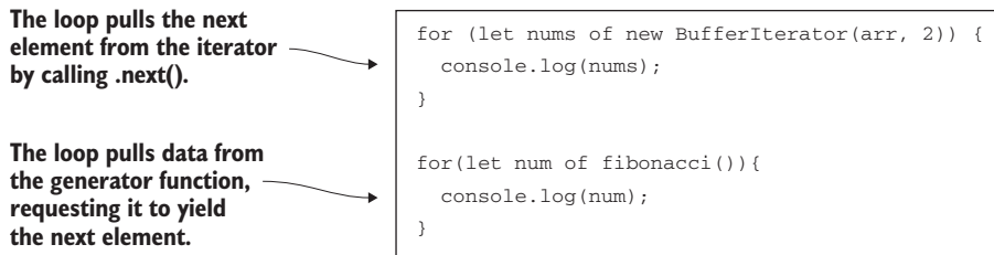
Figure 2.16 The pull mechanism of iterators
