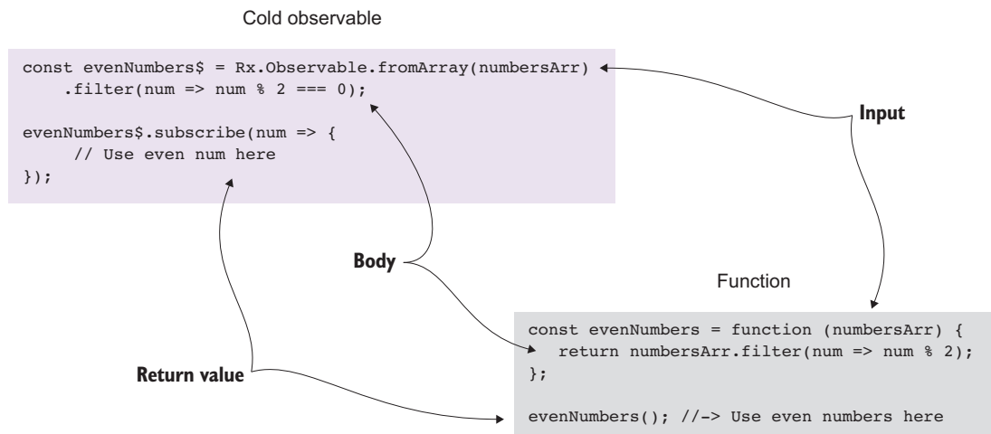
Figure 8.1 A cold observable can be thought of as a function that takes input—data that is to be processed—and, based on this, returns an output to the caller.
