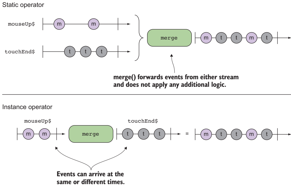
Figure 5.3 Static and instance versions of the merge operator between two streams. The results are the same. merge() is the simplest operator because it only forwards events from either stream as they come.
