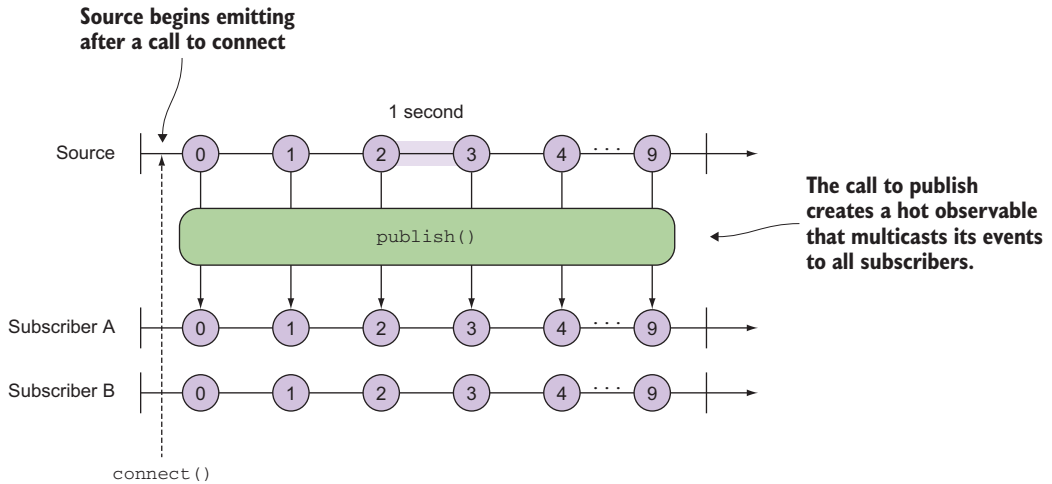
Figure 8.14 publish creates a hot observable whereby all subscribers begin receiving the events as soon as the call to connect is made. Otherwise, the source stream behaves like a cold observable, sitting idle until connect() is called. The share() operator would yield the same results except that the call to connect() would be done internally by the library.
