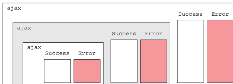
Figure 7.1 Imperative asynchronous error handling tends to nest when processing a series of asynchronous calls.
