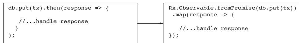
Figure 6.8 Adapting the callback-based API into an observable
