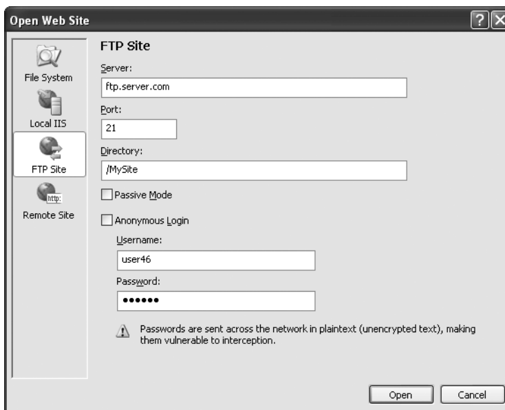
Figure 12-22. Setting the target site
