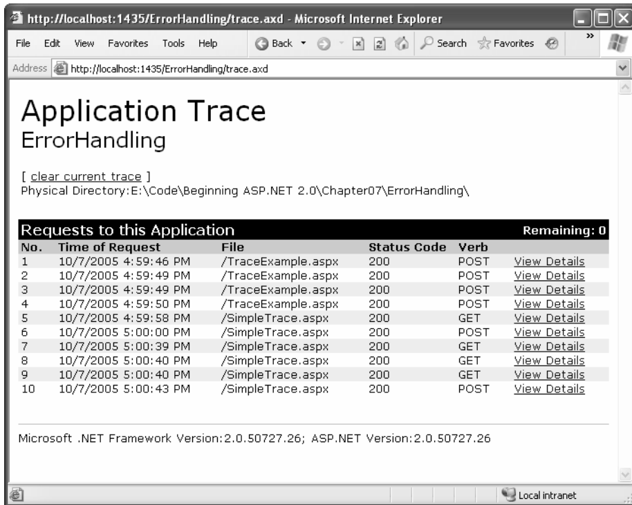
Figure 7-28. Traced application request
