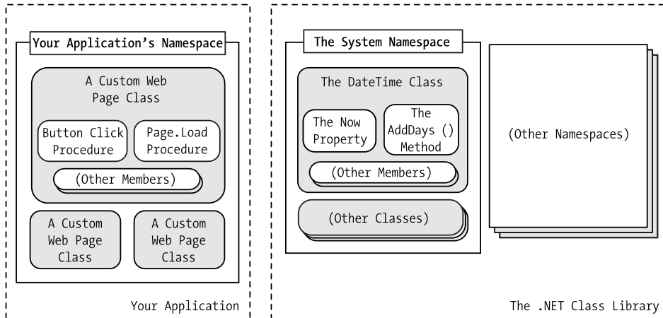
Figure 3-3. A look at two namespaces
