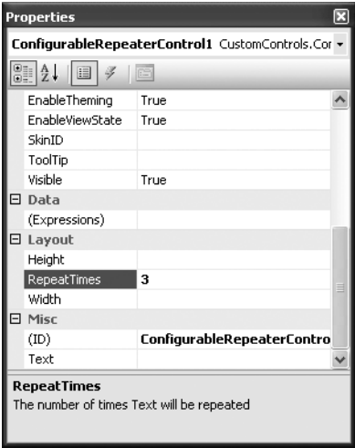
Figure 25-16. Custom control design-time support
