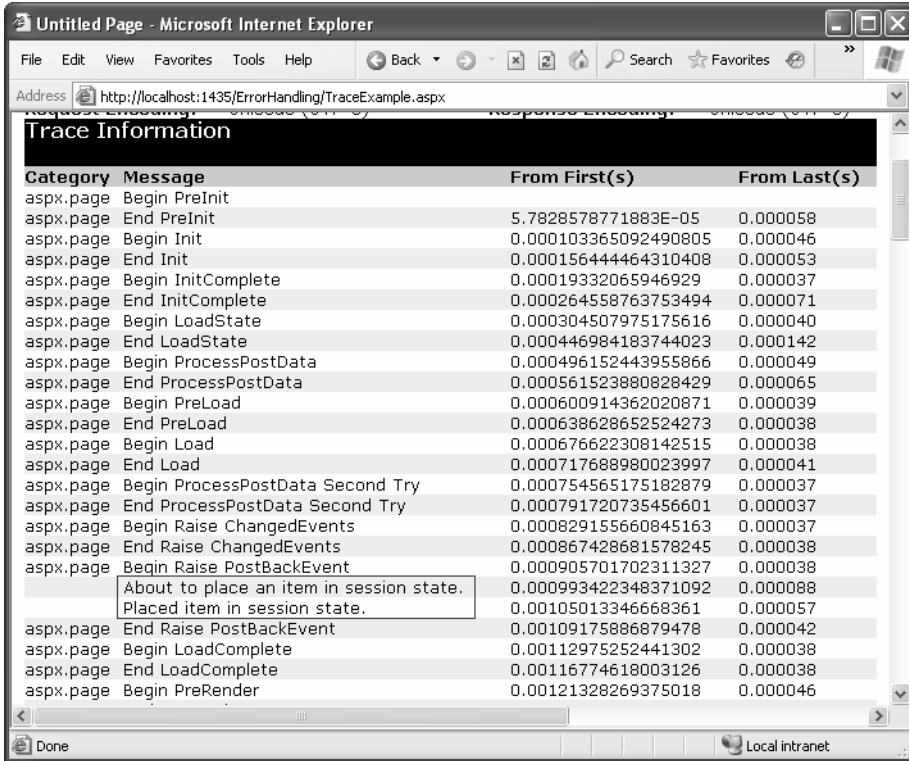
Figure 7-25. Custom trace messages
