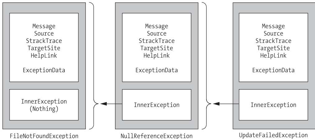
Figure 7-3. Exceptions can be chained together.
