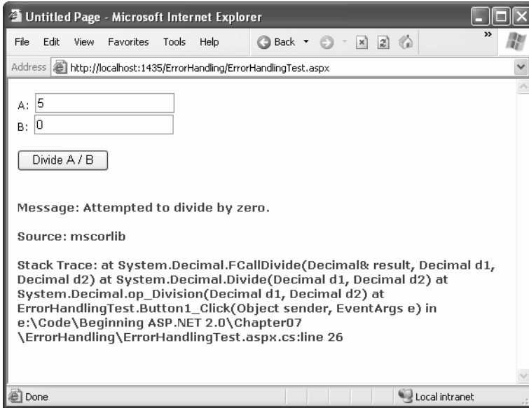
Figure 7-4. Catching and displaying exception information
