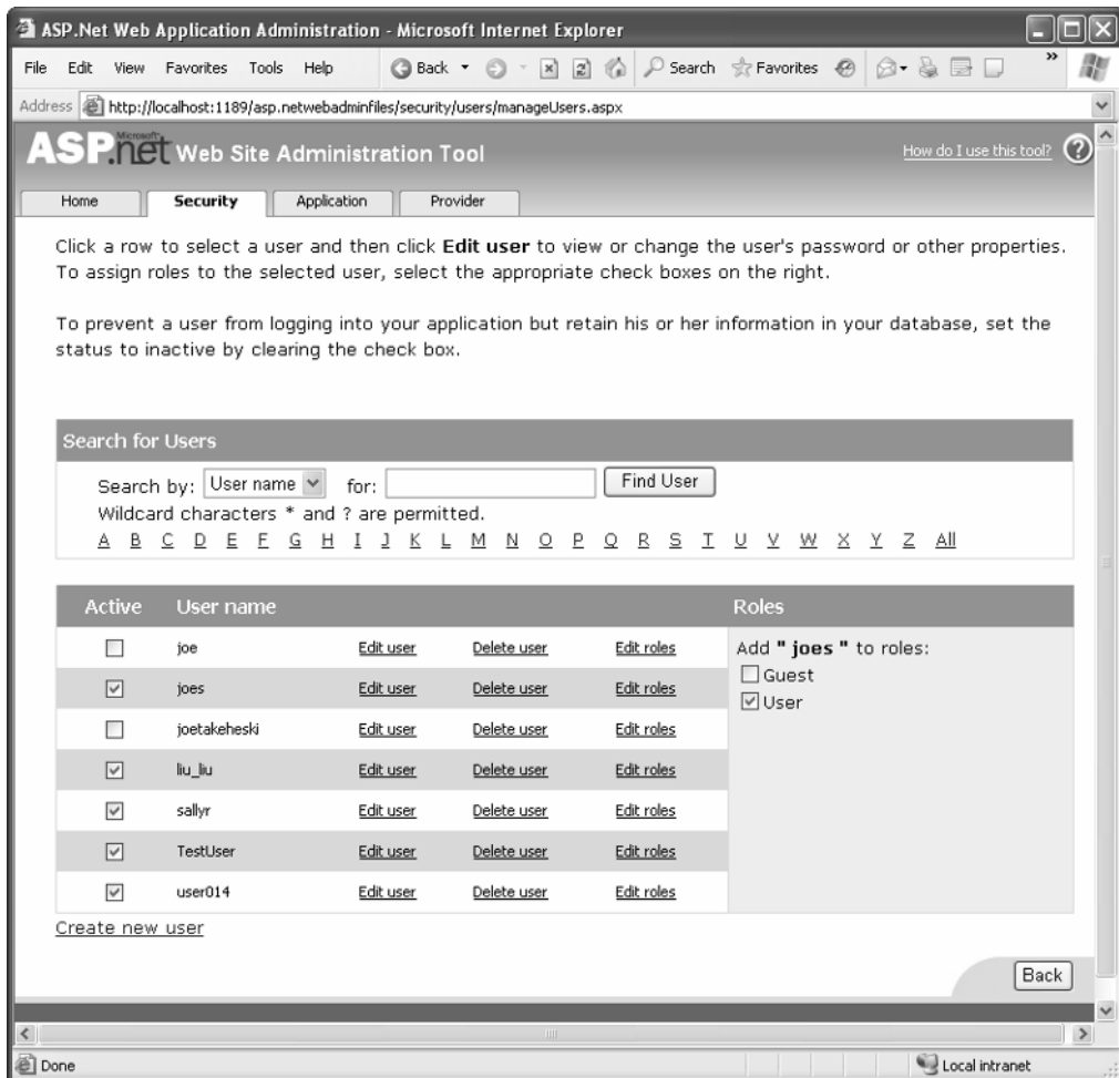
Figure 19-14. Applying roles
