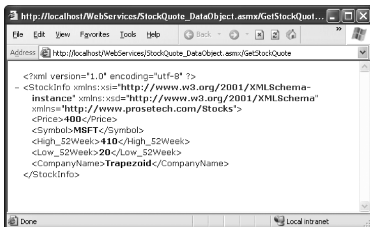
Figure 22-7. The result from GetStockQuote() as a data object
