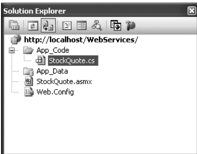
Figure 22-2. A web service with a code-behind file
