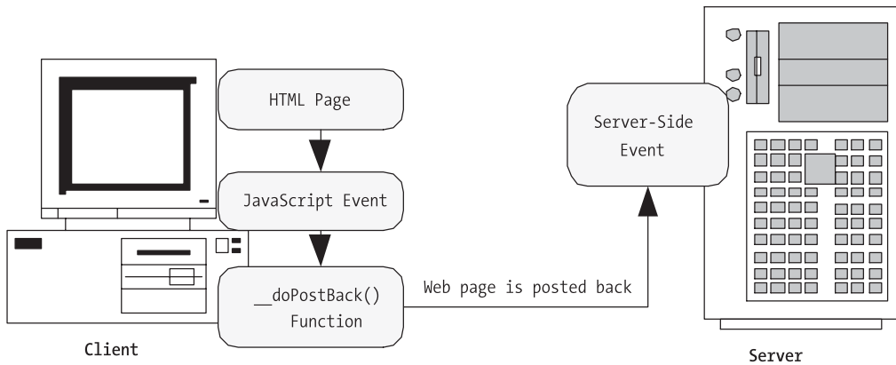
Figure 6-13. An automatic postback
