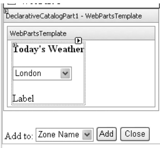
Figure 27-14. A DeclarativeCatalogPart
