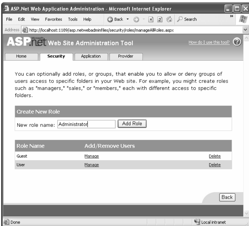
Figure 19-13. Creating roles
