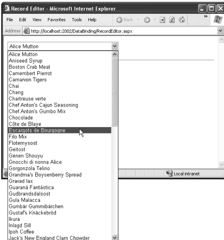
Figure 14-9. Product choices
