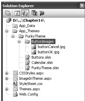
Figure 10-15. Adding images to a theme
