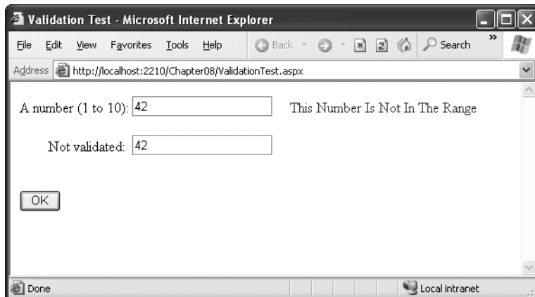
Figure 8-1. Failed validation
