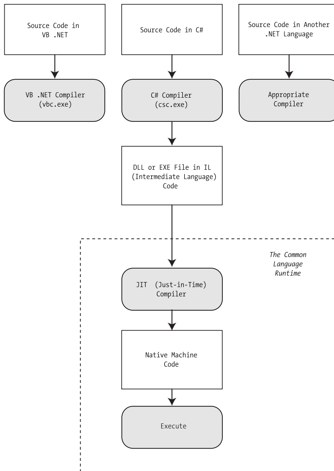
Figure 1-5. Language compilation in .NET
