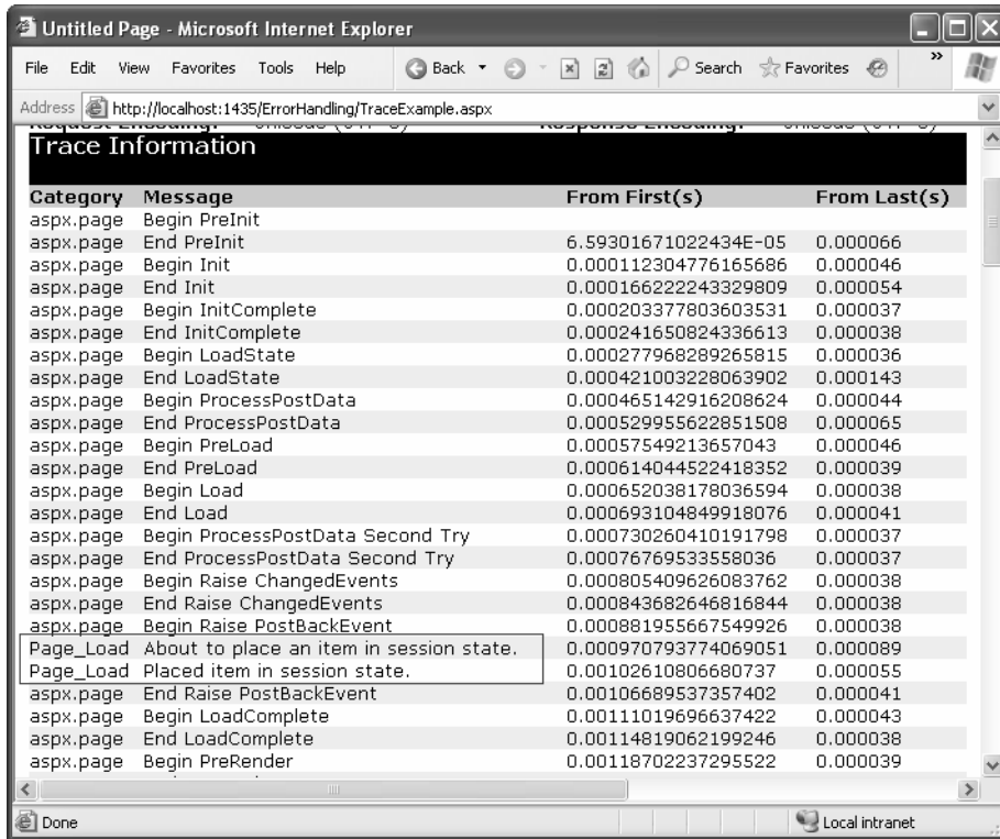
Figure 7-26. A categorized trace message
