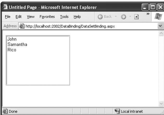
Figure 14-8. DataSet binding
