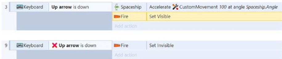
Figure 3-12. Events for setting the visibility of the Fire object
