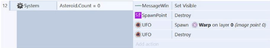
Figure 3-25. Modified “you win” event
