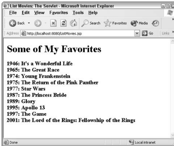
Figure 3-4: The ListMovies JSP in action.
