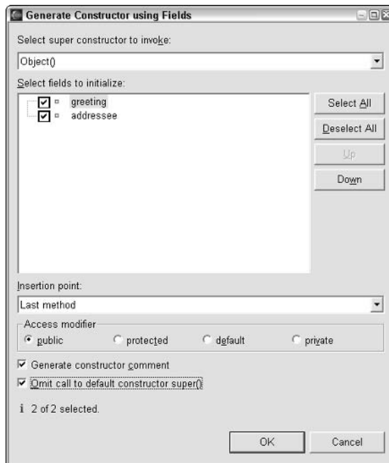
Figure 4-9: Eclipse can auto- matically create constructors for you.
