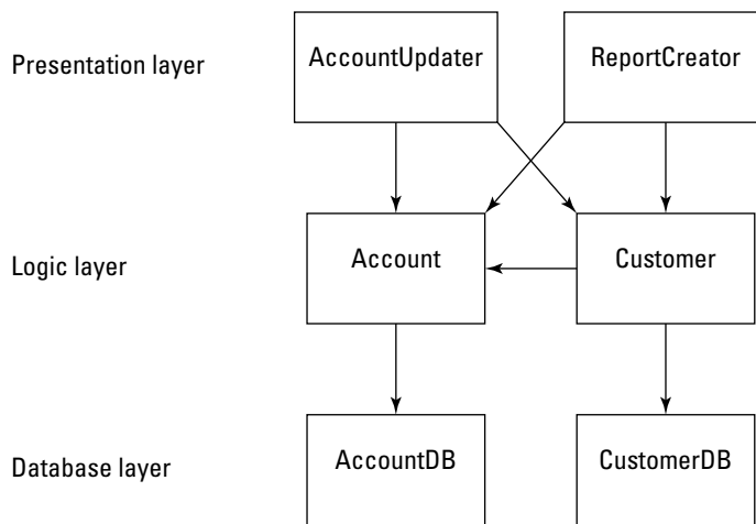
Figure 1-1: Three- layered design.
