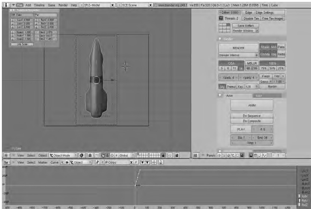
Figure 7-1. Blender
