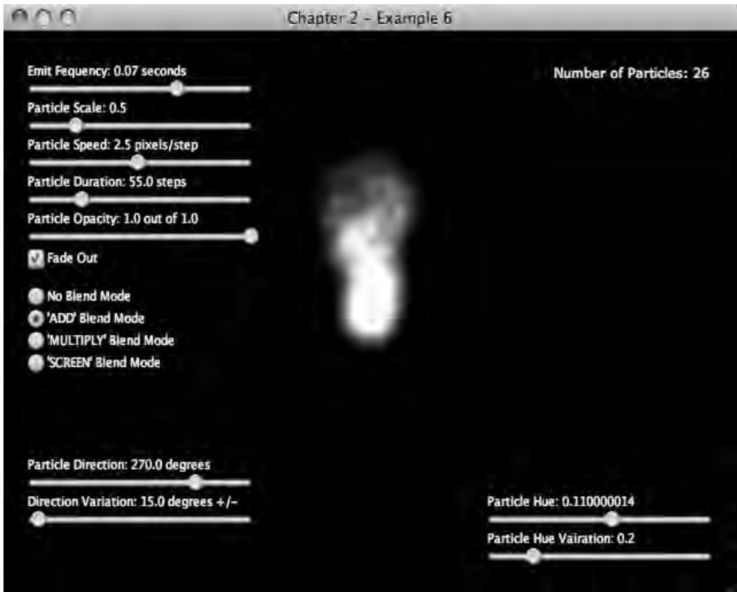
Figure 2-9. Example 6, fire
