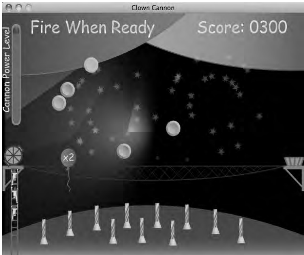
Figure 11-7. Fireworks
