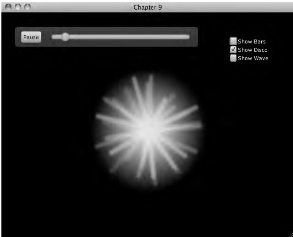
Figure 9-4. Disco effect
