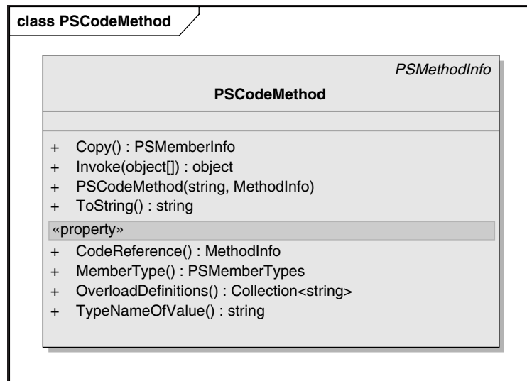
Figure 3-17: PSCodeMethod
