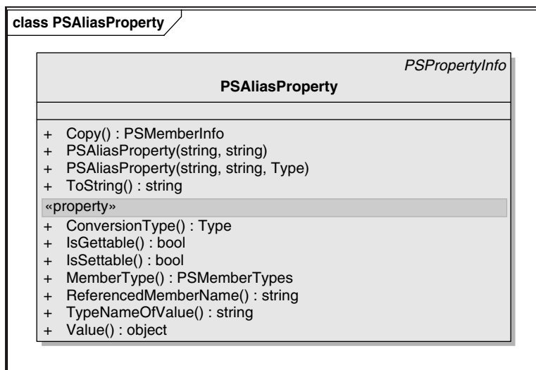
Figure 3-13: AliasProperty
