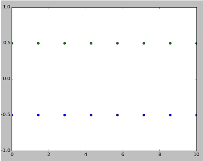
Figure 10-9. linspace() graph
