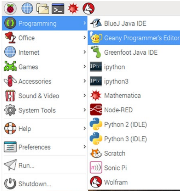
Figure 3-3. Raspbian Menu
