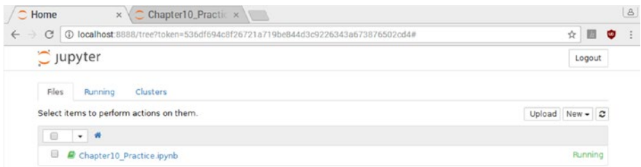
Figure 10-6. Notebook running
