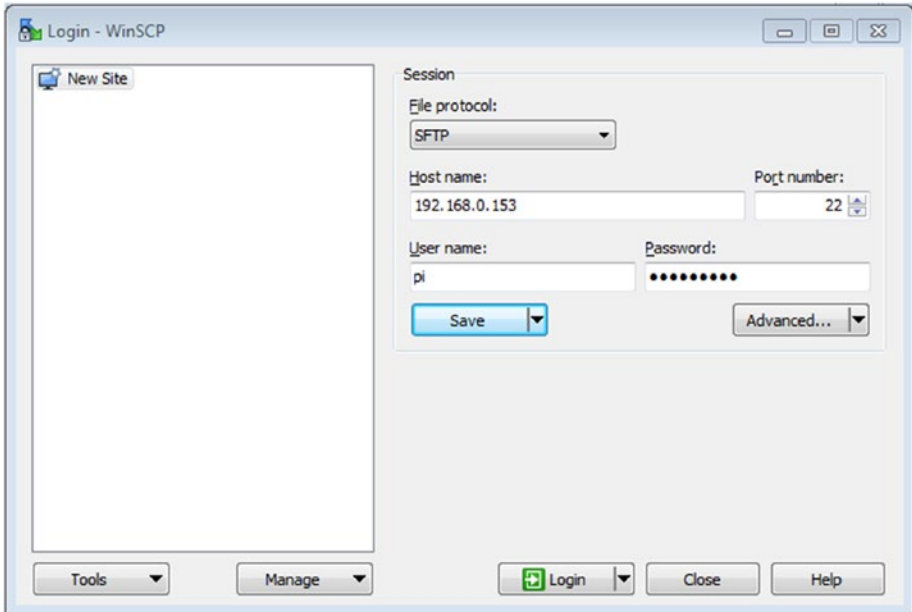
Figure 2-10. WinSCP window
