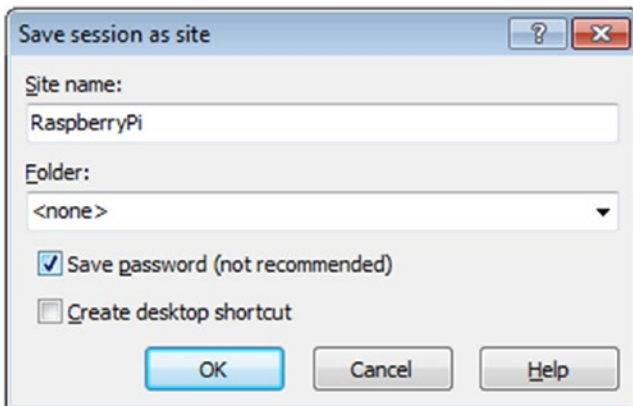
Figure 2-11. Save session
