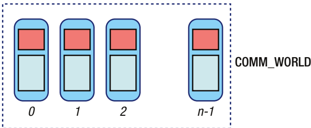
Figure 8-2. COMM_WORLD
