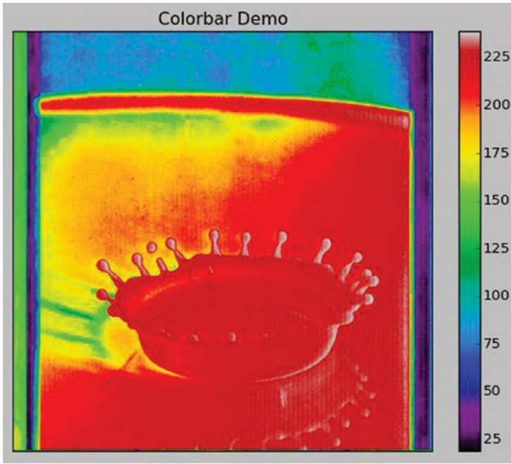
Figure 14-3. Colorbar demo
