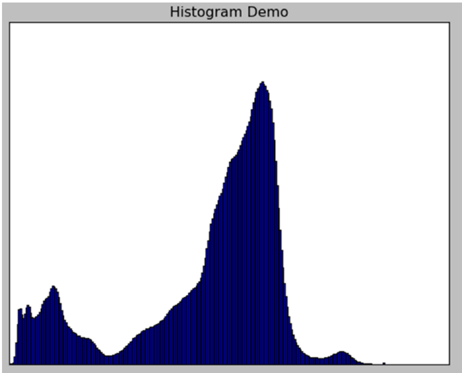
Figure 14-4. Histogram demo
