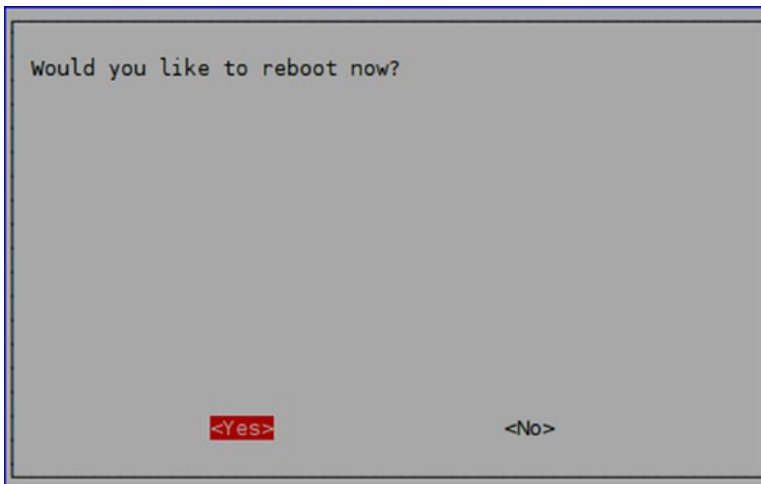
Figure 1-21. Reboot Prompt
