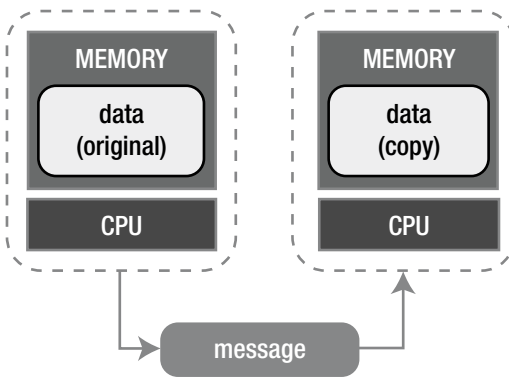
Figure 8-3. One-to-one communication
