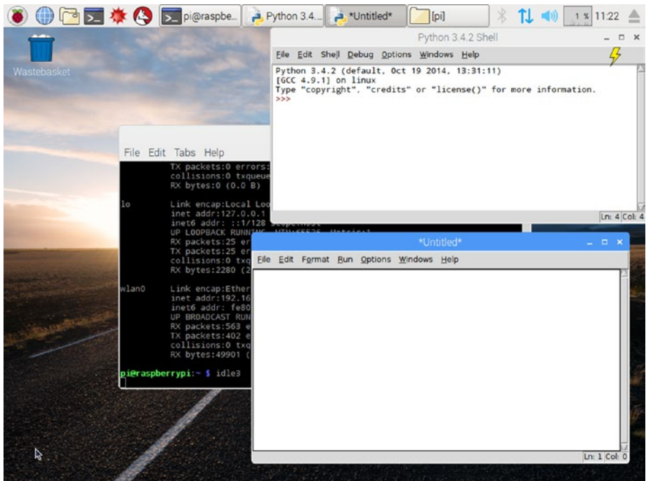
Figure 3-1. IDLE3
