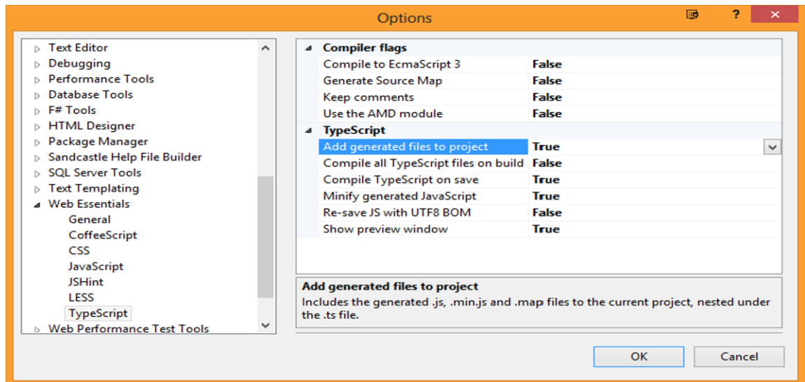
Figure 3-1. The Web Essentials Options dialog box for TypeScript
