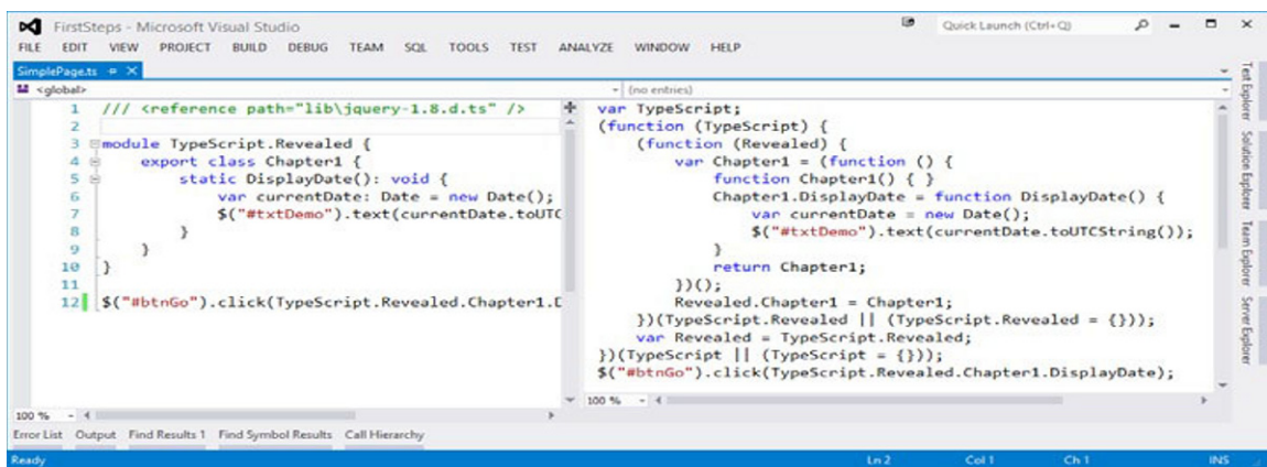
Figure 2-1. The TLS displays the JavaScript your TypeScript will be compiled into
