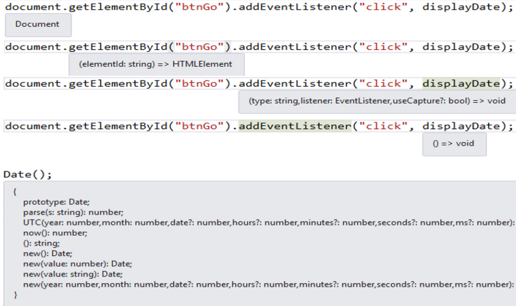
Figure 1-7. The TypeScript Language Service displays type and method information as you hover
