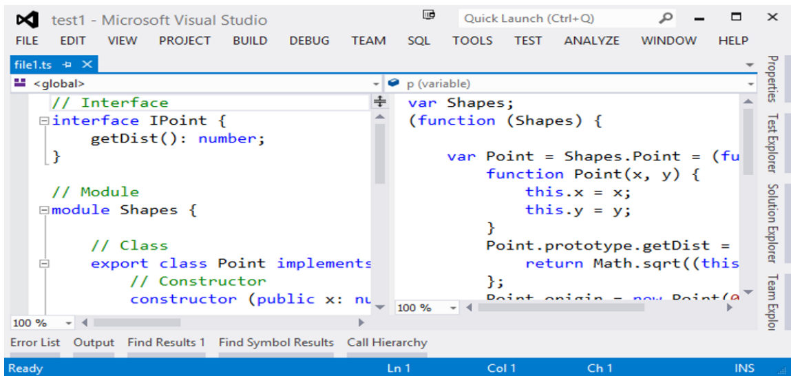
Figure 1-5. The split-pane view of a TypeScript file in Visual Studio 2012 with the Web Essentials extension installed
