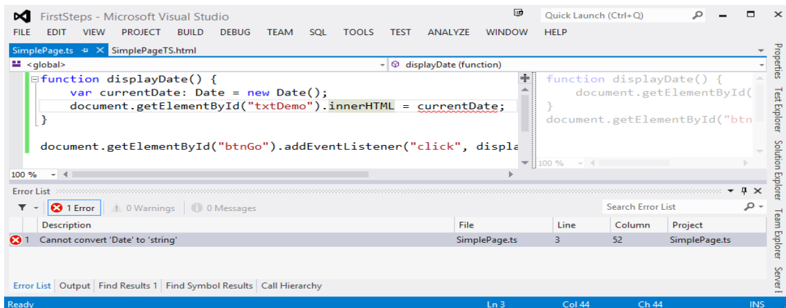
Figure 1-8. TypeScript errors are underscored in the edit window and listed in the Error List window
