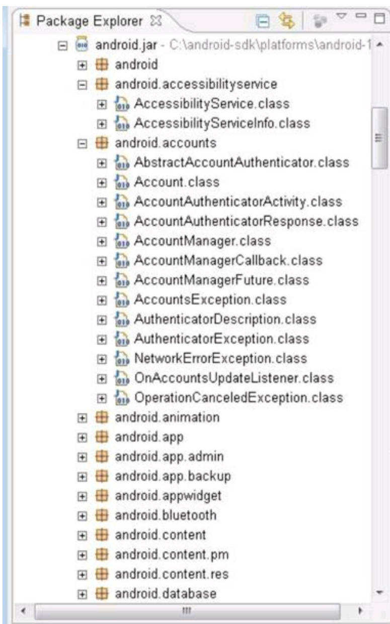
Figure 3-18: The android.jar file includes general-purpose Java packages.
