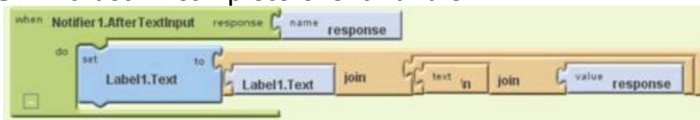
Figure 1-34: At last! A complete event handler!
