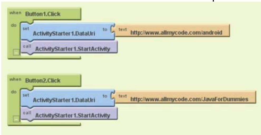
Figure 2-22: The Blocks viewer for this section's example.
