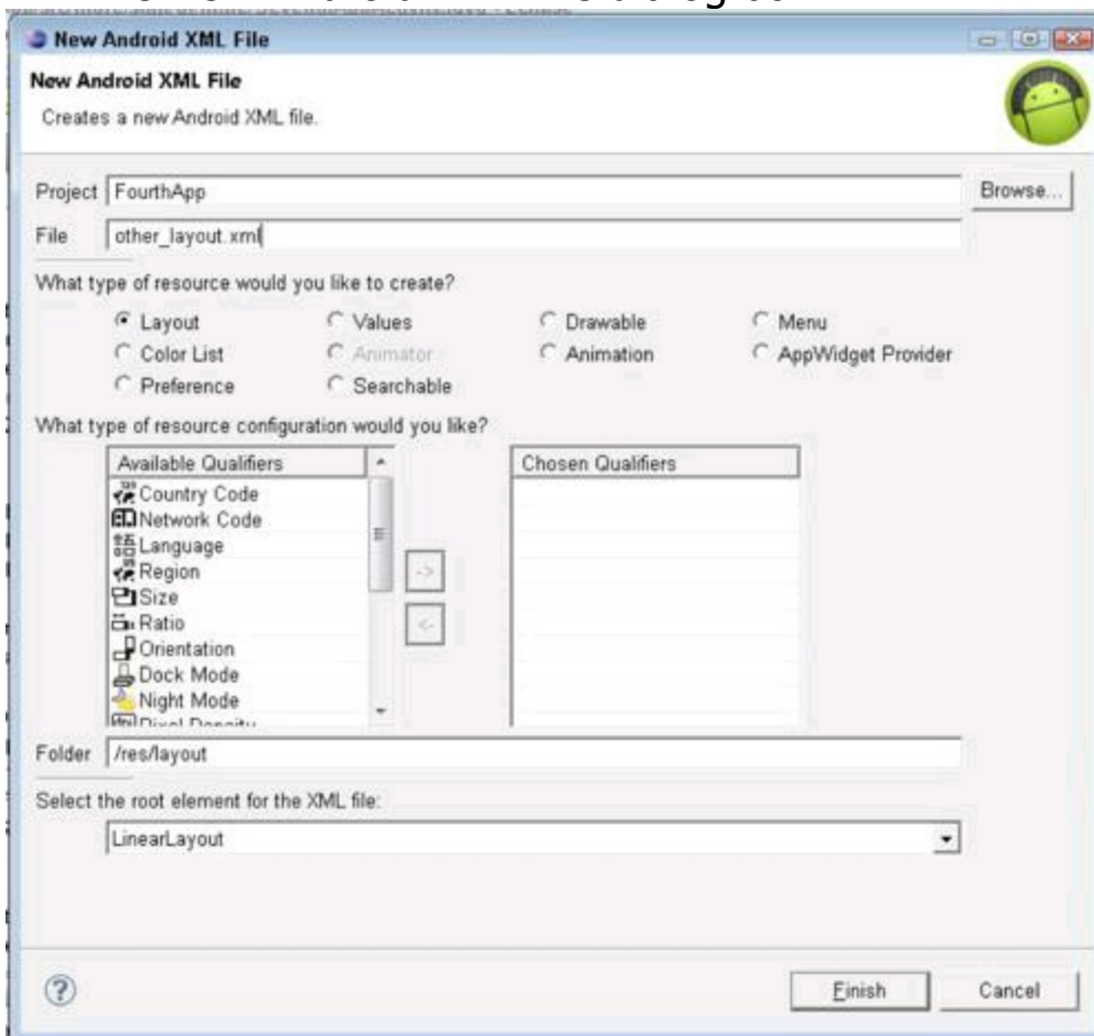
Figure 4-11: The New Android XML File dialog box.
