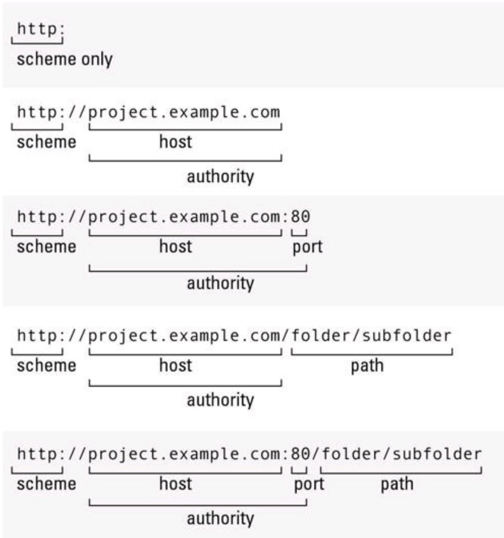
Figure 2-3: Uniform Resource Identifiers.
