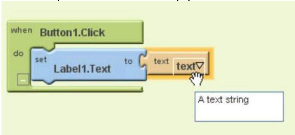
Figure 1-26: A clump of blocks with no empty socket.
