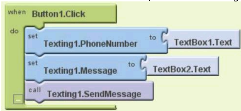
Figure 2-5: When the user clicks the button, send a text message.
