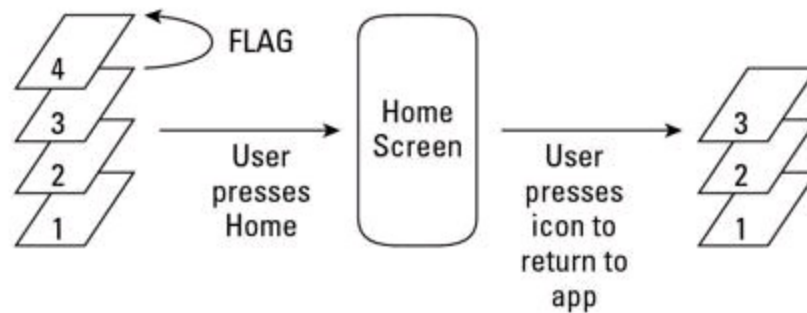
Figure 2-15: The effect of adding FLAG_ACTIVITY_SINGLE_TOP .
