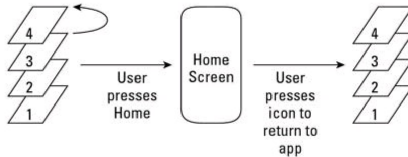
Figure 2-14: The effect of adding FLAG_ACTIVITY_NO_HISTORY . Without FLAG_ACTIVITY_NO_HISTORY :
