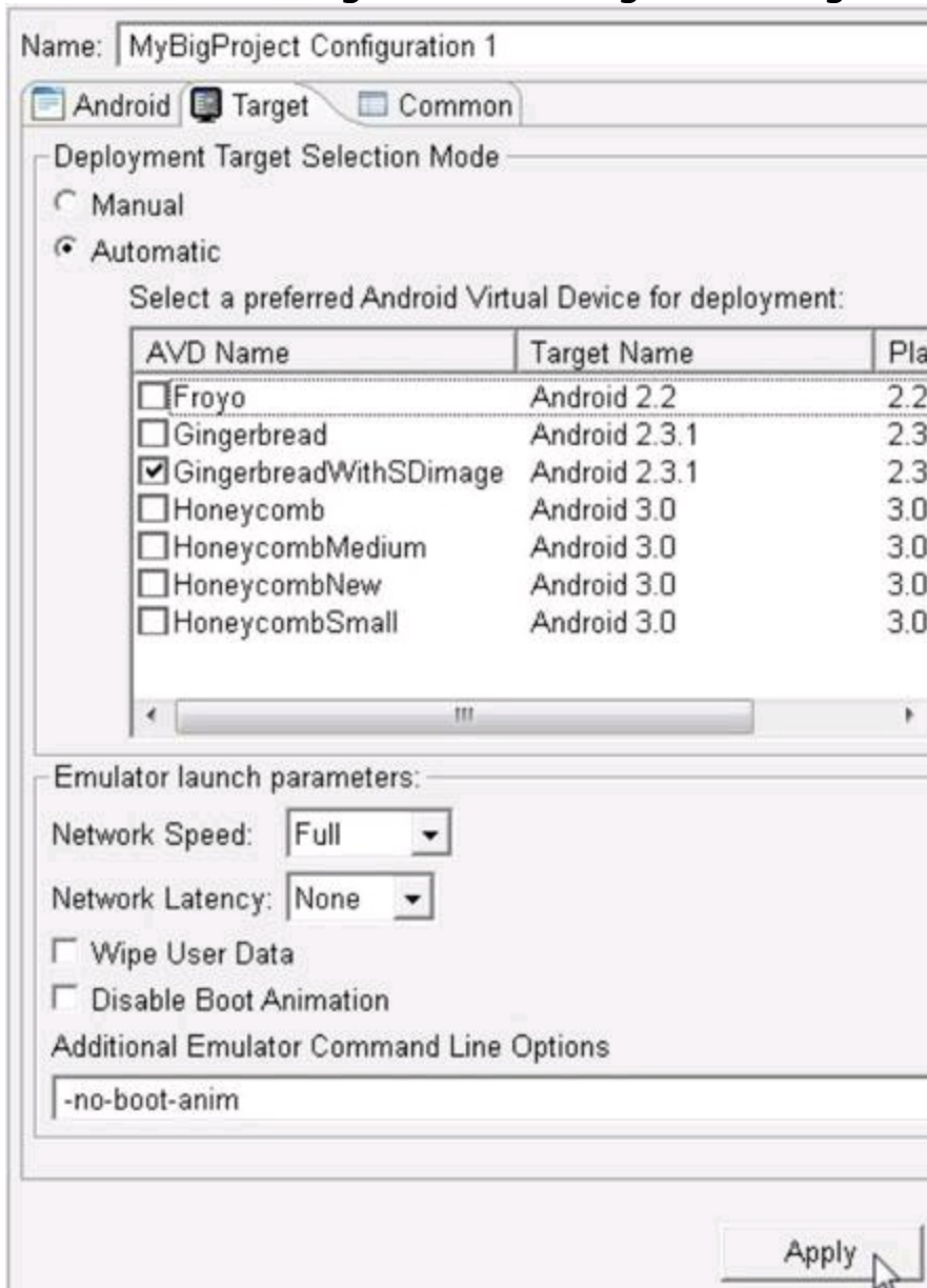
Figure 1-29: The Run Configurations dialog box's Target tab.
