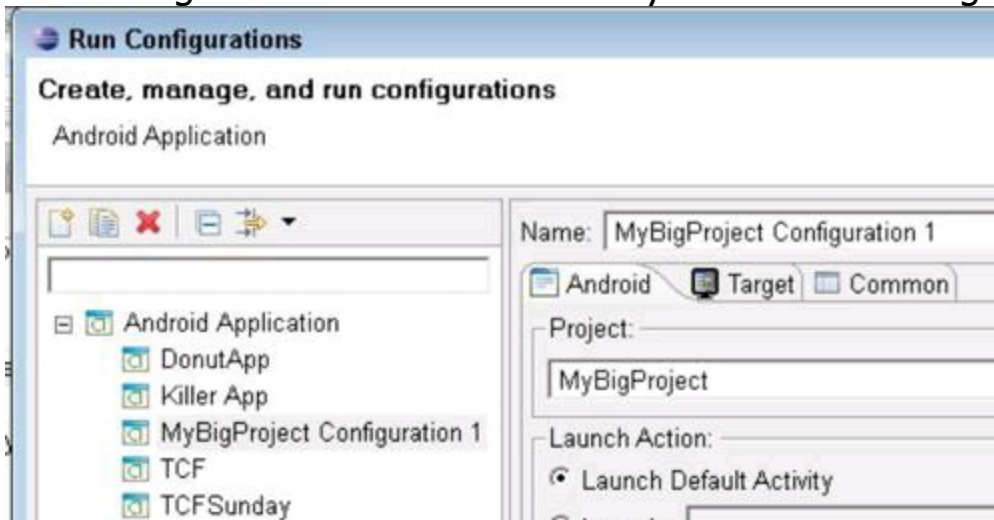
Figure 1-28: Adding some information about your custom configuration.
