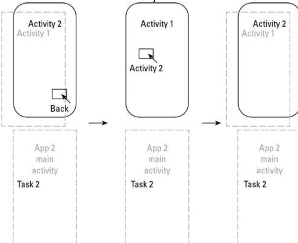
Figure 1-4: The user dismisses Activity 2 and then invokes Activity 2.
