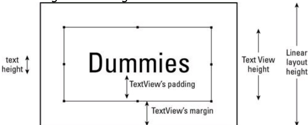
Figure 1-6: Padding versus margin.
