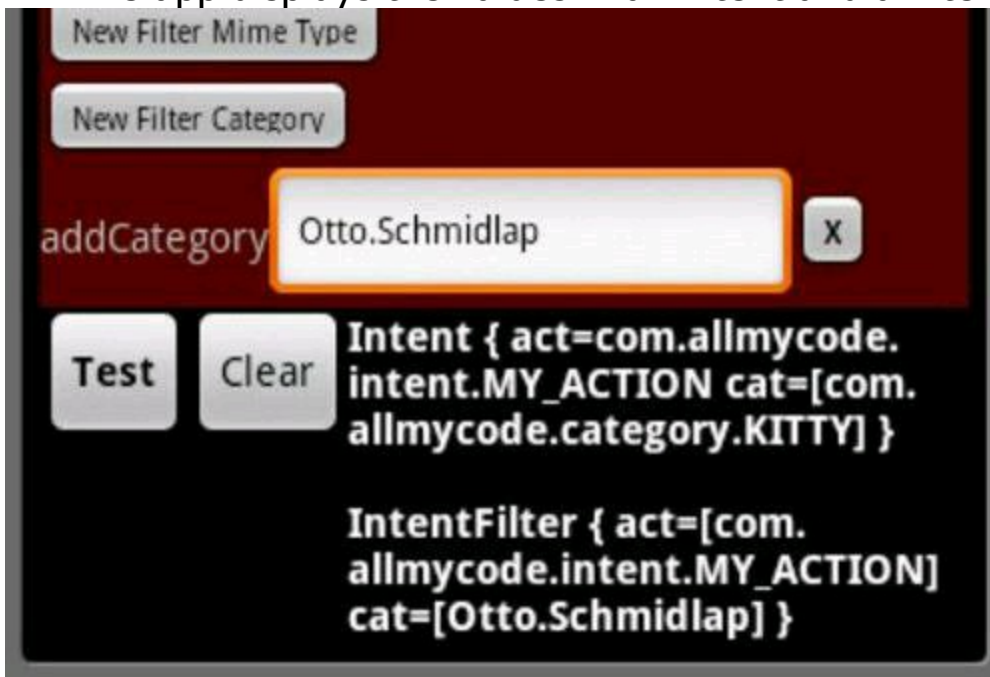
Figure 2-11: The app displays the values in an intent and a filter.
