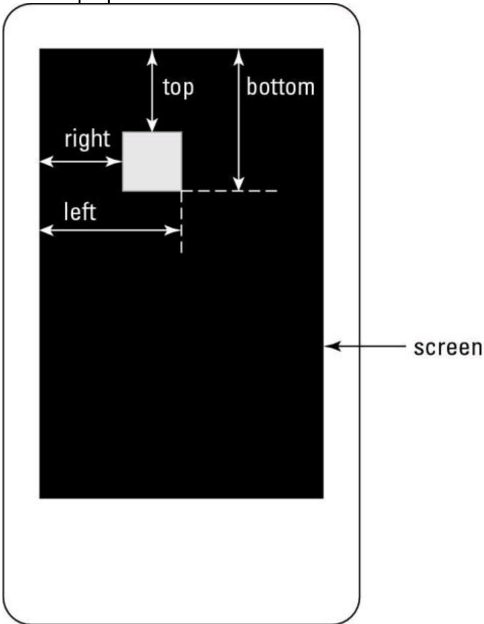
Figure 3-11: The properties of a Rect instance.
