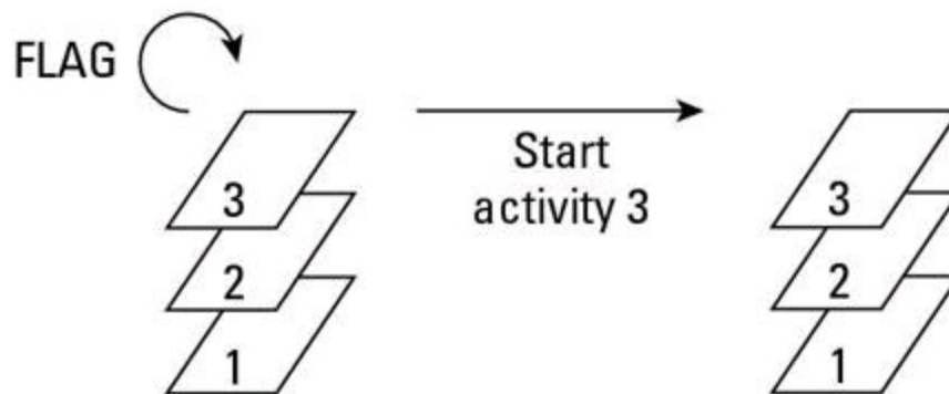
Figure 2-16: The effect of adding FLAG_ACTIVITY_CLEAR_TOP .
