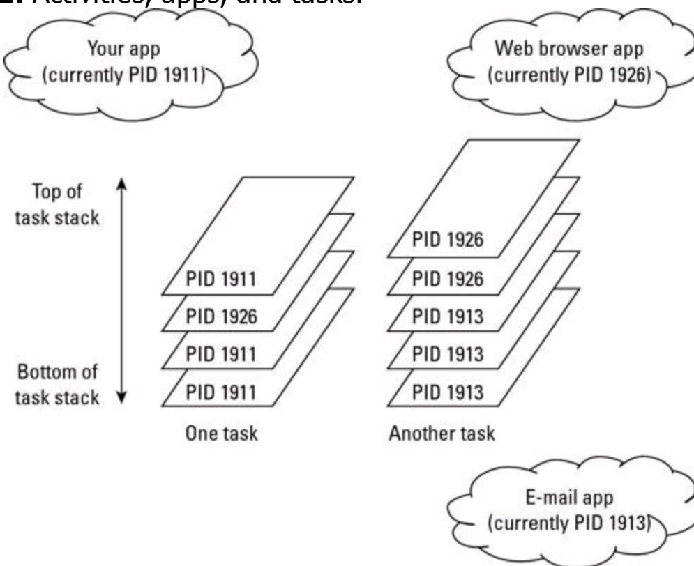
Figure 1-1: Activities, apps, and tasks.
