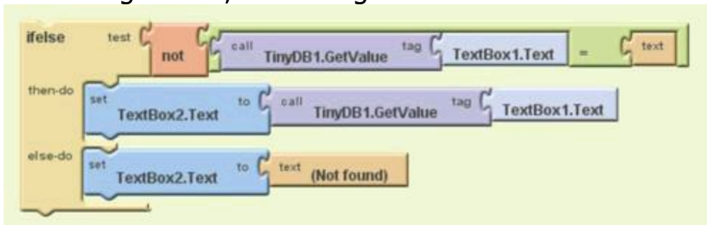
Figure 2-18: Store Barry's info and Harriet's info.
