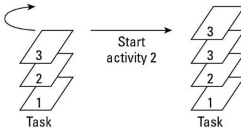
Figure 2-19: The effect of adding FLAG_ACTIVITY_REORDER_TO_FRONT. Without FLAG_ACTIVITY_REORDER_TO_FRONT:
