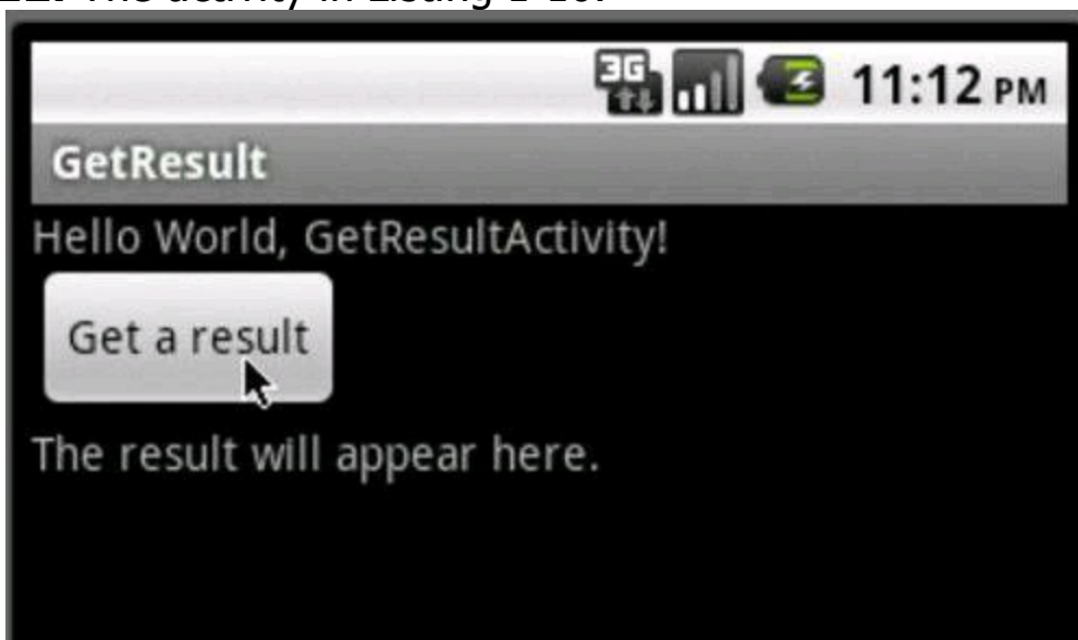
Figure 1-12: The activity in Listing 1-10.
