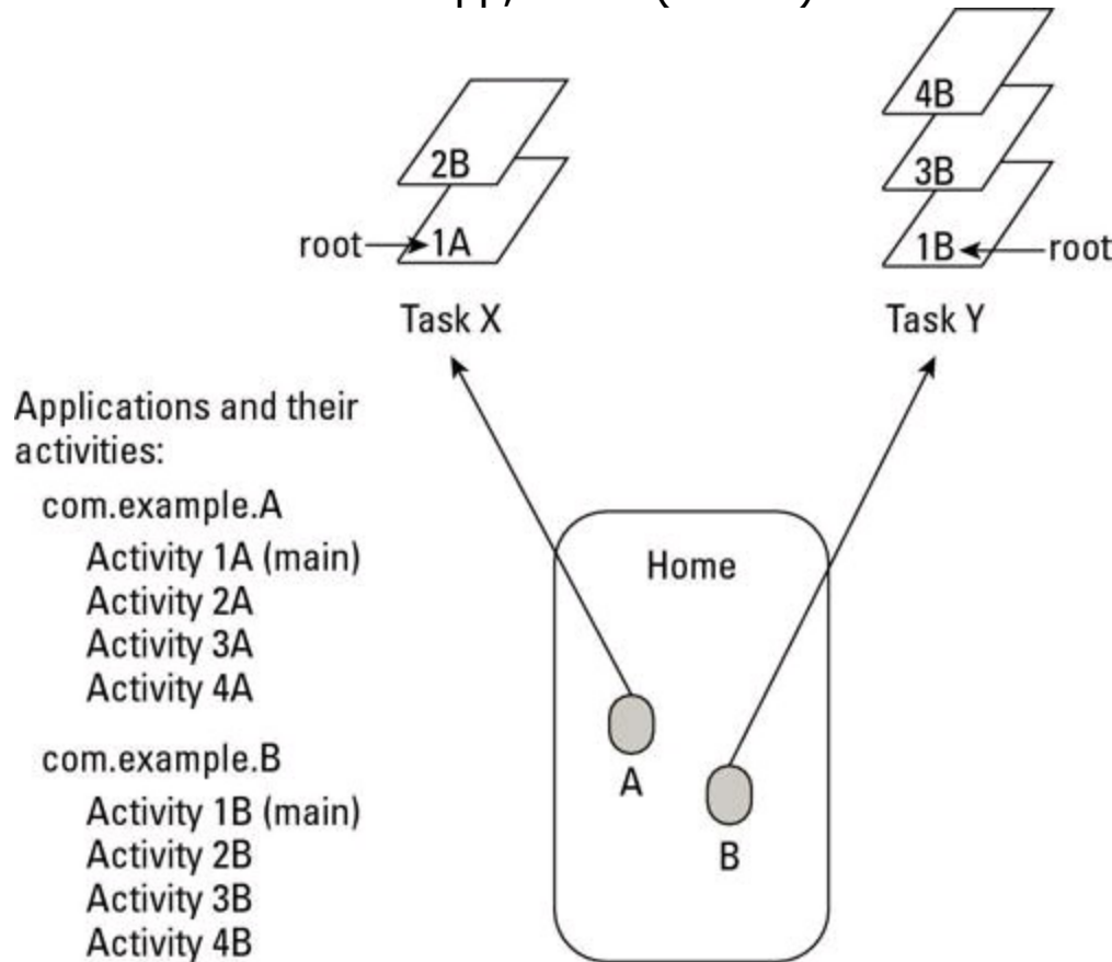
Figure 2-12: Each task has an app, which (in turn) has an icon.
