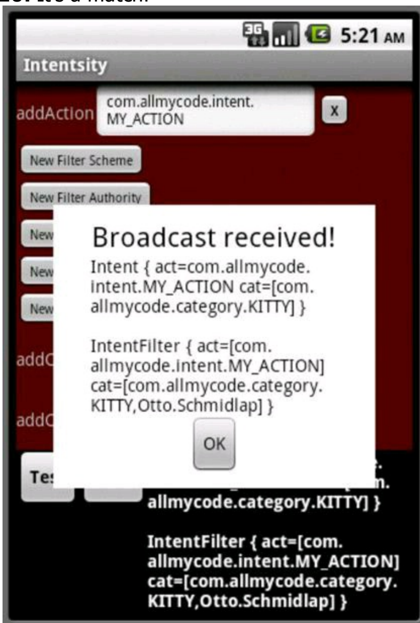
Figure 2-10: It's a match!
