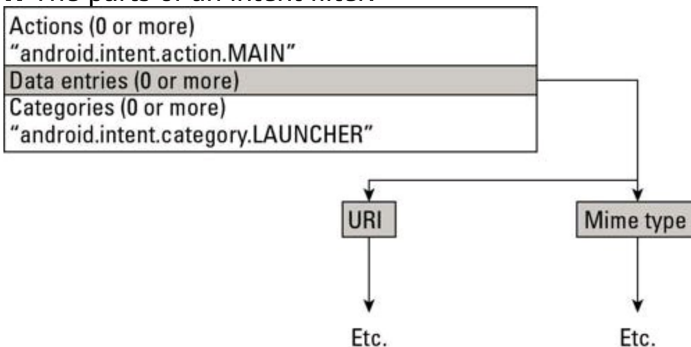
Figure 2-4: The parts of an intent filter.
