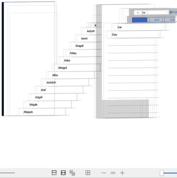
Figure 8-40. Our View Hierarchy when searching for “Zoe”
