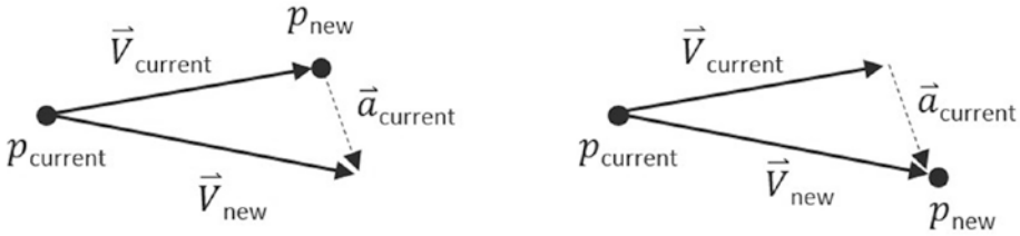
Figure 4-2. Explicit (Left) and Symplectic (Right) Euler Integration
