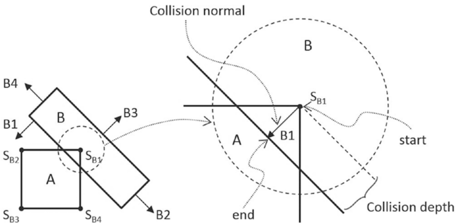
Figure 3-15. Axis of least penetration and the corresponding collision information
