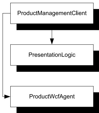
Figure 7.11 The application consists of three distinct assemblies. The ProductManagementClient assembly is the executable and contains the UI implemented in XAML with no code-behind. The PresentationLogic library contains the ViewModels and supporting classes, and the ProductWcfAgent library contains an Adapter between the custom IProductManagementAgent ABSTRACTION and the concrete WCF proxy that is used to communicate with the product-management web service. The dependency arrows imply that ProductManagementClient acts as the COMPOSITION ROOT, because it wires together the other modules.
