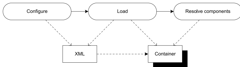
Figure 12.2 The overall usage pattern of Spring.NET involves three steps: first, we define how objects are configured and composed in an XML file. Second, we load that XML configuration into a container instance. In the third and final step, we can resolve objects from the container instance.
