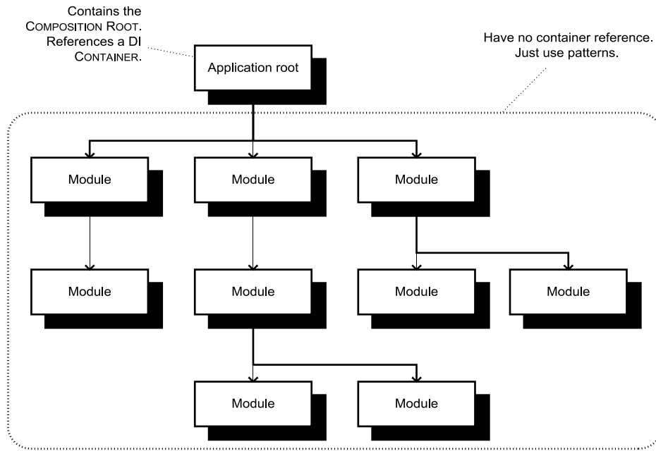
Figure 3.8 Only the COMPOSITION ROOT contained in the application root should have a reference to a DI CONTAINER. All other modules in the application should rely entirely on DI patterns and have no reference to the container.
