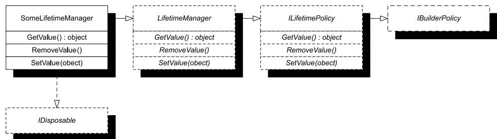
Figure 14.5 The SomeLifetimeManager implements a custom lifetime by deriving from the abstract LifetimeManager class which itself implements the ILifetimePolicy interface that derives from the IBuilderPolicy marker interface. A custom lifetime can optionally implement IDisposable to implement cleanup functionality when a container is being disposed of.
