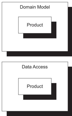
Figure 2.18 The Domain Model and Data Access libraries both define a class named Product . The Domain Product is the important class that encapsulates the Domain concept of a Product . The Data Access Product class is only an artifact of the Entity Framework wizard. It can easily be renamed or made internal.
