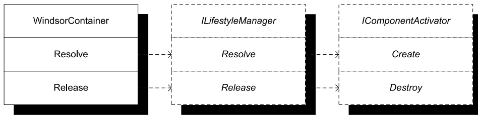
Figure 10.5 An ILifestyleManager acts as a sort of interceptor that's called instead of the underlying IComponentActivator . An ILifestyleManager implementation is expected to use the supplied IComponentActivator to create object instances. Because the ILifestyleManager sits in the middle, it gets a chance to intercept each call and perform its own lifestyle logic. It's free to reuse instances instead of calling through to the IComponentActivator each time.
