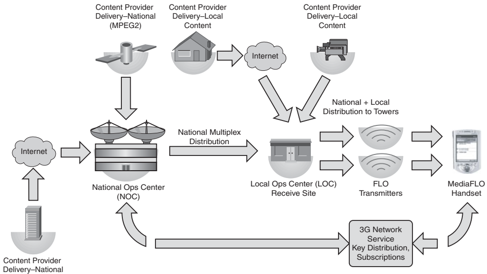
Figure 9-46 MediaFLO Architecture
