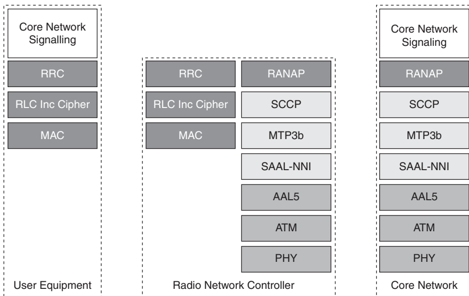
Figure 2-12 UTRAN to Core Network Control Plane
