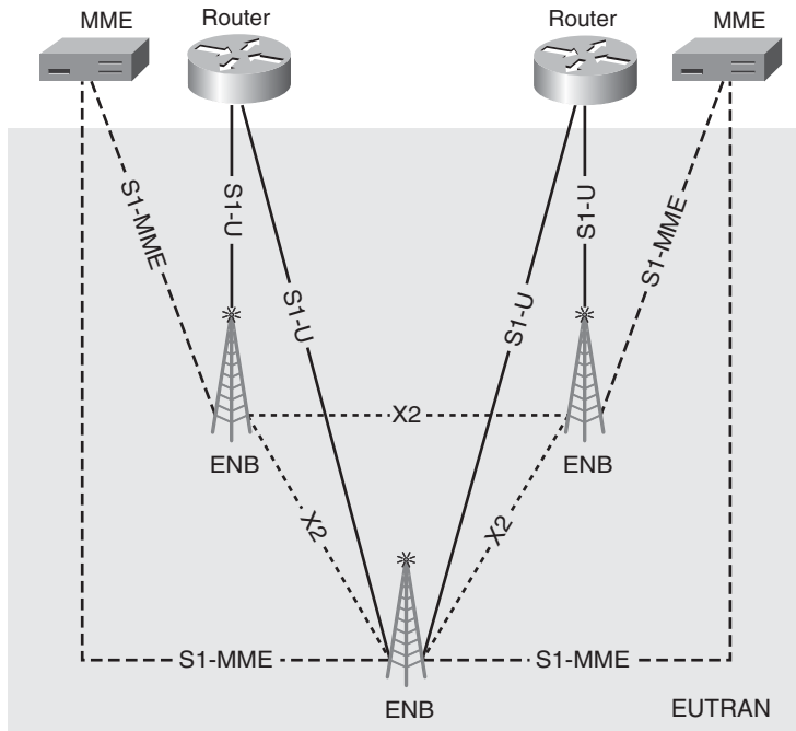
Figure 3-10 EUTRAN Architecture
