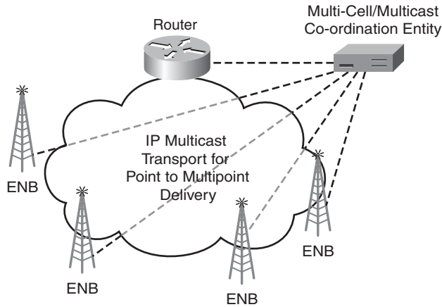
Figure 3-11 MBSFN Architecture
