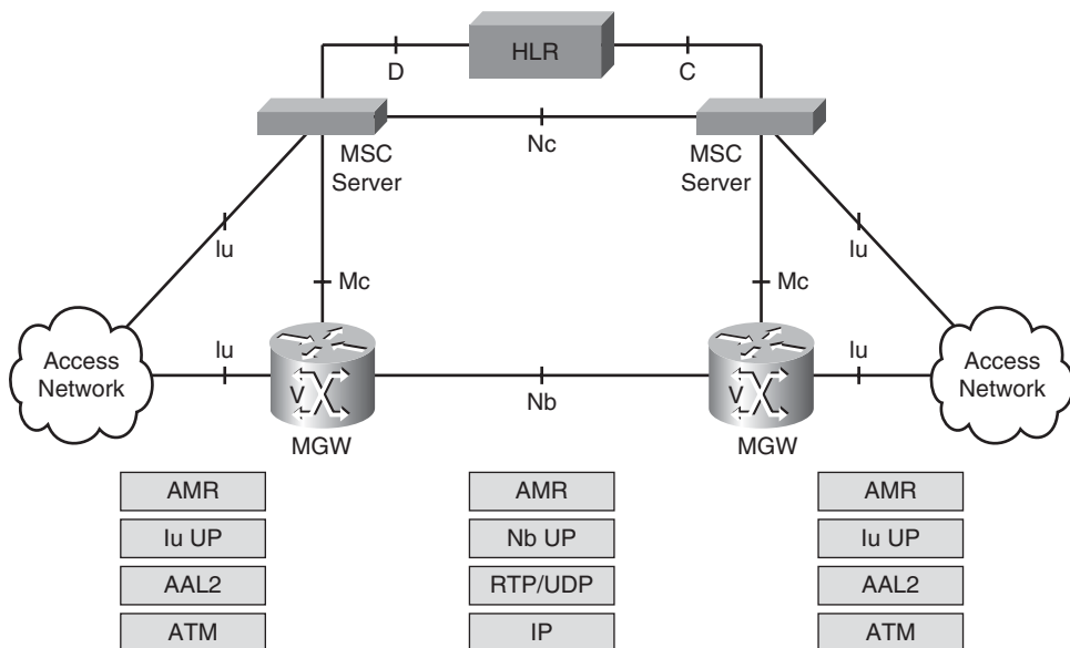
Figure 6-12 Transcoder Free Operation
