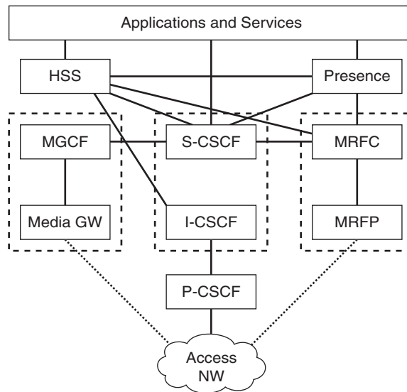
Figure 9-37 IMS Components
