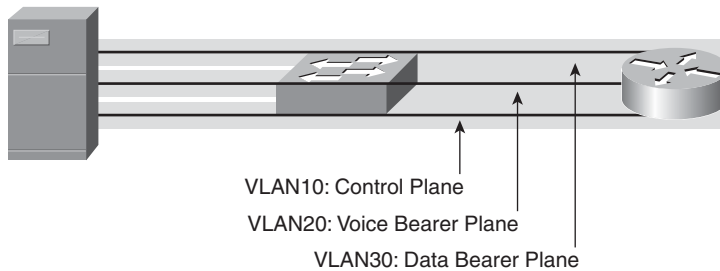
(b) Shared End-System Interface with Logically Segmented Planes
