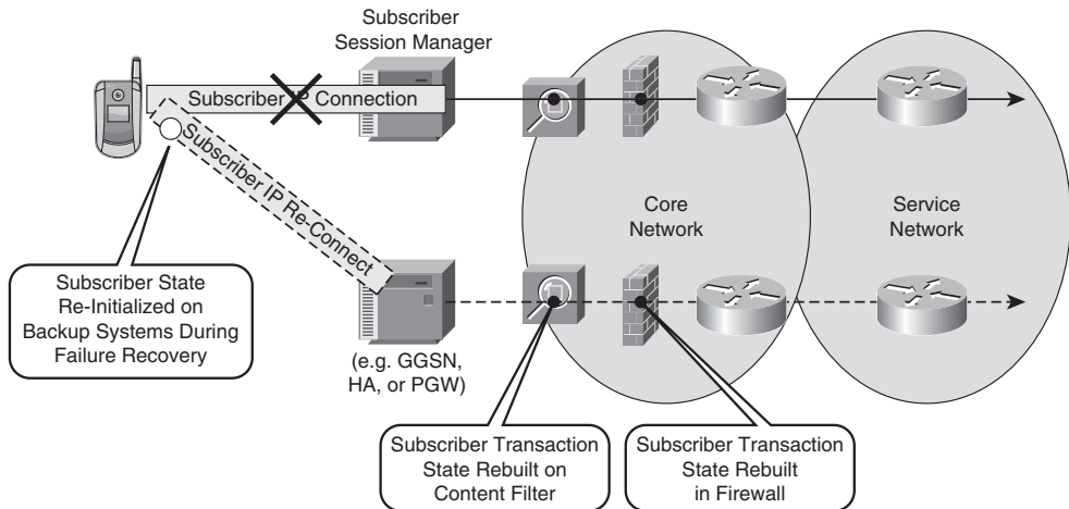
Figure 5-13 Stateless Transition of the Data Bearer Plane
