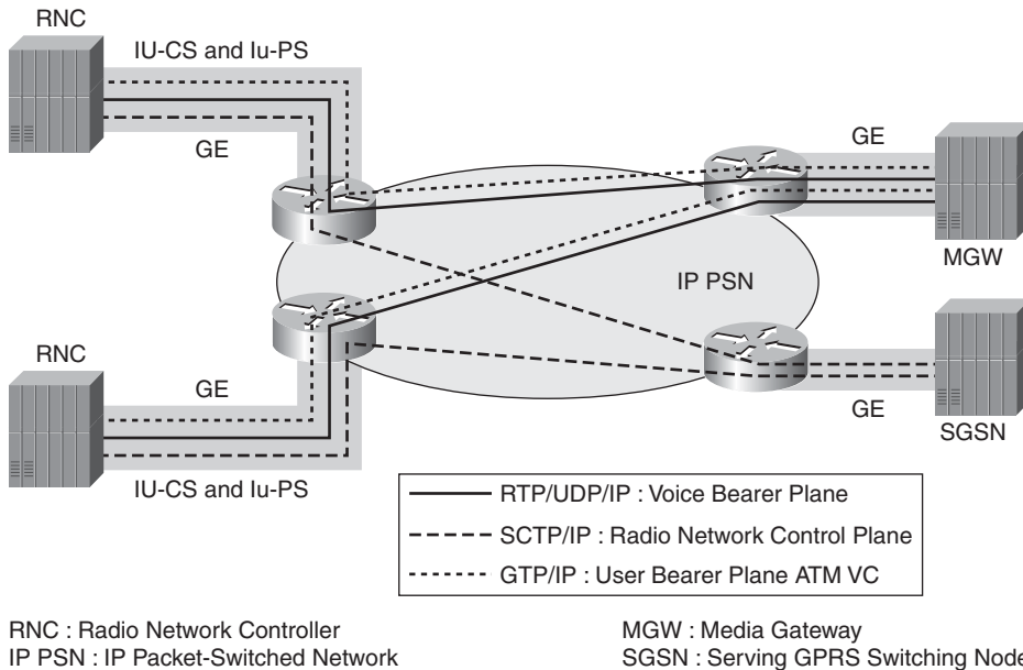
Figure 5-40 Aggregation of IuCS Traffic on PSN
