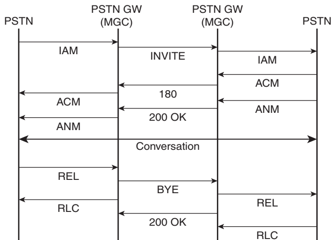
Figure 9-36 PSTN to PSTN Call with SIP Transport Network
