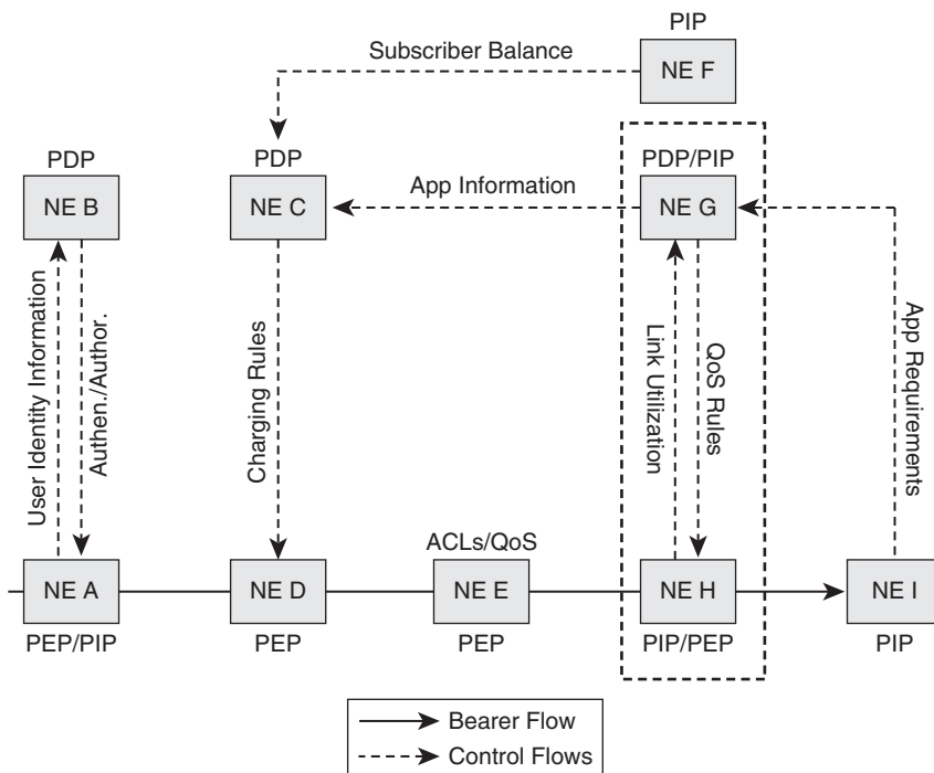
Figure 8-4 Global Policies
