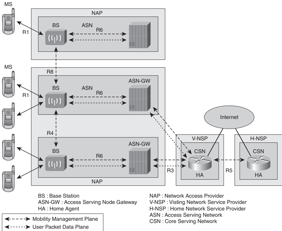
Figure 5-63 WiMAX Architecture
