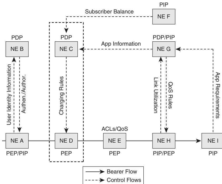
Figure 8-5 Subscriber-Specific Policies
