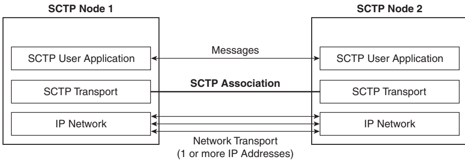
Figure 9-20 SCTP Association
