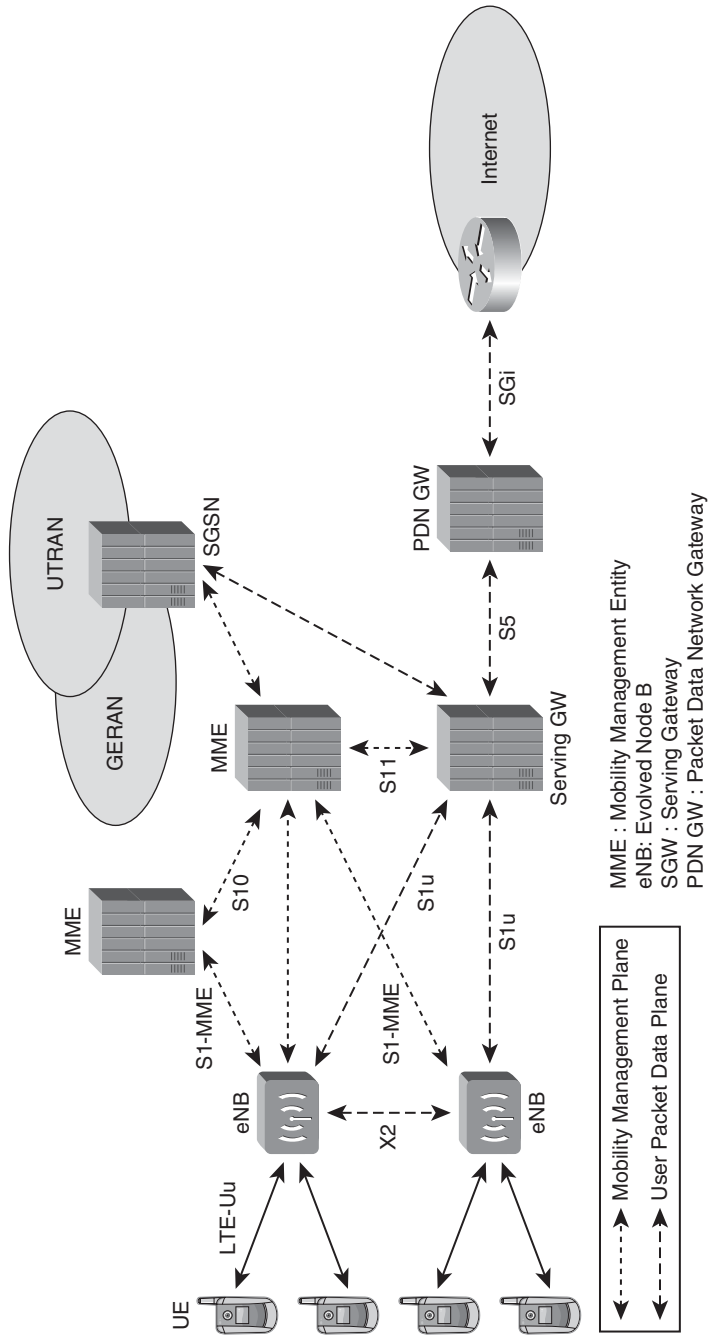
Figure 5-55 LTE/SAE Architecture
