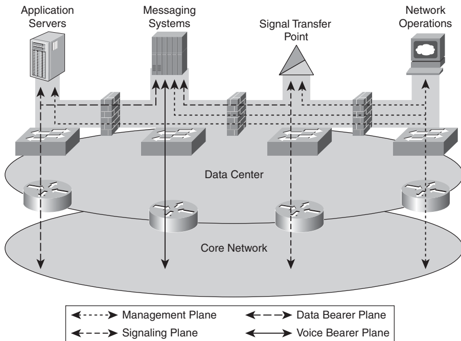
Figure 5-21 Single-Homed Application Servers
