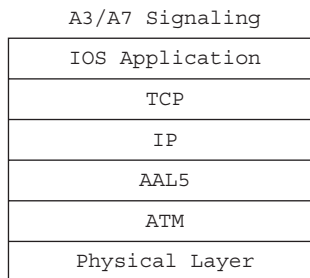
Figure 5-48 BSC to BSC Protocol Transport
