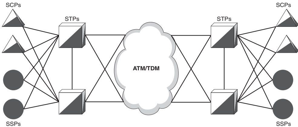
Figure 9-10 SS7 Architecture
