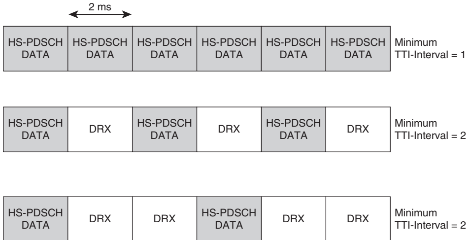
Figure 2-18 Inter TTI Interval Operation
