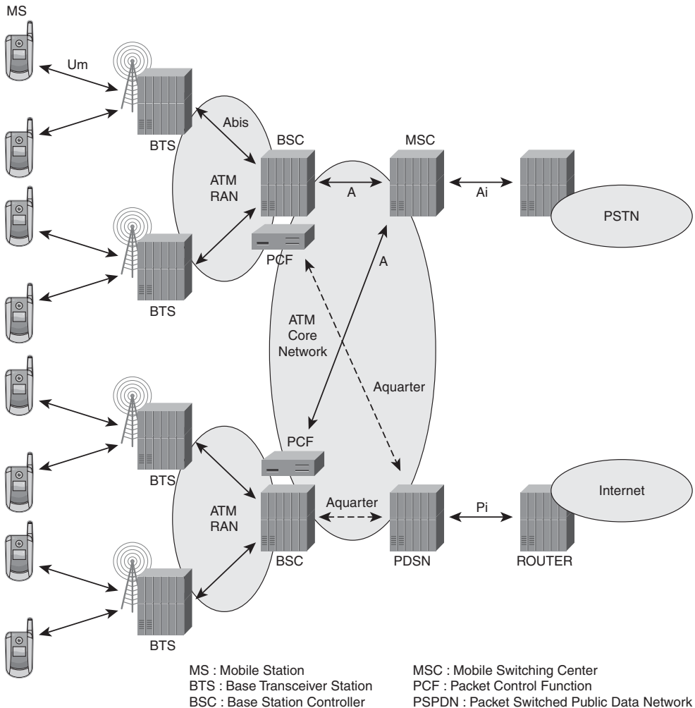
Figure 5-42 ATM-Switching Infrastructure for CDMA
