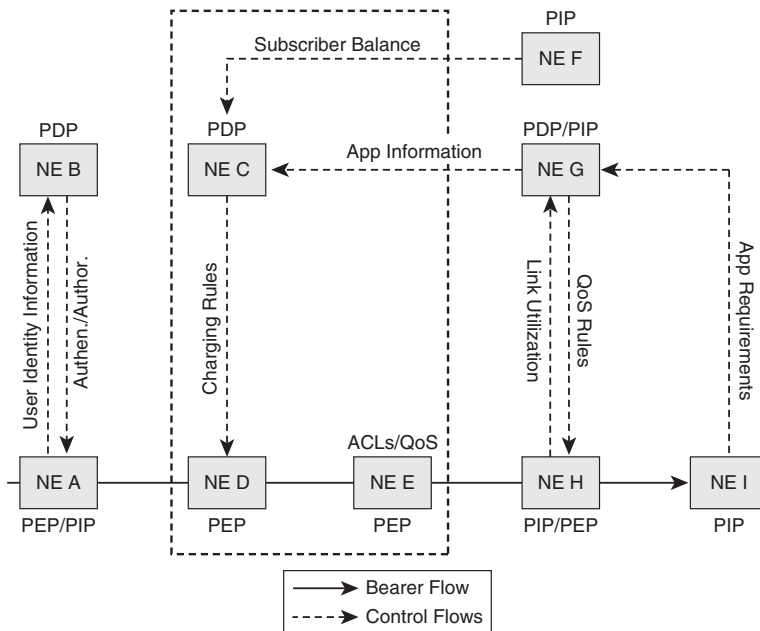
Figure 8-2 Proactive Policies
