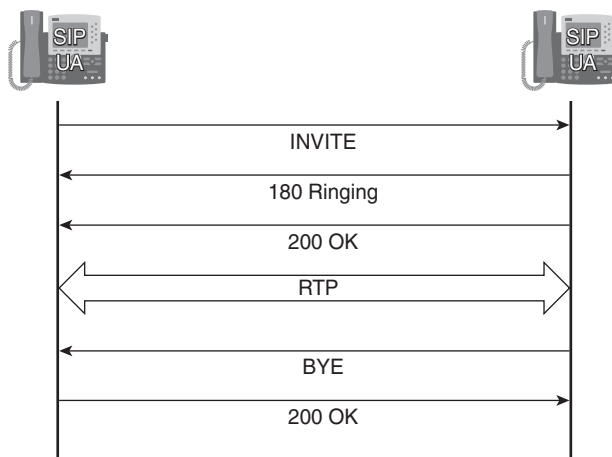
Figure 9-32 BYE Method
