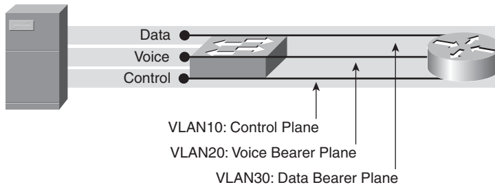
(a) Distinct End-System Interfaces for Segmented Planes
