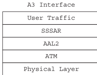
Figure 5-53 Voice Transport on A3 Interface
