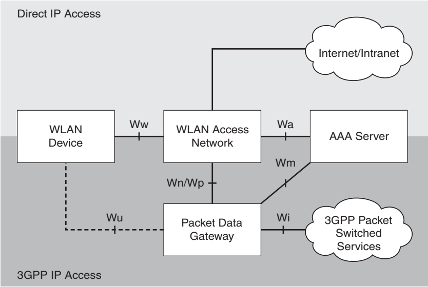
Figure 3-1 I-WLAN Architecture
