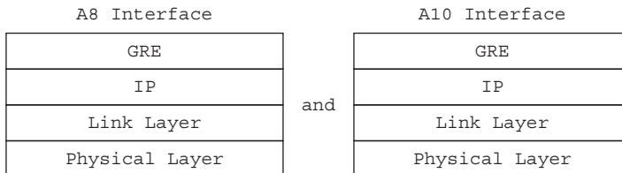
Figure 5-54 Data Transport on A8/A10 Interface
