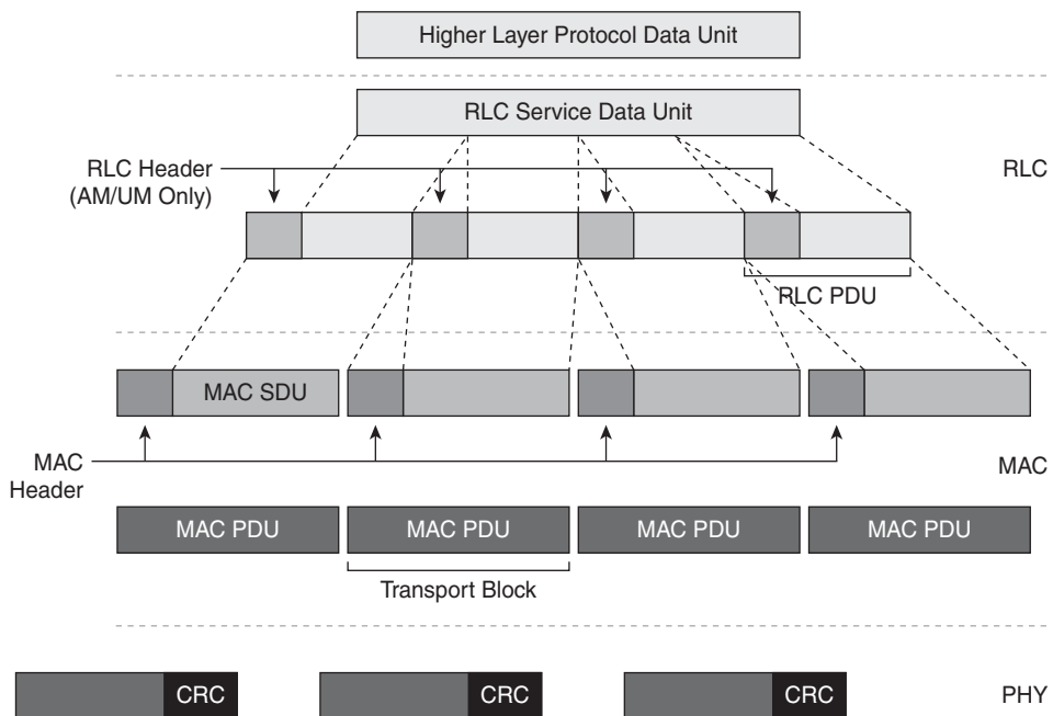
Figure 2-13 UMTS RLC/MAC Functions
