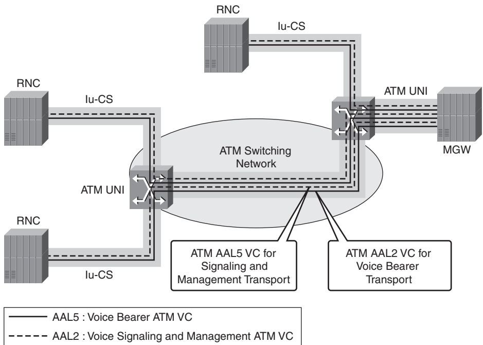
Figure 5-39 Aggregation of IuCS Traffic
