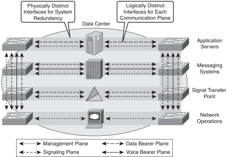
Figure 5-20 Multi-Homed Application Servers
