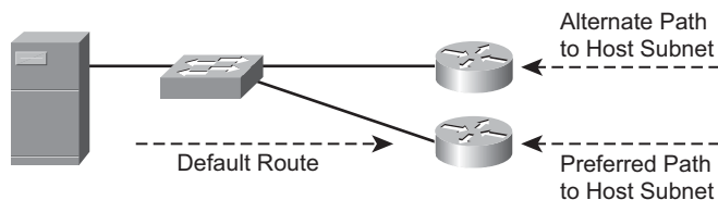
Figure 4-45 Single-Homed End-System
