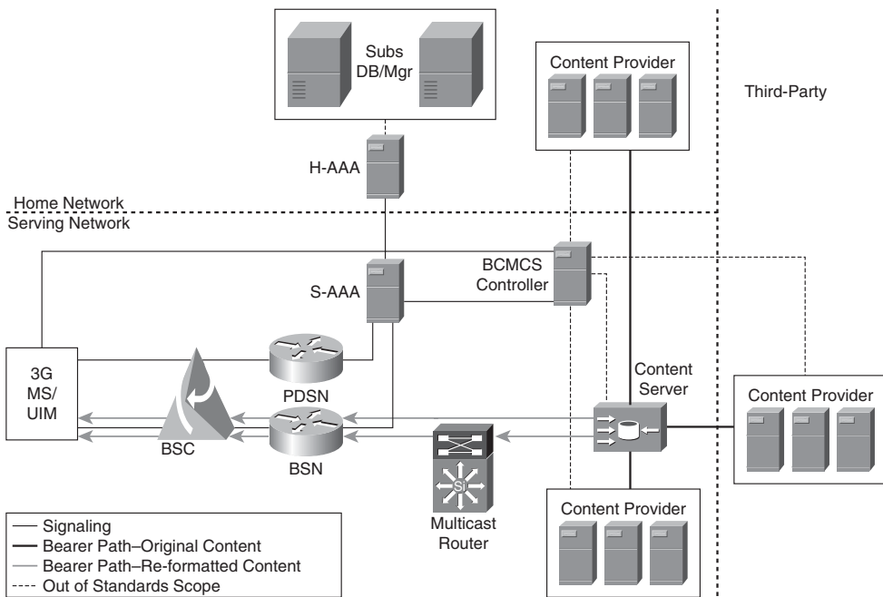
Figure 9-42 BCMCS Architecture
