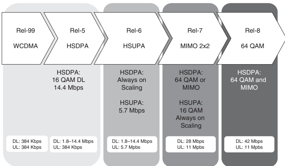
Figure 2-21 HSPA+ Radio Interface Evolution
