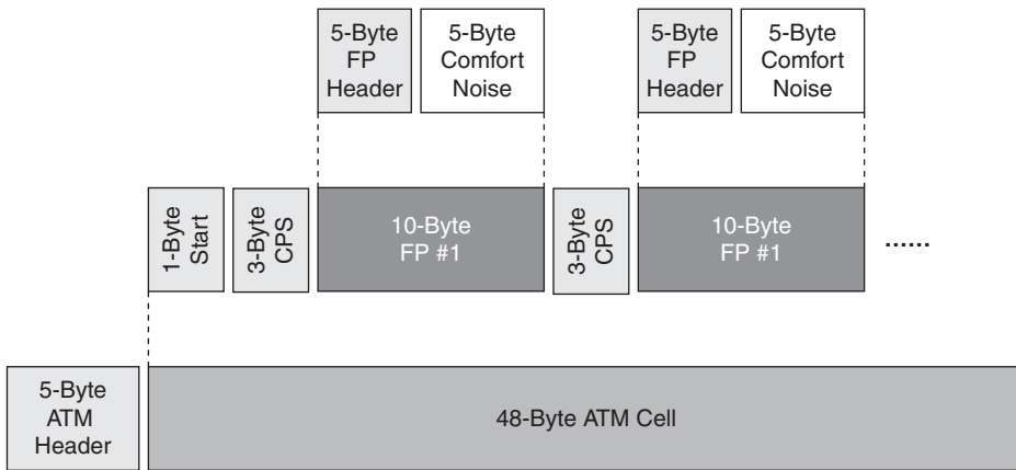
Figure 2-15 Iub SID Transport for Voice Inactivity
