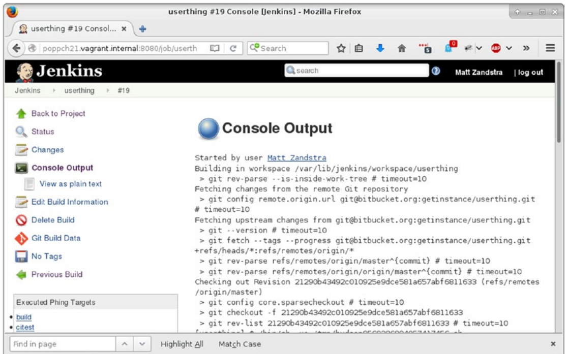
Figure 21-9. Console output
