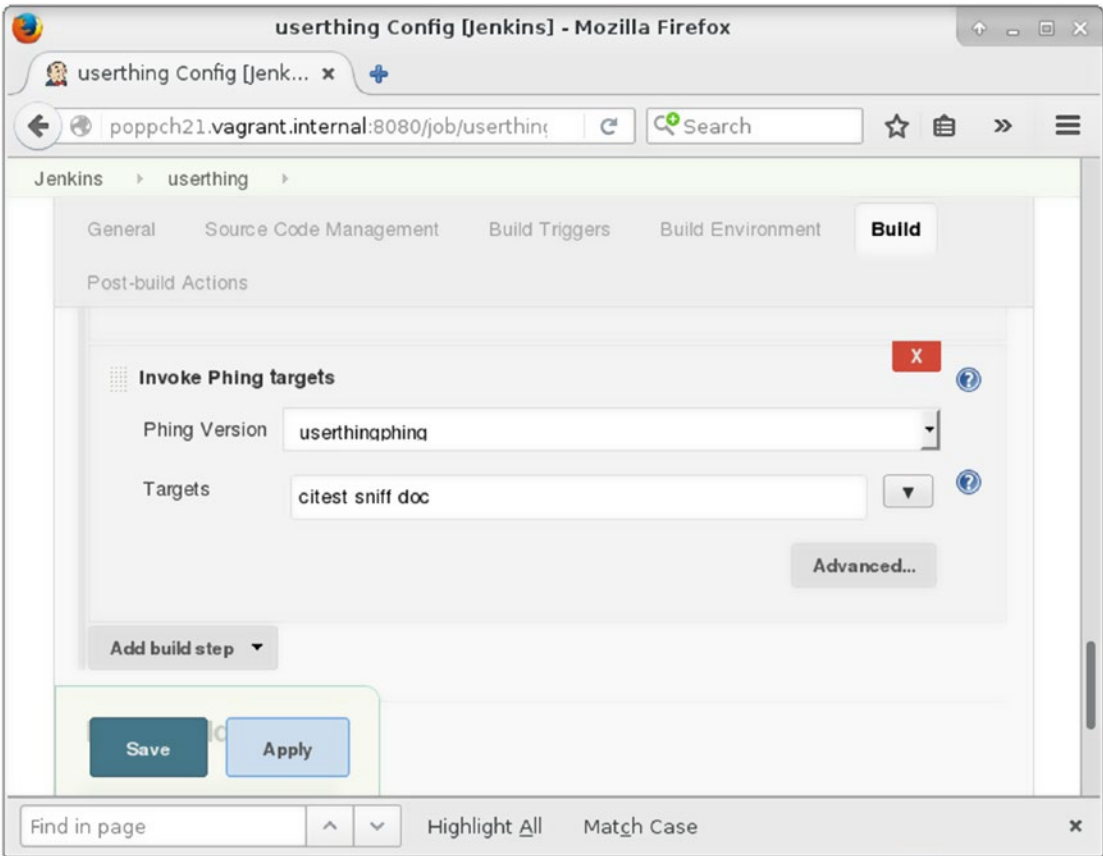
Figure 21-8. Configuring Phing
