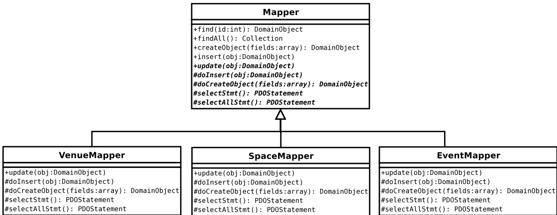
Figure 13-1. Mapper classes
