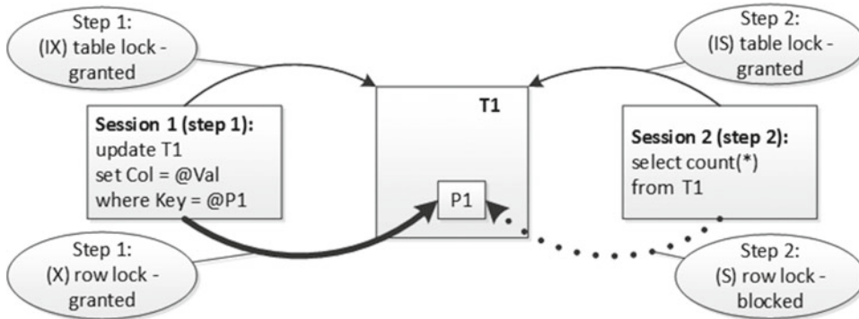
Figure 23-3. Deadlock due to mixed DDL and DML statements: Step 1
