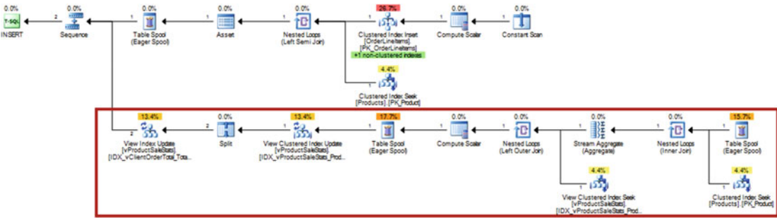
Figure 10-8. Execution plan of a query that inserts data into OrderLineItems table
