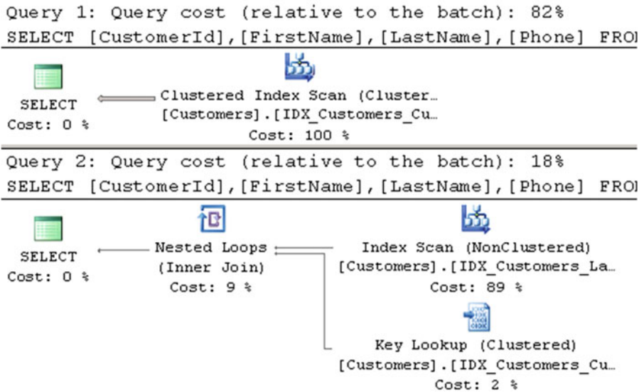
Figure 3-4. Column-level statistics: Execution plans
