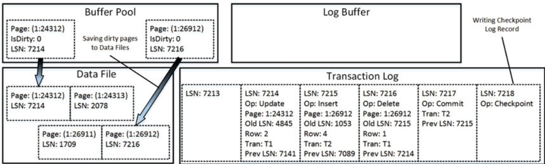
Figure 30-5. Data modifications: CHECKPOINT
