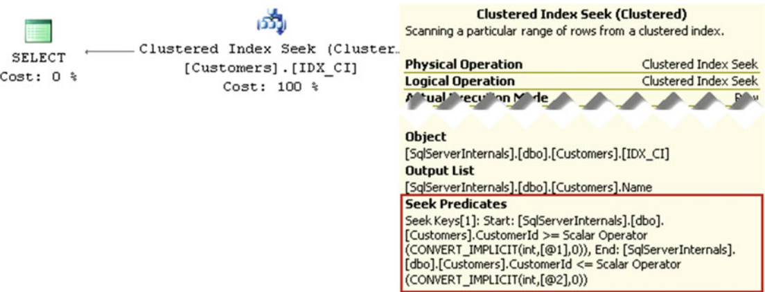
Figure 2-13. Index seek execution plan
