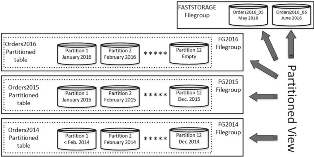
Figure 16-6. Using partitioned tables and views together: Data layout
