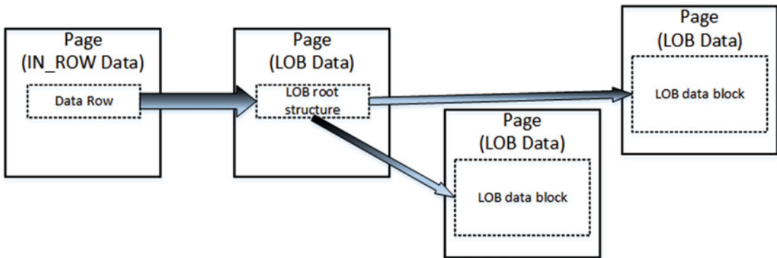
Figure 1-13. LOB data: Logical structure
