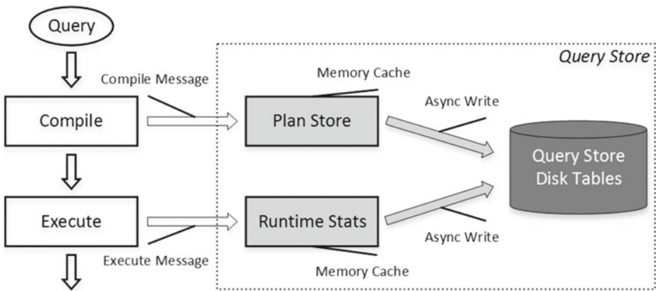
Figure 29-2. High-level SQL Server Query Store workflow
