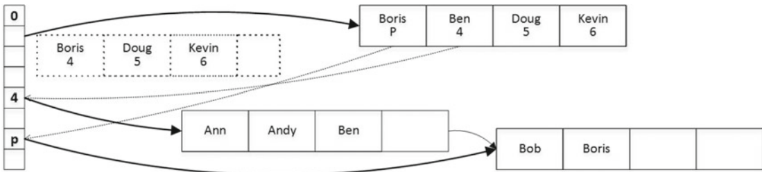
Figure 35-14. Page splitting: Second step
