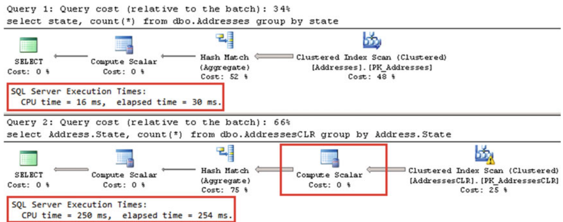
Figure 15-2. UDT performance: Querying the data
