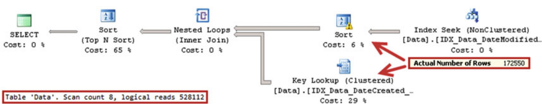
Figure 16-15. Execution plan with index hint
