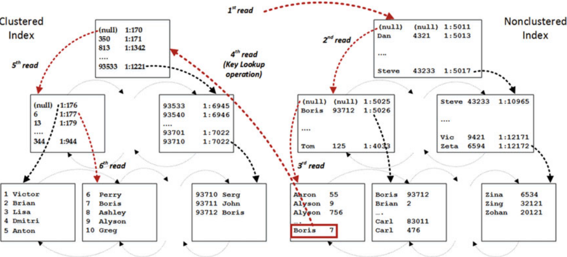
Figure 2-18. Nonclustered index usage: Step 1
