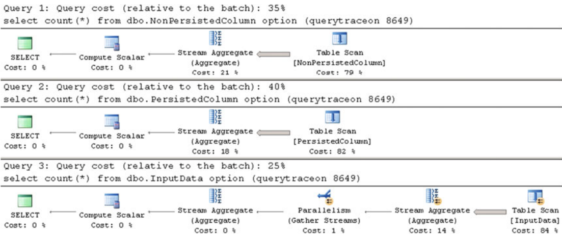
Figure 4-13. Calculated columns and parallel execution plans
