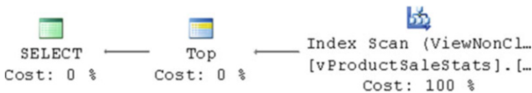
Figure 10-9. Execution plan of a query that does not reference the indexed view (Enterprise or Developer editions)
