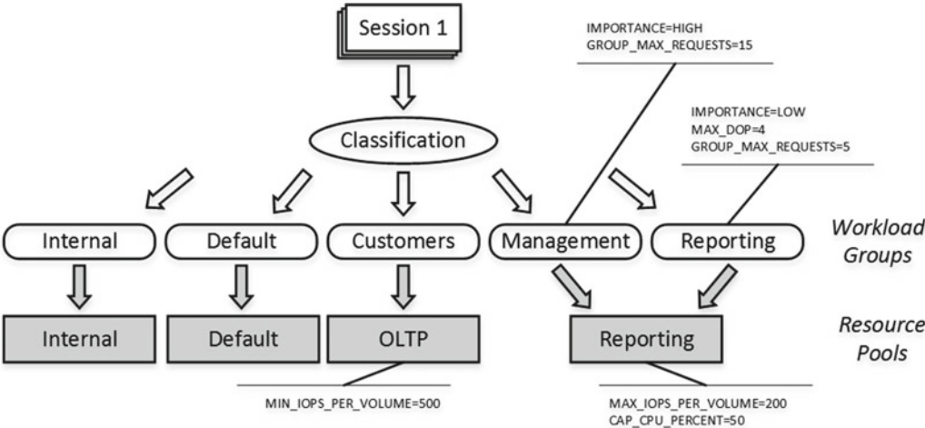
Figure 28-1. Example of Resource Governor configuration
