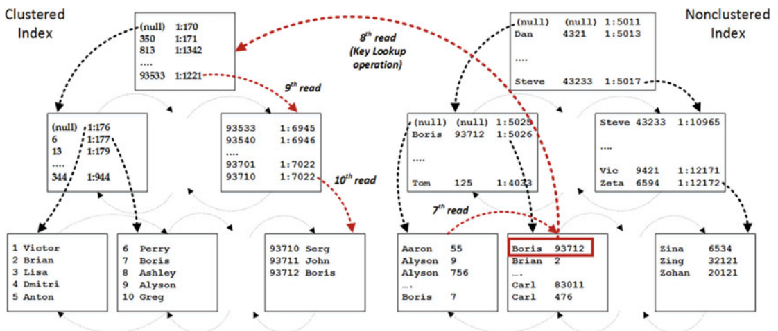
Figure 2-19. Nonclustered index usage: Step 2
