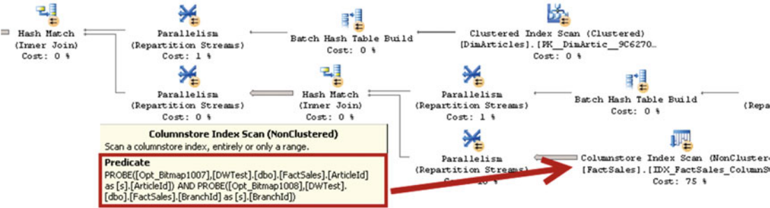
Figure 33-23. Execution plan for a query that uses a dimensions table to filter the article category
