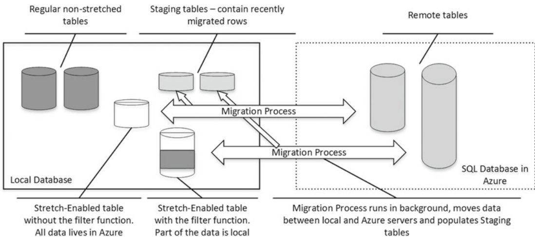
Figure 5-9. Stretch database overview
