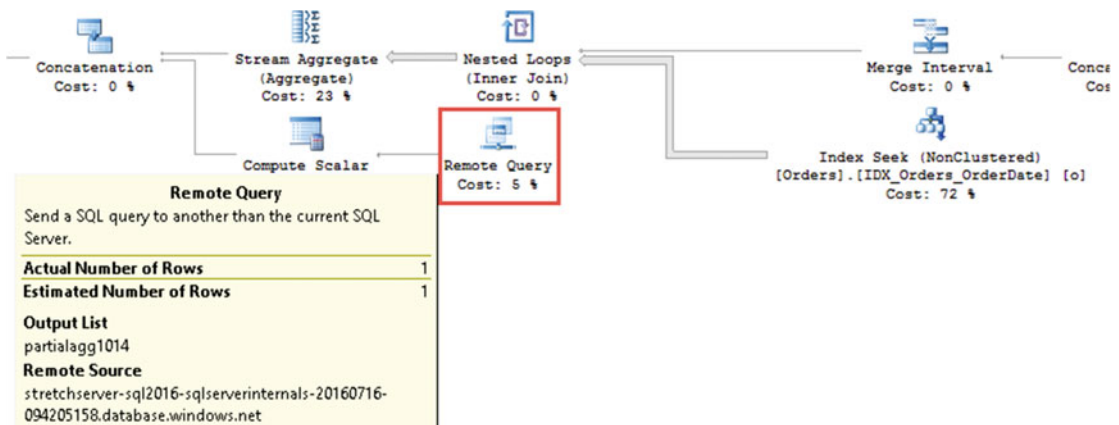
Figure 5-10. Execution plan: Counting total number of orders
