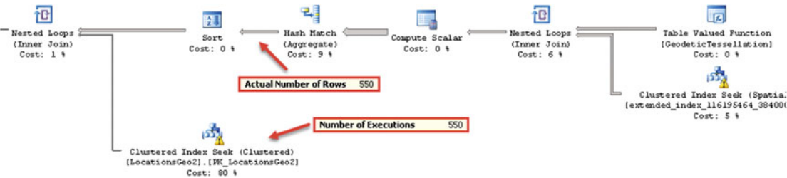
Figure 15-8. Customer-based POI 'lookup: Execution plan for the second query
