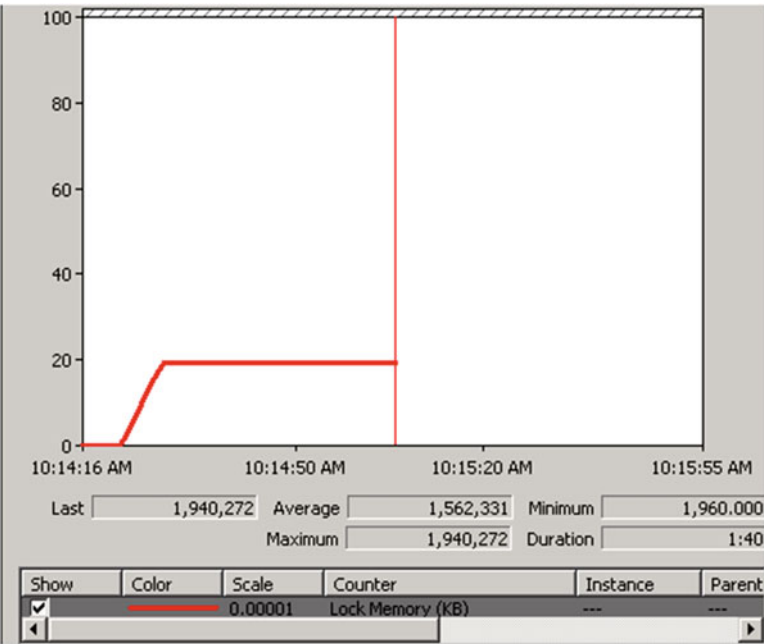
Figure 20-1. Lock Memory (KB) system performance counter
