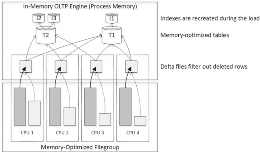
Figure 35-28. Loading data to memory
