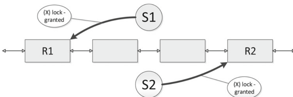
Figure 19-1. Classic deadlock, step 1
