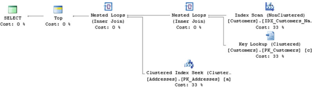
Figure 25-9. Execution plan without blocking operators
