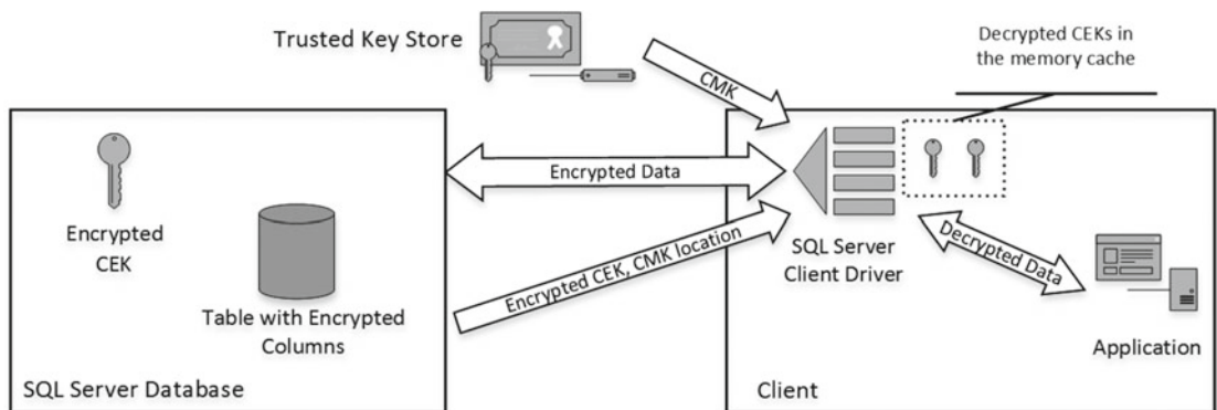
Figure 5-19. Always Encrypted workflow
