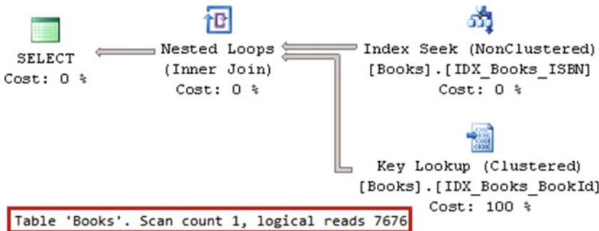
Figure 2-20. Selecting data for the single prefix: Execution plan
