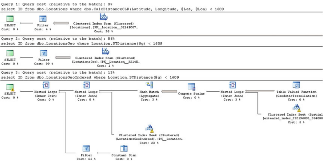
Figure 15-6. POI Lookup: Execution plans
