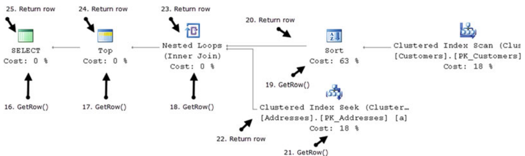
Figure 25-7. Row-based model: Getting the subsequent row
