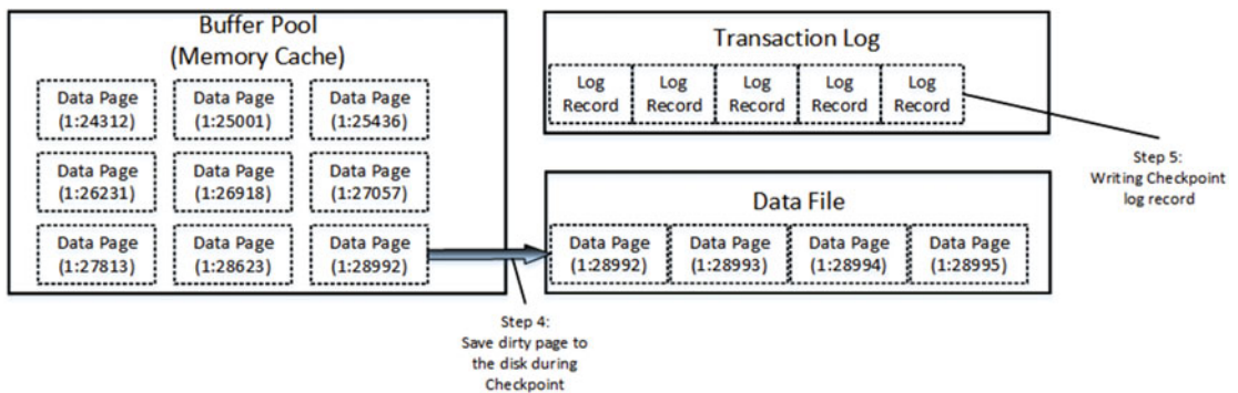
Figure 1-19. Data modification: Checkpoint
