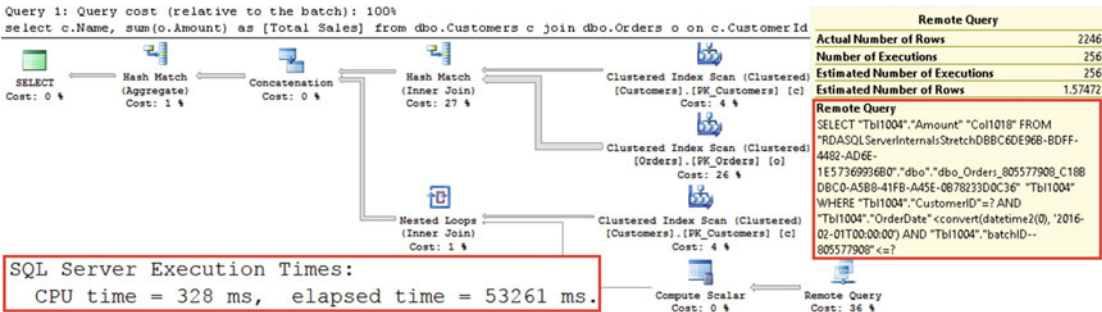
Figure 5-12. Execution plan: Filtering by PostalCode
