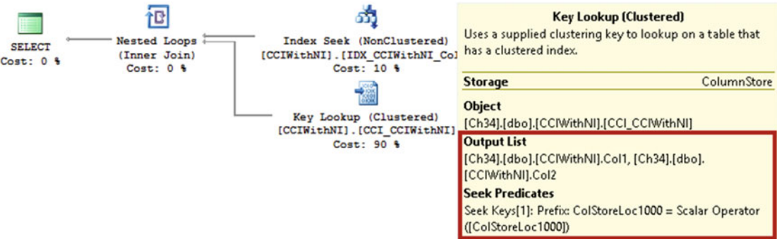
Figure 34-18. Execution plan with nonclustered B-Tree index seek
