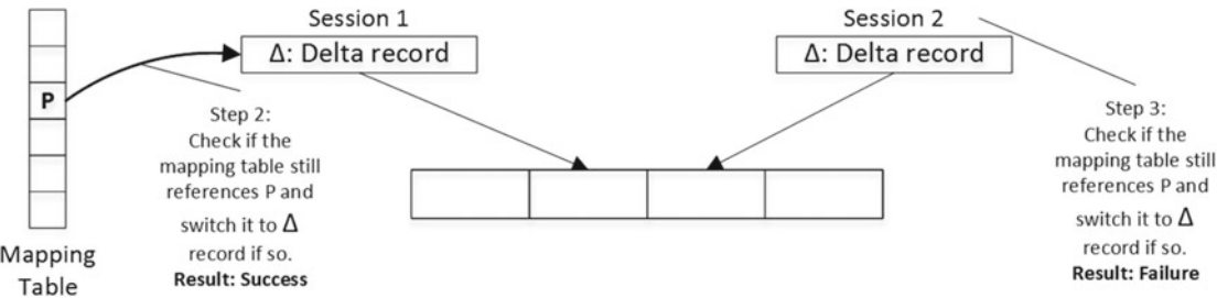
Figure 35-9. Data modifications and concurrency: Steps 2 and 3
