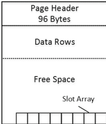
Figure 1-6. The data page structure
