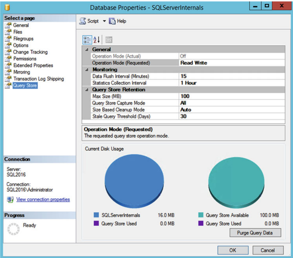
Figure 29-1. Query Store configuration in SSMS
