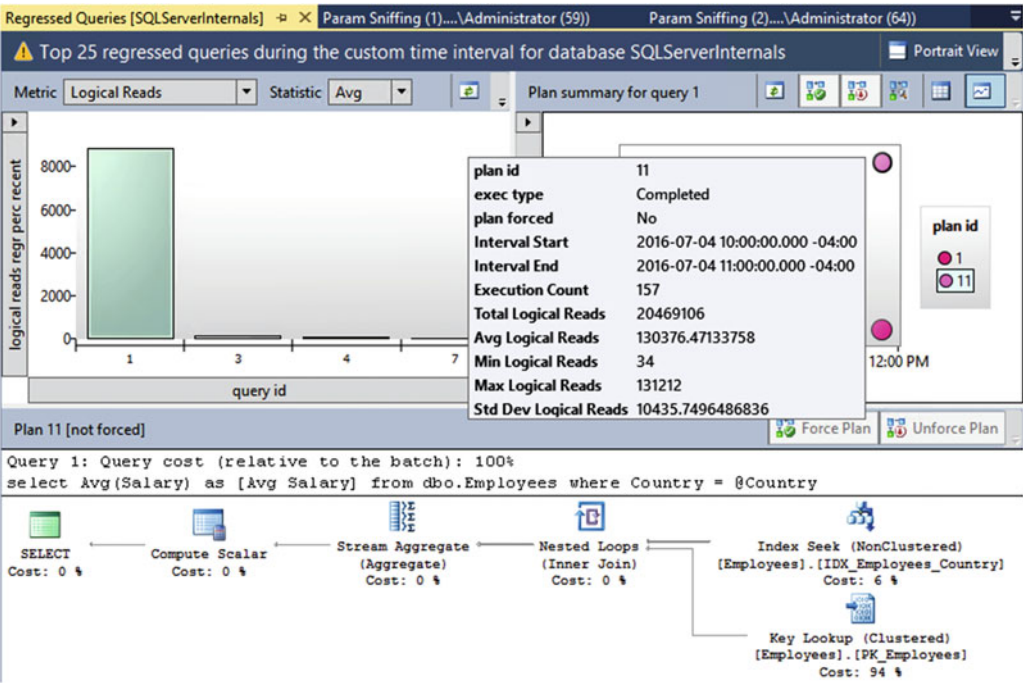
Figure 29-6. Regressed Queries report
