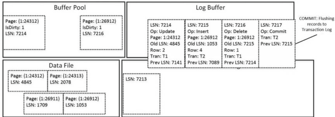
Figure 30-4. Data modifications: Commit
