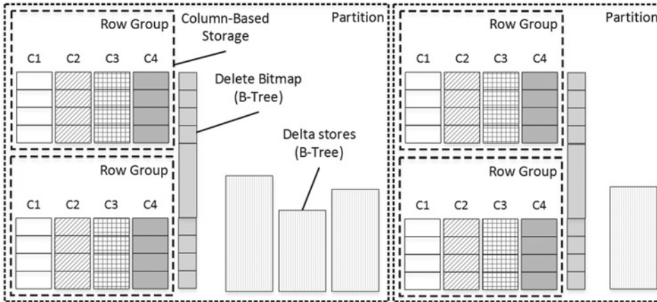
Figure 34-2. Clustered columnstore index structure
