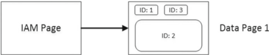
Figure 2-3. Forwarding pointers and I/O: Data pages after table creation
