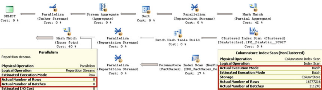
Figure 33-15. Execution plan with a columnstore index scan and batch mode execution (SQL Server 2012)
