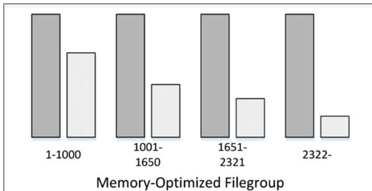
Figure 35-27. Database with multiple data and delta files
