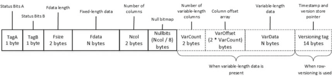
Figure 1-7. Data row structure
