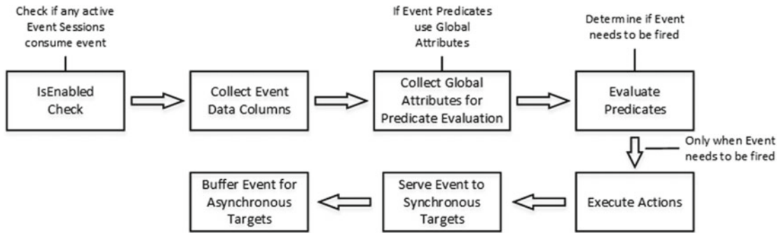
Figure 27-1. Extended Events life cycle
