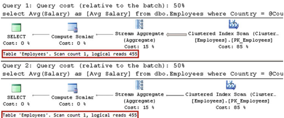
Figure 26-1. Parameter sniffing: Cached plan for @Country='USA'
