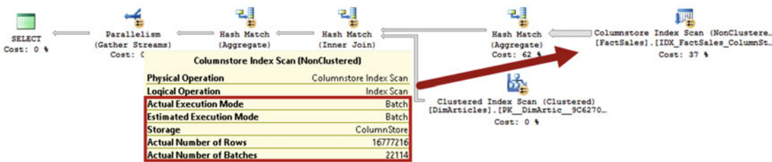
Figure 33-16. Execution plan with a columnstore index scan and batch mode execution (SQL Server 2014 and 2016)
