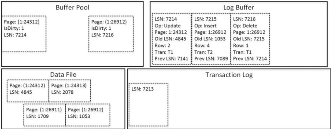
Figure 30-3. Data modifications: T1 and T2 change data on another page
