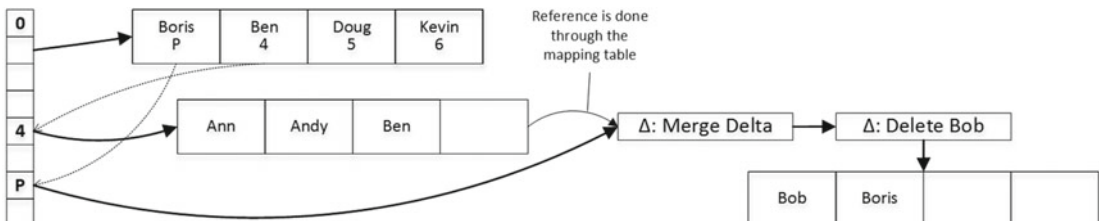
Figure 35-15. Page merging: First step
