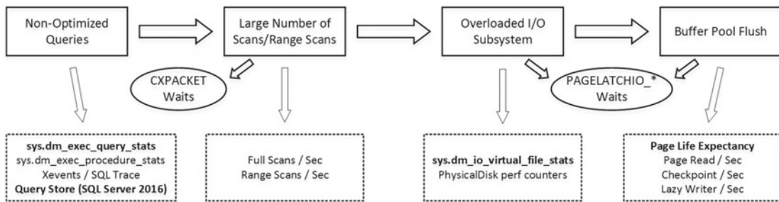
Figure 28-7. Nonoptimized queries troubleshooting
