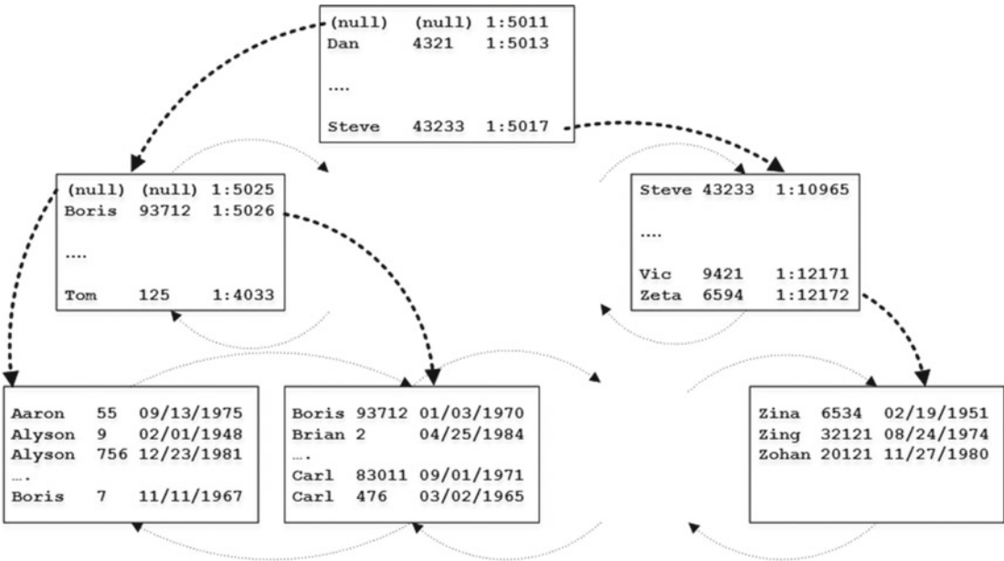
Figure 4-1. Structure of an index with included columns
