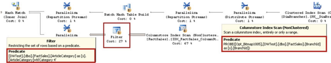
Figure 33-24. Execution plan for a query that uses a string attribute in the facts table to filter the article category (prior to SQL Server 2016)
