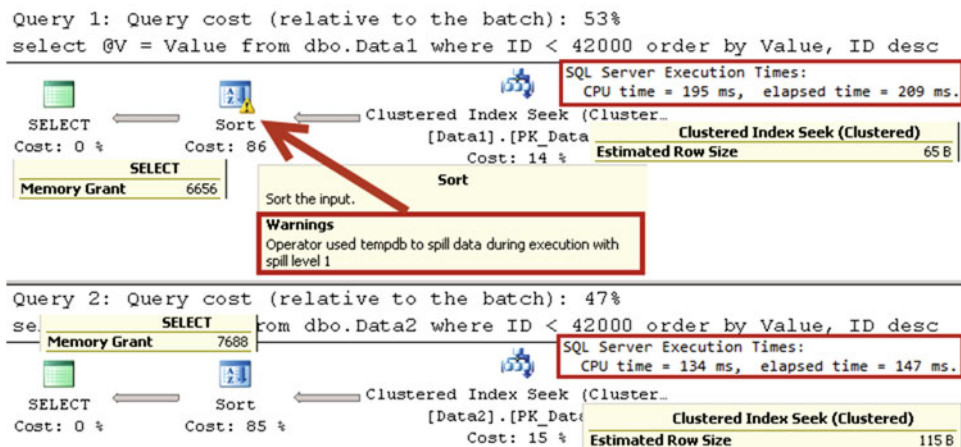
Figure 25-8. Variable-length columns and memory grant: Execution plan
