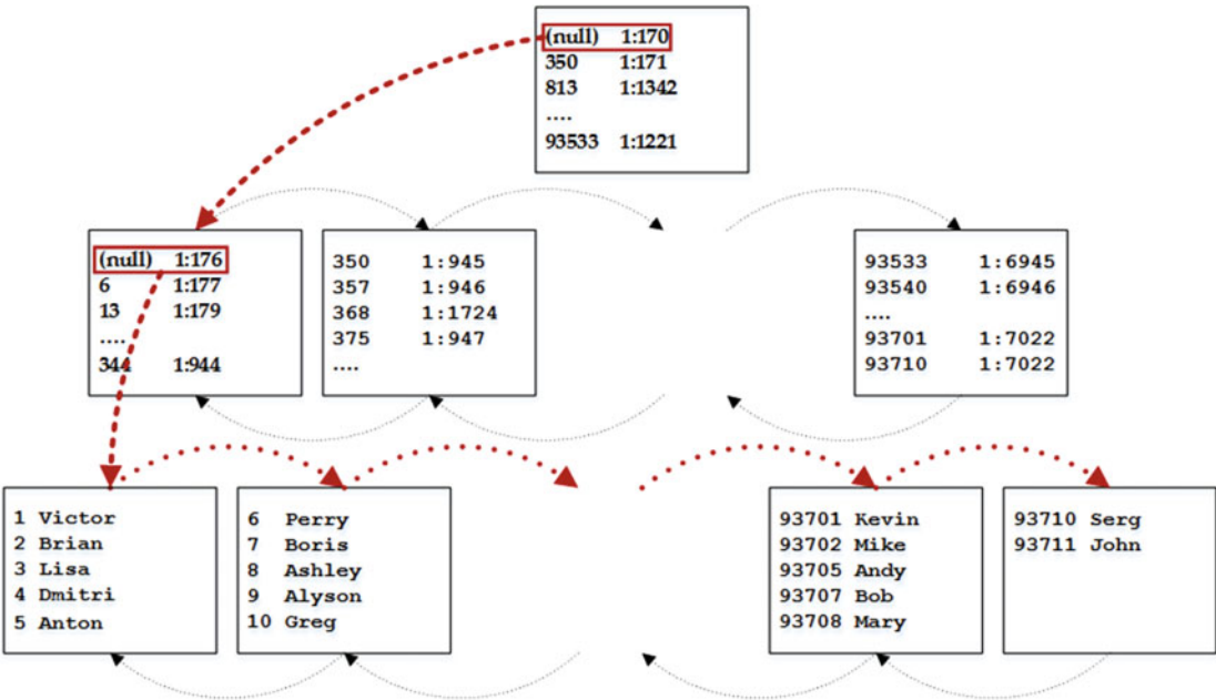
Figure 2-8. Ordered index scan
