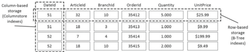
Figure 33-3. Row-based and column-based storage
