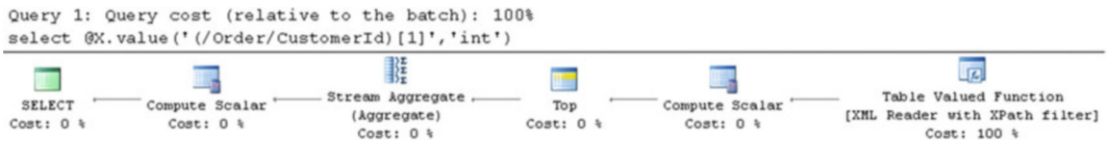
Figure 12-5. Typed XML and atomization of nodes
