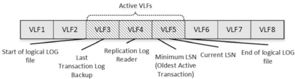
Figure 30-13. FULL and BULK LOGGED recovery models: Initial stage
