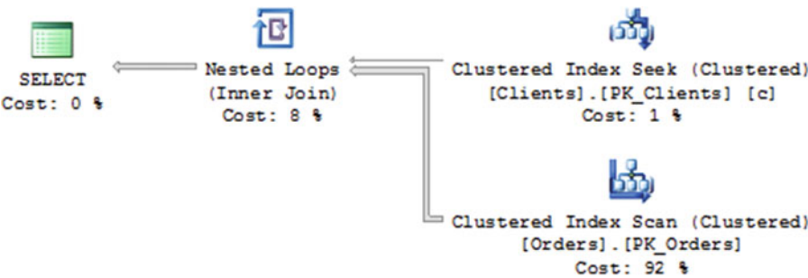
Figure 11-10. Execution plan of query without an inline table-valued function
