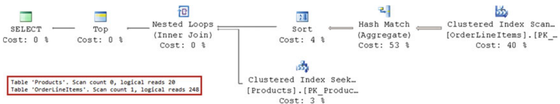
Figure 10-6. Execution plan of a query that selects the top 10 most popular products
