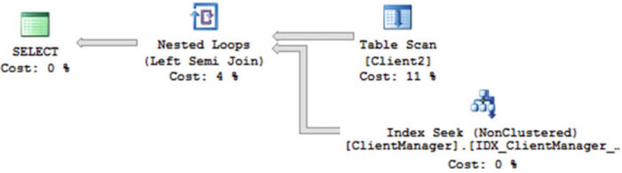
Figure 5-18. Execution plan with lookup table after index creation
