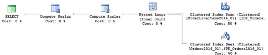
Figure 16-5. Execution plan of an optimized query
