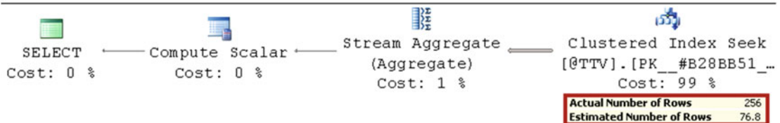
Figure 13-6. Cardinality estimations for temporary tables and table variables
