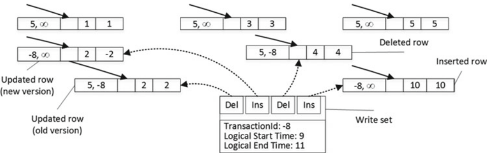
Figure 36-4. Start of validation phase
