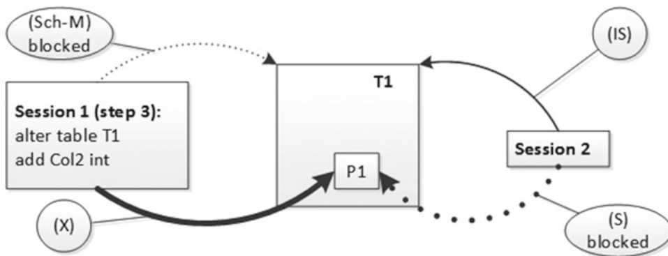
Figure 23-4. Deadlock due to mixed DDL and DML statements: Step 2
