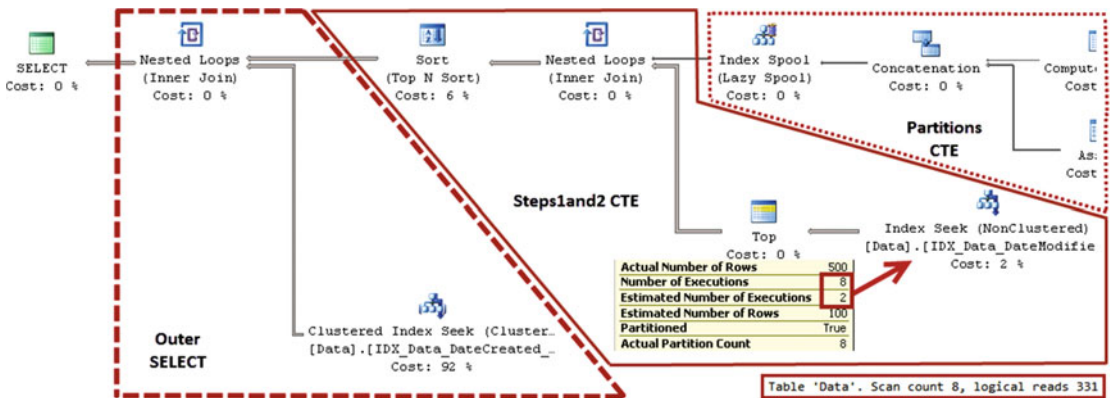
Figure 16-17. Execution plan of the optimized query
