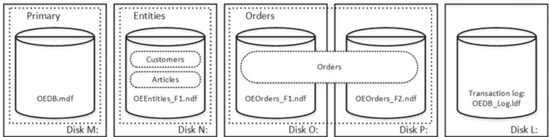
Figure 1-2. Physical layout of the tables
