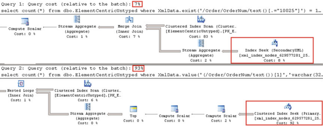
Figure 12-7. Comparing the exist() and value() methods
