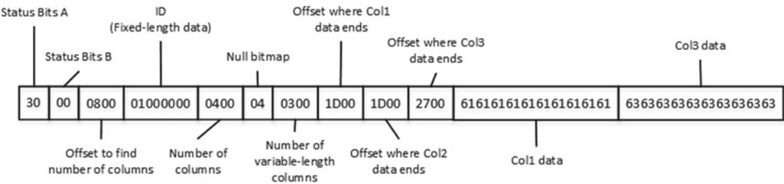
Figure 1-9. First data row
