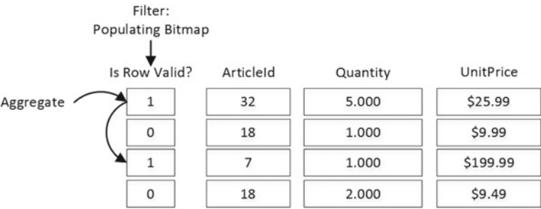
Figure 33-5. Batch mode execution
