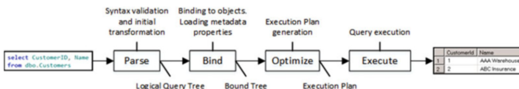
Figure 25-1. Query life cycle
