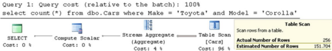
Figure 4-10. Cardinality estimation with correlated predicates (legacy cardinality estimator)
