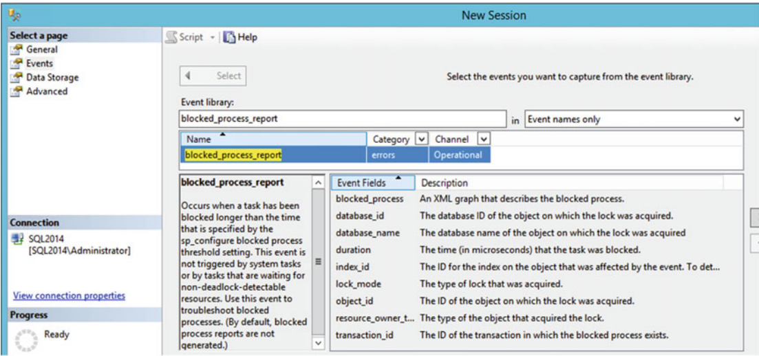
Figure 18-6. Capturing blocked process report with Extended Events
