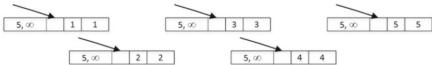
Figure 36-2. Data in the dbo.HKData table after insert
