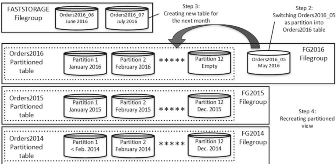
Figure 16-12. Tiered storage in action: Further steps
