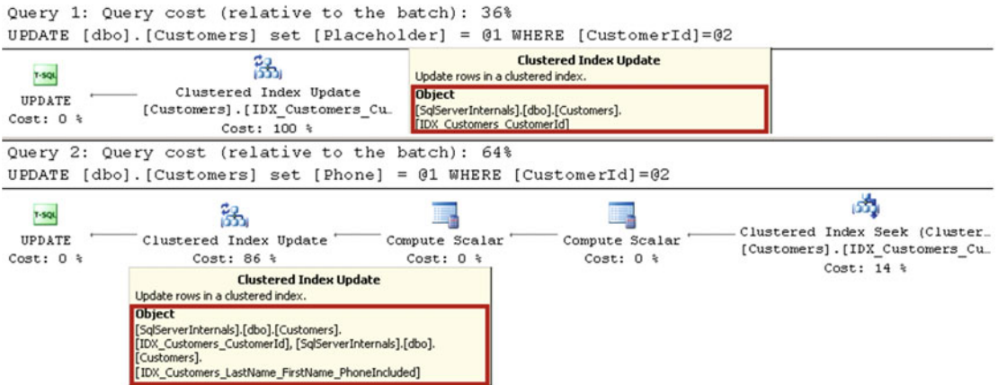
Figure 4-4. Execution plans for UPDATE statements
