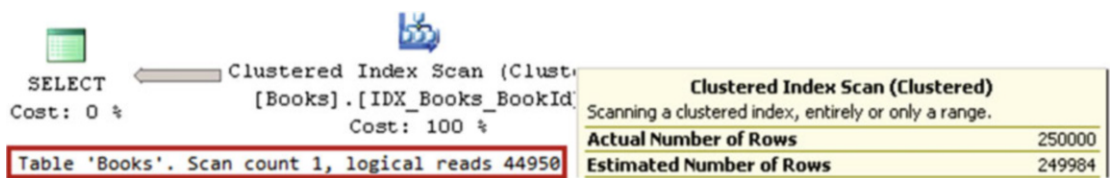
Figure 3-9. Execution plan for the query selecting rows with the 999 prefix after a statistics update
