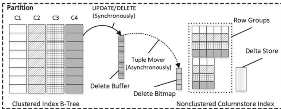
Figure 34-19. Partition of the table with a nonclustered columnstore index
