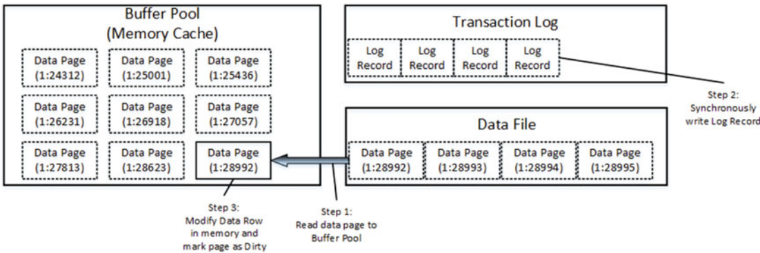
Figure 1-18. Data modification: Modifying data
