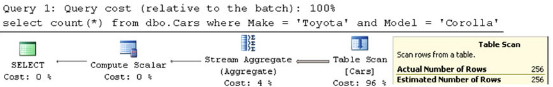
Figure 4-12. Cardinality estimation with filtered statistics
