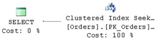
Figure 10-4. Execution plan with inner join when foreign-key constraint is present
