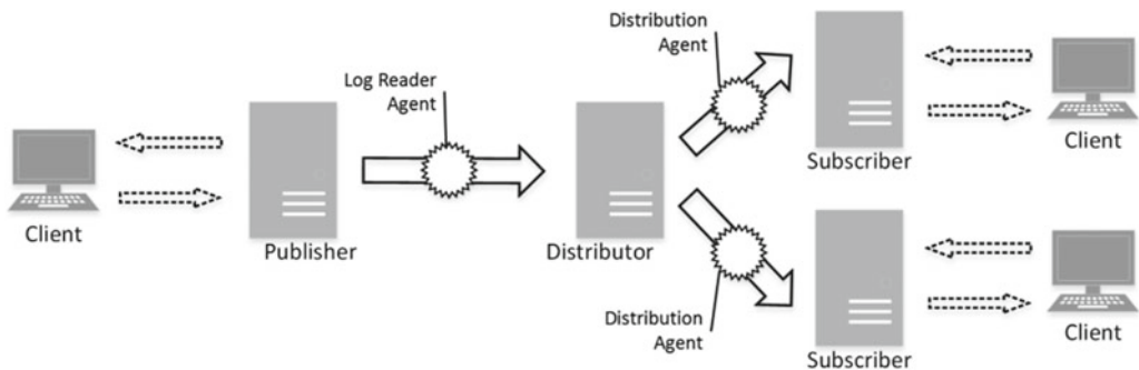
Figure 32-9. Transactional replication with push subscriptions
