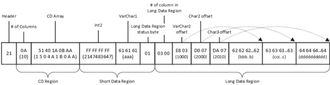
Figure 4-18. Row compression: Row data
