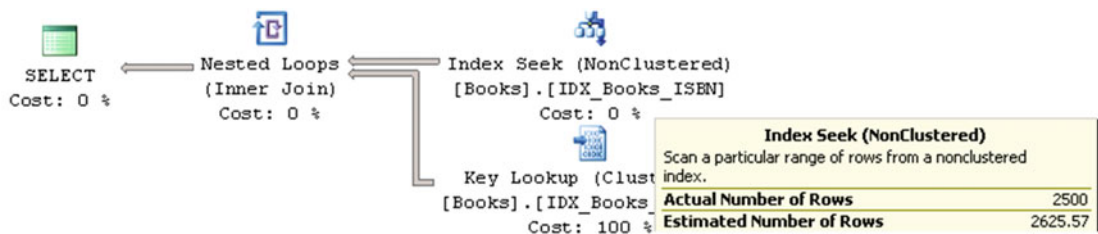
Figure 3-3. Execution plan of the query
