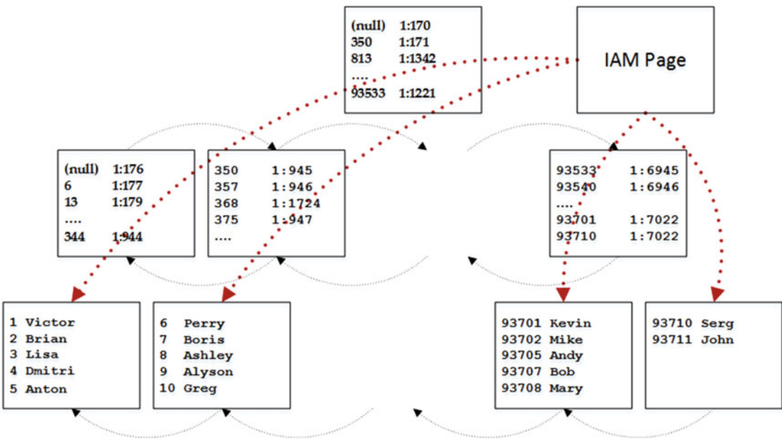
Figure 2-10. Allocation order scan
