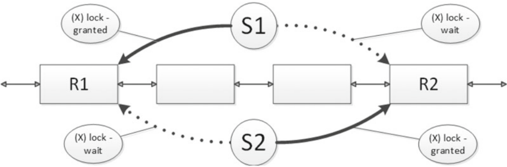
Figure 19-2. Classic deadlock, step 2
