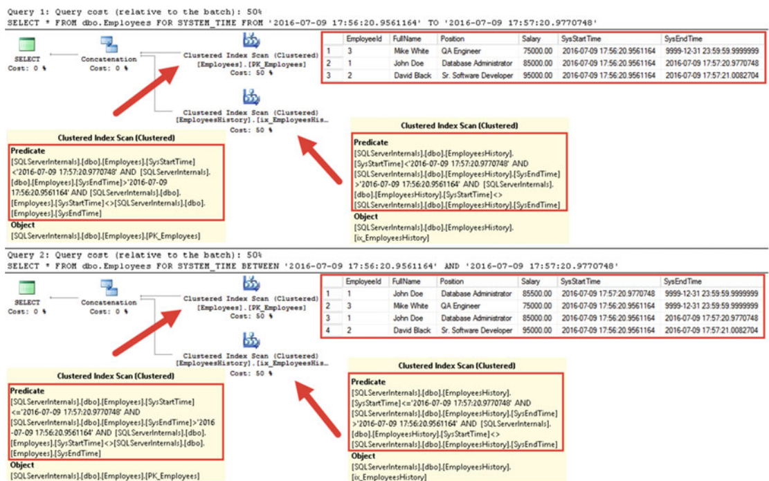
Figure 5-6. Querying temporal table: FOR SYSTEM_TIME FROM and FOR SYSTEM_TIME BETWEEN
