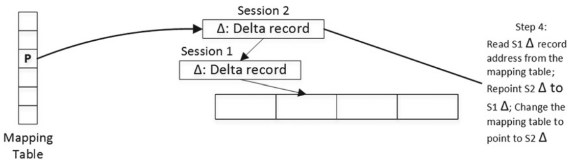
Figure 35-10. Data modifications and concurrency: Final steps
