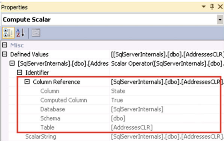
Figure 15-5. UDT performance: Computer scalar operator with calculated column
