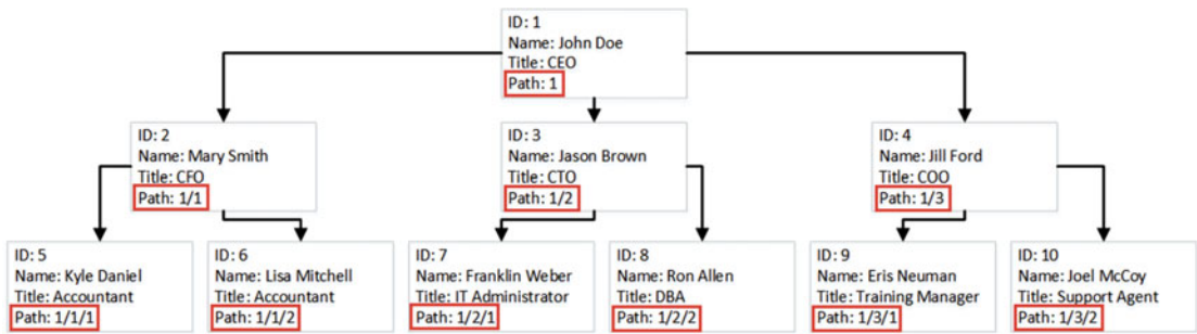
Figure 15-14. Materialized (hierarchical) path
