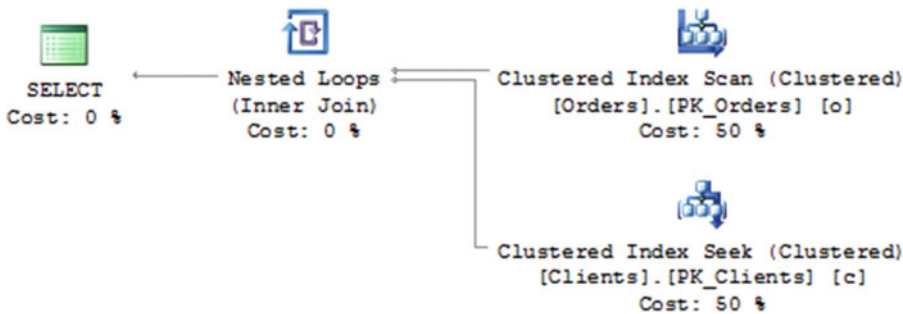
Figure 11-1. Execution plan of the dbo.usp_Orders_GetActiveOrders stored procedure
