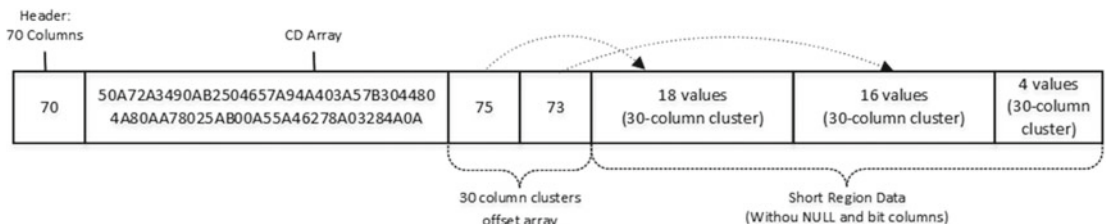
Figure 4-16. Example of CD and Short Data Regions data
