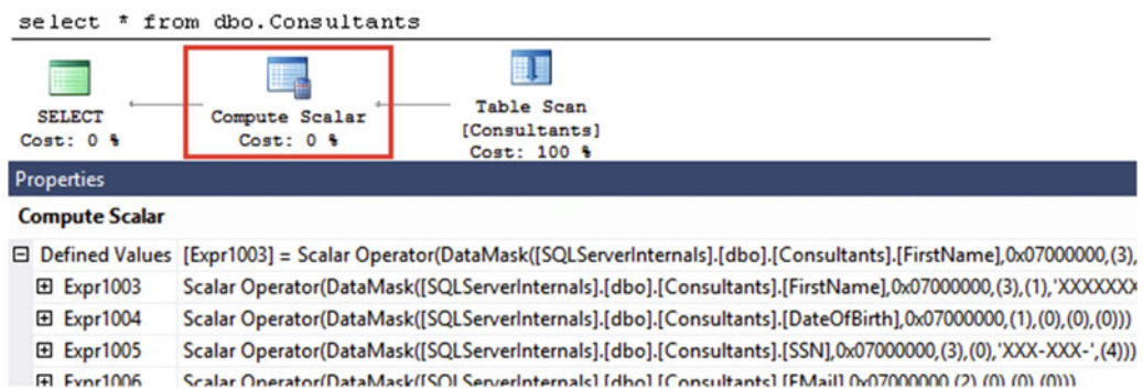
Figure 5-22. Execution plan of the query with dynamic data masking
