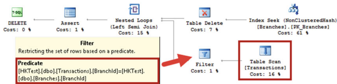
Figure 36-8. Referential integrity validation: Execution plan of DELETE statement
