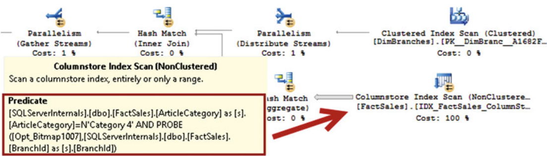
Figure 33-25. Execution plan for a query that uses a string attribute in the facts table to filter the article category (SQL Server 2016)
