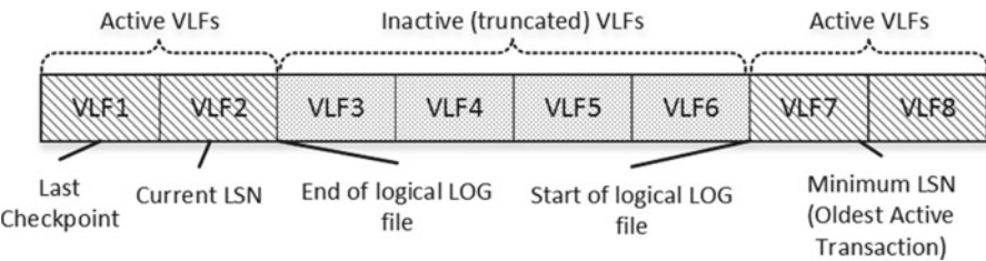
Figure 30-9. A transaction log is a wraparound file
