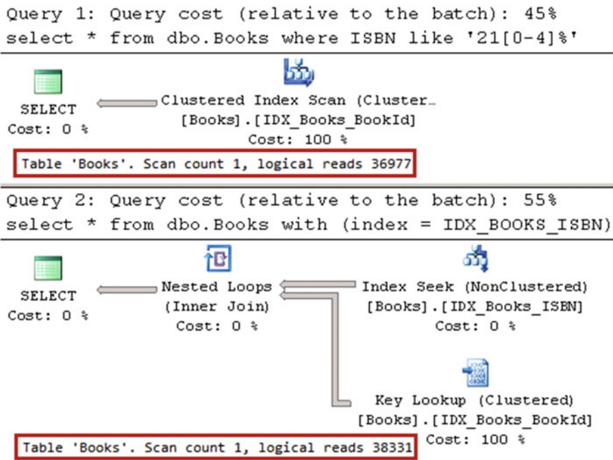
Figure 2-21. Selecting data for five prefixes: Execution plans
