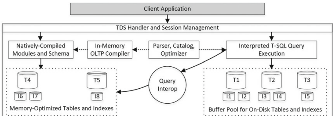
Figure 35-1. SQL Server Engine architecture
