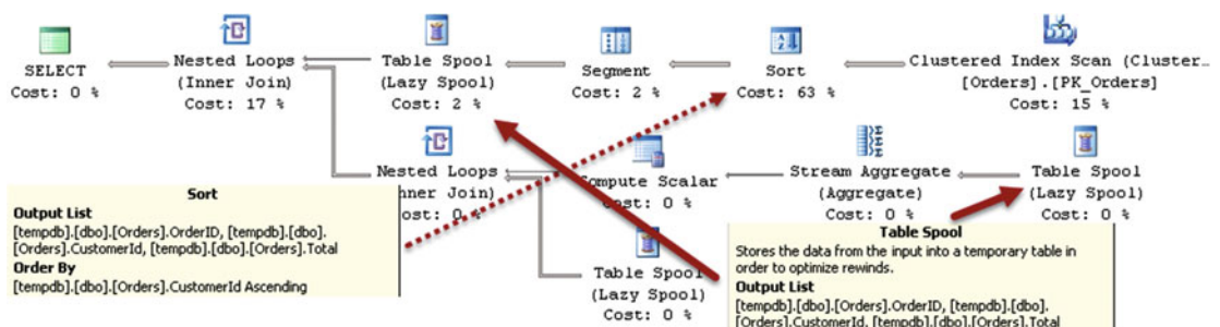
Figure 25-11. Execution plan of the query
