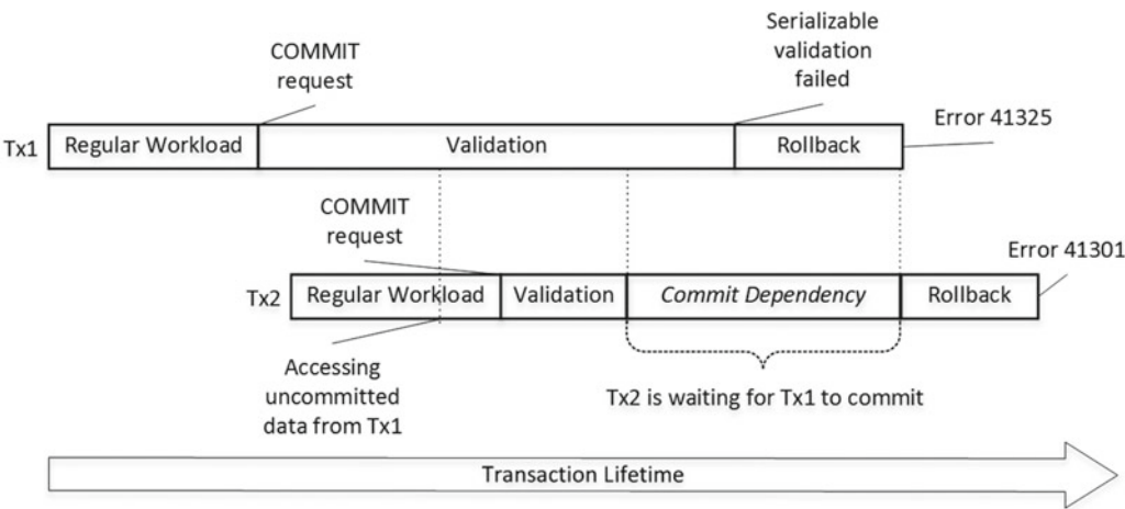
Figure 36-6. Commit dependency: Validation error
