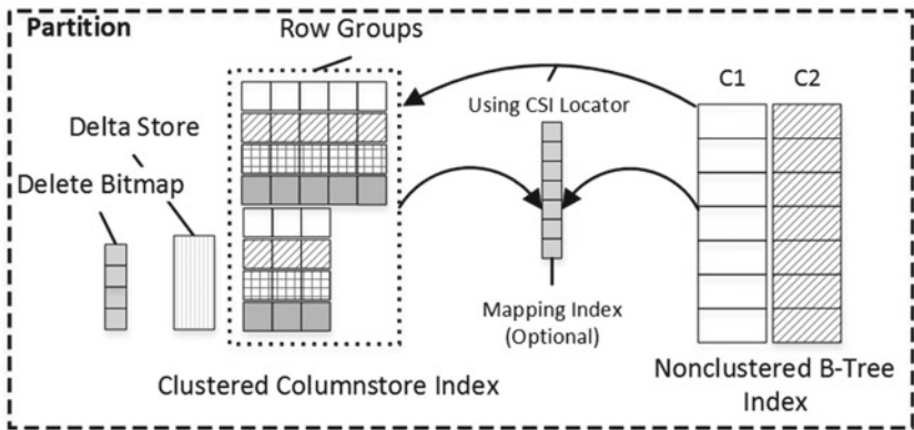
Figure 34-12. Partition of the table with clustered columnstore and nonclustered B-Tree indexes
