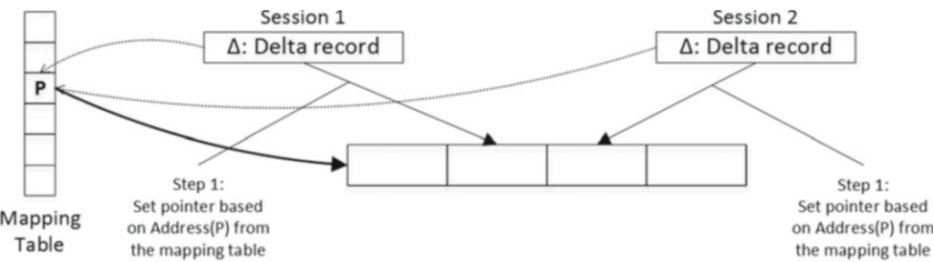
Figure 35-8. Data modifications and concurrency: Step 1
