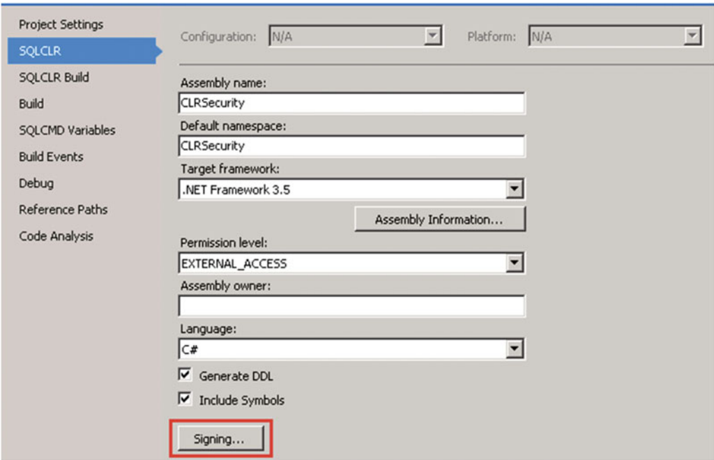
Figure 14-3. Signing CLR project: Step 1
