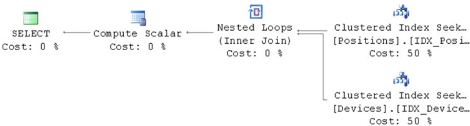
Figure 10-5. Execution plan with multi-column foreign key constraints
