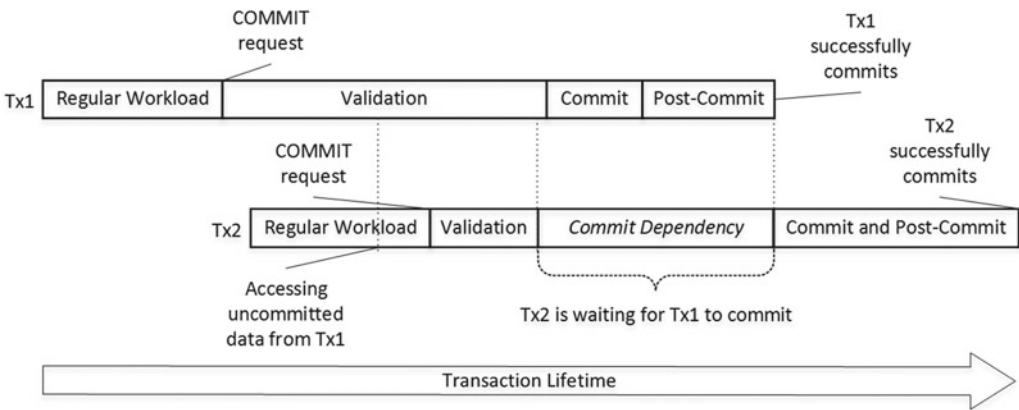
Figure 36-5. Commit dependency: Successful commit
