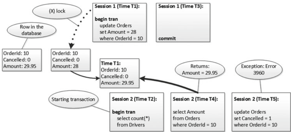
Figure 21-6. Snapshot isolation level and writer's behavior (2)
