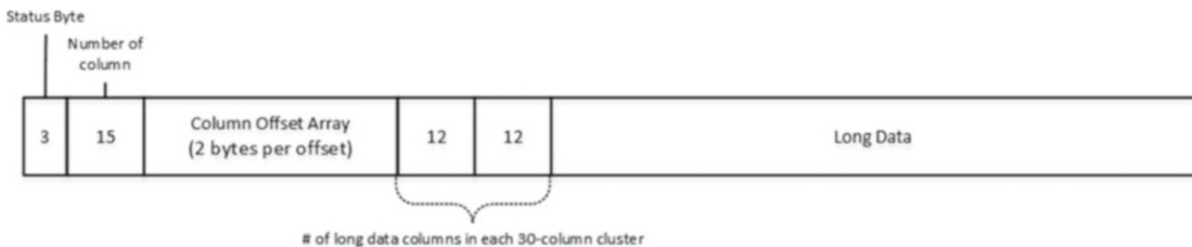
Figure 4-17. Example of Long Data Region data
