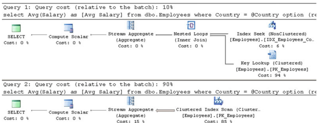
Figure 26-3. Parameter sniffing: Statement-level recompile
