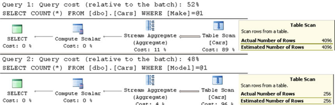
Figure 4-9. Cardinality estimations with a single predicate
