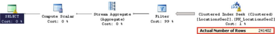
Figure 15-7. Customer-based POI lookup: Execution plan for the first query
