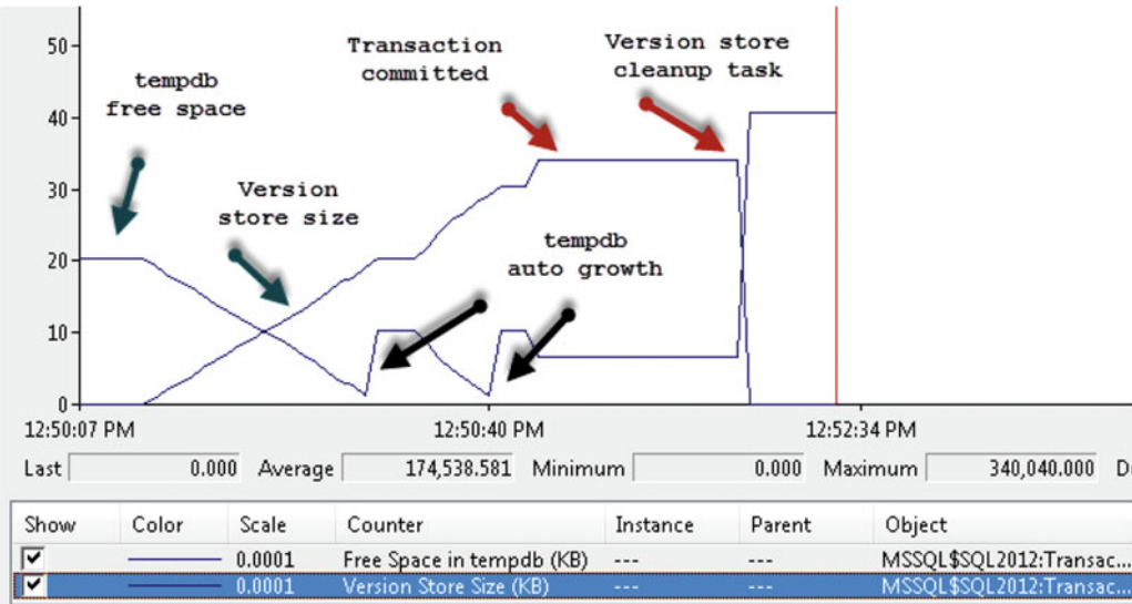
Figure 21-11. Tempdb free space and version store size
