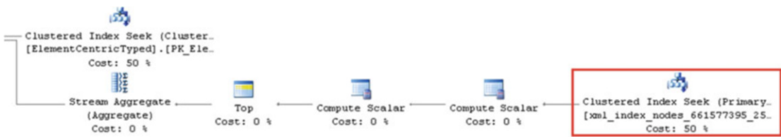
Figure 12-6. Execution plan when the XML index is present
