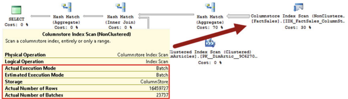
Figure 33-10. Execution plan with a columnstore index scan and MAXDOP=1 in SQL Server 2016 with compatibility level of 130
