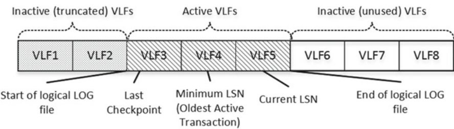
Figure 30-11. SIMPLE recovery model: Initial stage
