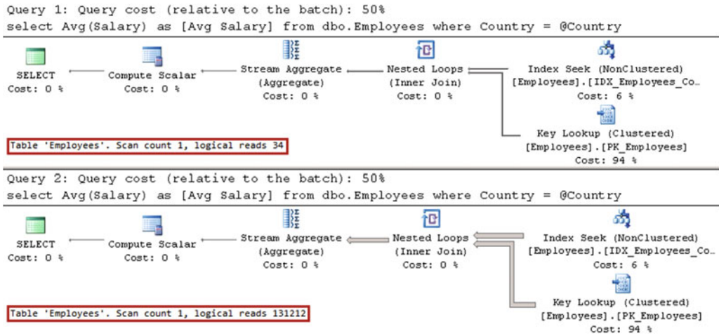
Figure 26-2. Parameter sniffing: Cached plan for @Country= 'Canada'
