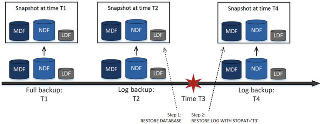
Figure 31-11. File snapshot point-in-time restore
