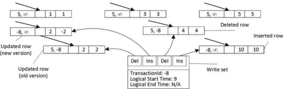
Figure 36-3. Data in the dbo.HKData table after modifications
