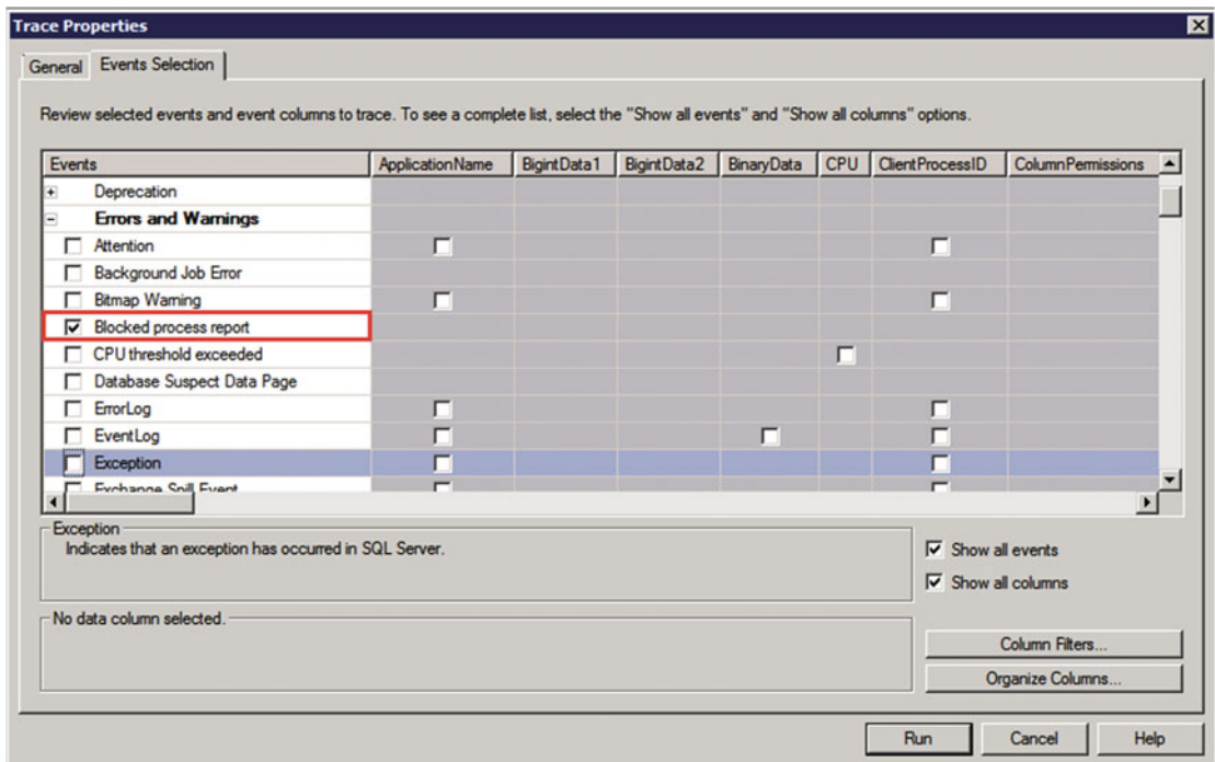
Figure 18-5. Blocked process report event in SQL Trace
