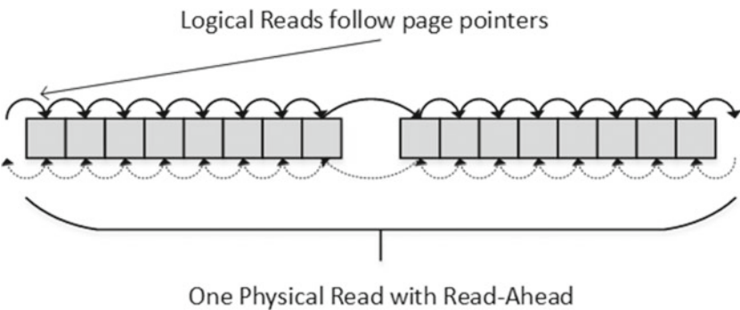
Figure 6-1. Logical and physical reads
