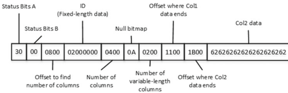
Figure 1-10. Second data row data
