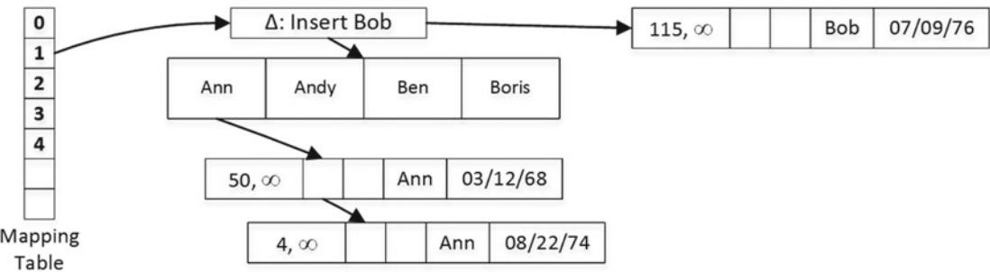
Figure 35-11. Leaf-level index page with an inserted delta record
