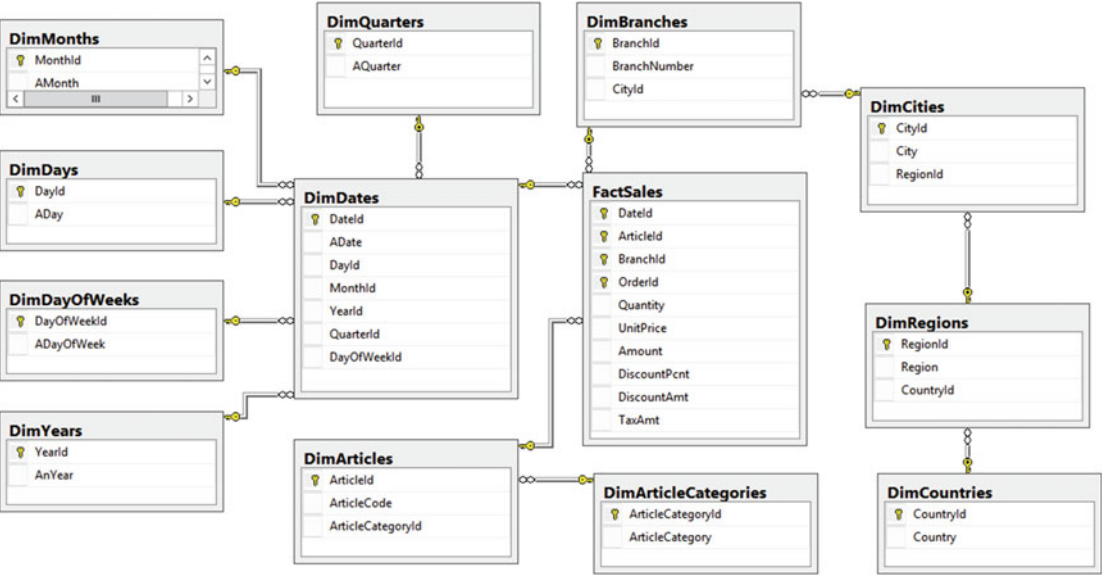
Figure 33-2. Snowflake schema
