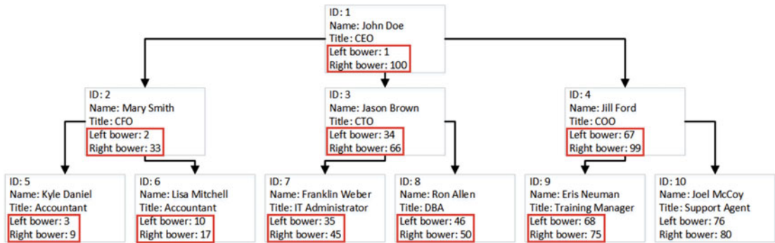
Figure 15-13. Nested sets
