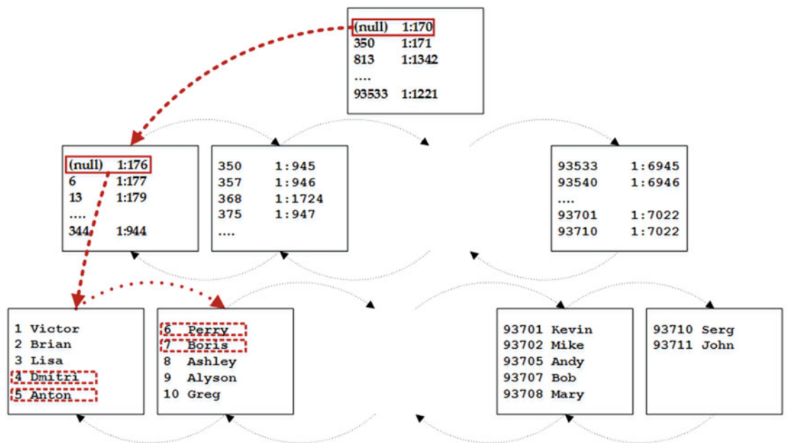
Figure 2-12. Index seek
