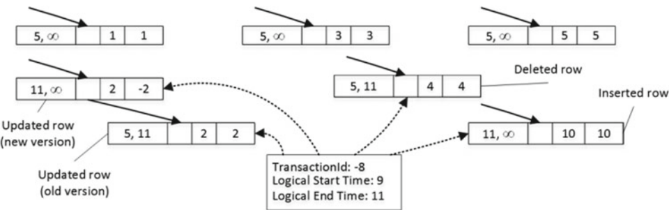
Figure 36-7. Completed transaction
