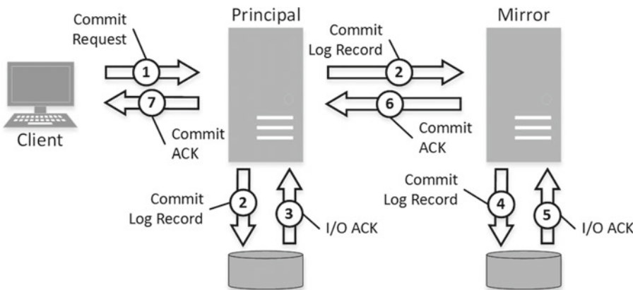
Figure 32-5. Synchronous commit
