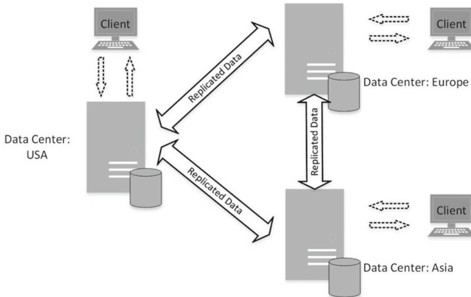
Figure 32-10. Peer-to-peer replication
