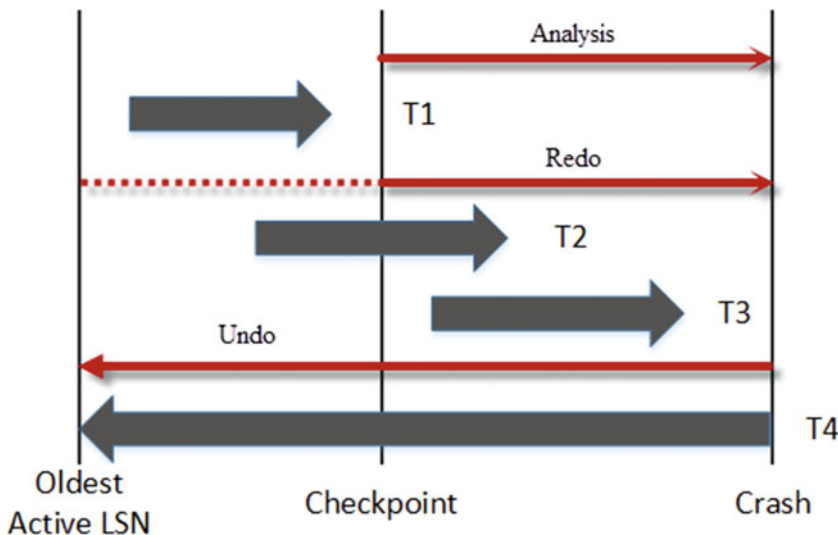
Figure 30-7. Database recovery
