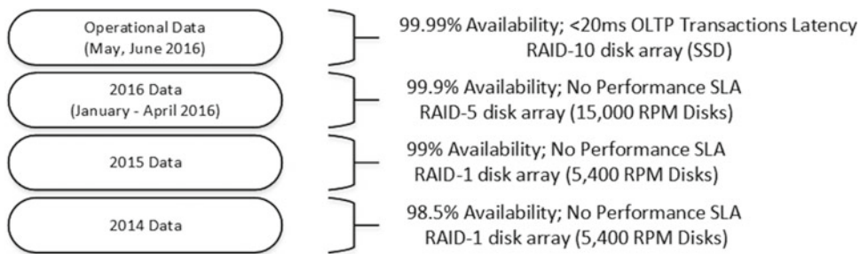
Figure 16-7. Tiered storage
