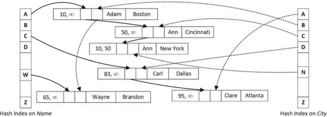
Figure 35-3. Hash indexes
