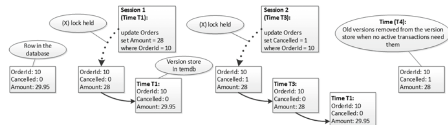
Figure 21-1. Version store
