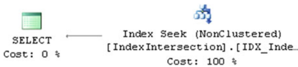
Figure 7-6. Multiple nonclustered indexes: Execution plan with covering index
