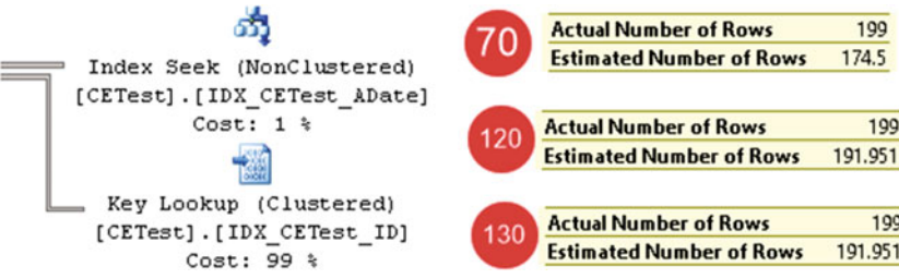
Figure 3-17. Outdated statistics: Cardinality estimations for a value that is not a key in the histogram step
