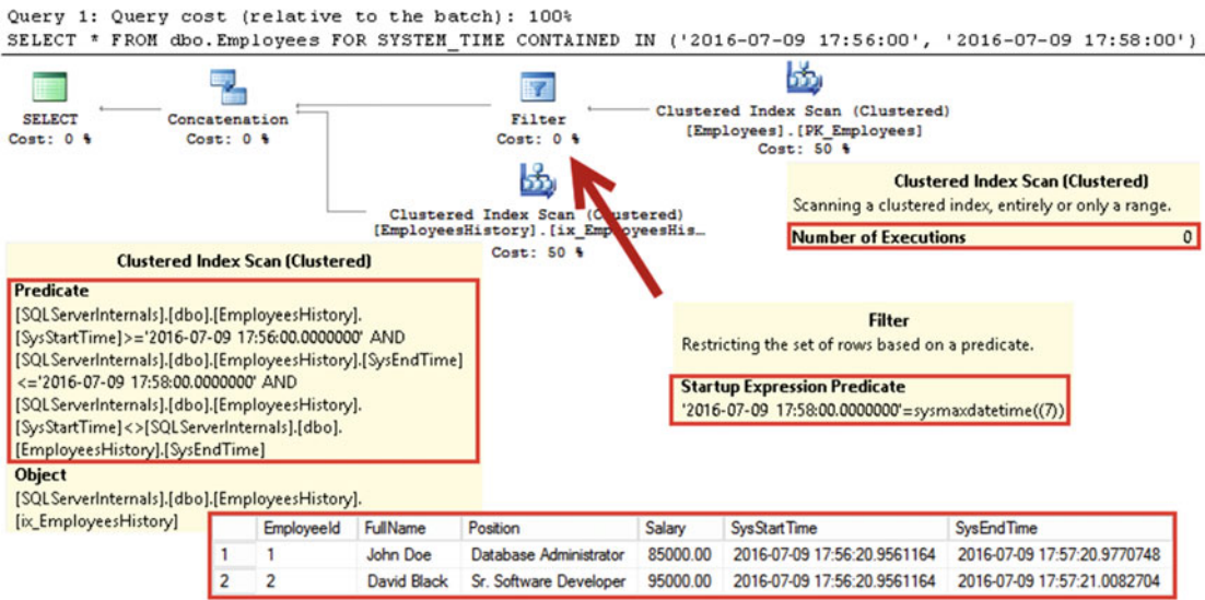
Figure 5-7. Querying temporal table: FOR SYSTEM_TIME CONTAINED IN
