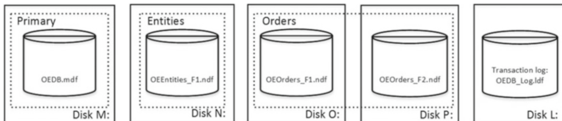
Figure 1-1. Physical layout of the database and data files
