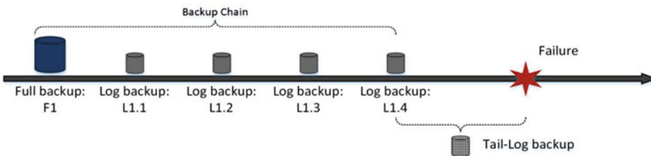
Figure 31-1. Backup chain and tail-log backup
