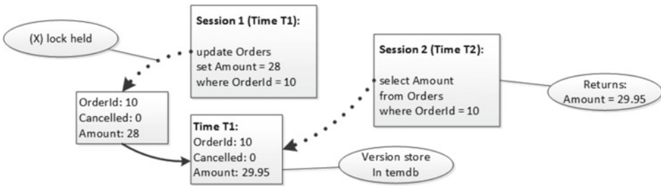
Figure 21-2. Readers and version store
