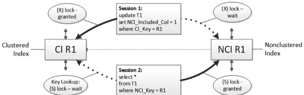
Figure 19-7. Key lookup deadlock, step 2
