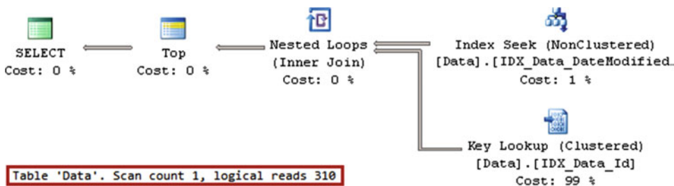
Figure 16-13. Execution plan with non-partitioned table
