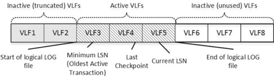
Figure 30-8. Transaction log and virtual log files
