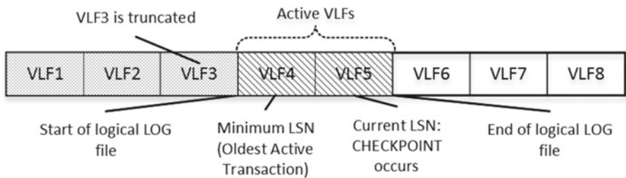
Figure 30-12. SIMPLE recovery model: Log truncation after CHECKPOINT
