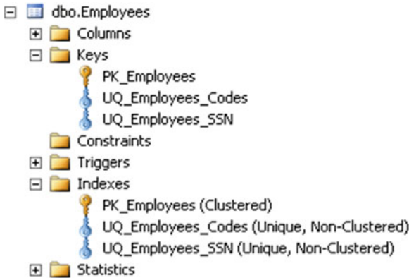
Figure 8-1. Unique constraints in SQL Server Management Studio
