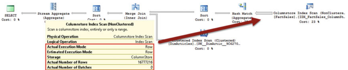
Figure 33-11. Execution plan with a columnstore index scan and MAXDOP=1 in SQL Server 2016 with compatibility level less than 130
