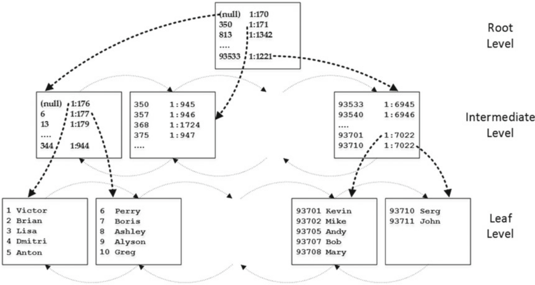
Figure 2-7. Clustered index structure: Root level
