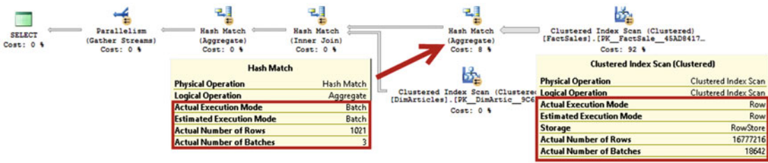
Figure 33-13. Execution plan with clustered index scan in SQL Server 2014 and SQL Server 2016 with a database compatibility level of less than 130
