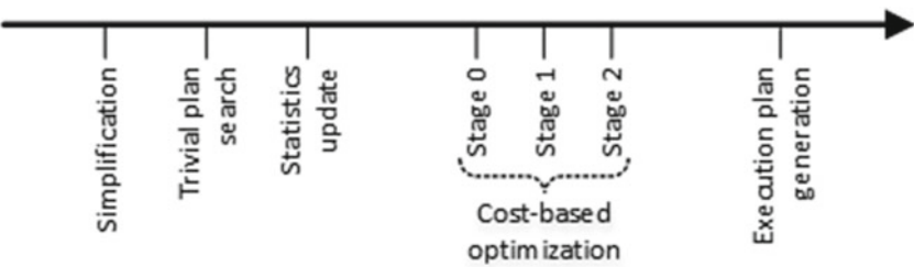
Figure 25-2. Query optimization phases
