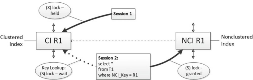
Figure 19-9. Deadlock due to multiple updates of the same row, step 2
