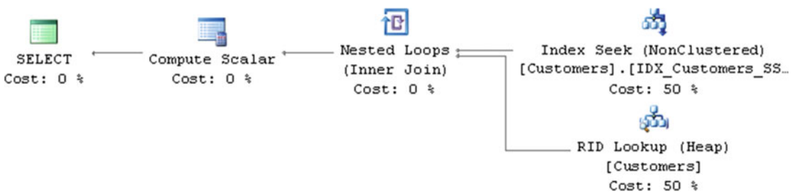
Figure 4-14. Execution plan that utilizes a nonclustered index on a non-persisted calculated column
