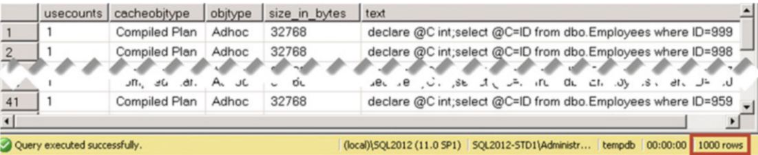
Figure 26-9. Plan cache content after query execution
