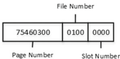
Figure 1-12. Row-overflow data: Row-overflow page pointer structure
