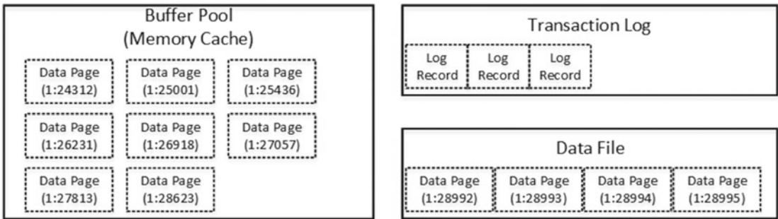
Figure 1-17. Data modification: Initial stage
