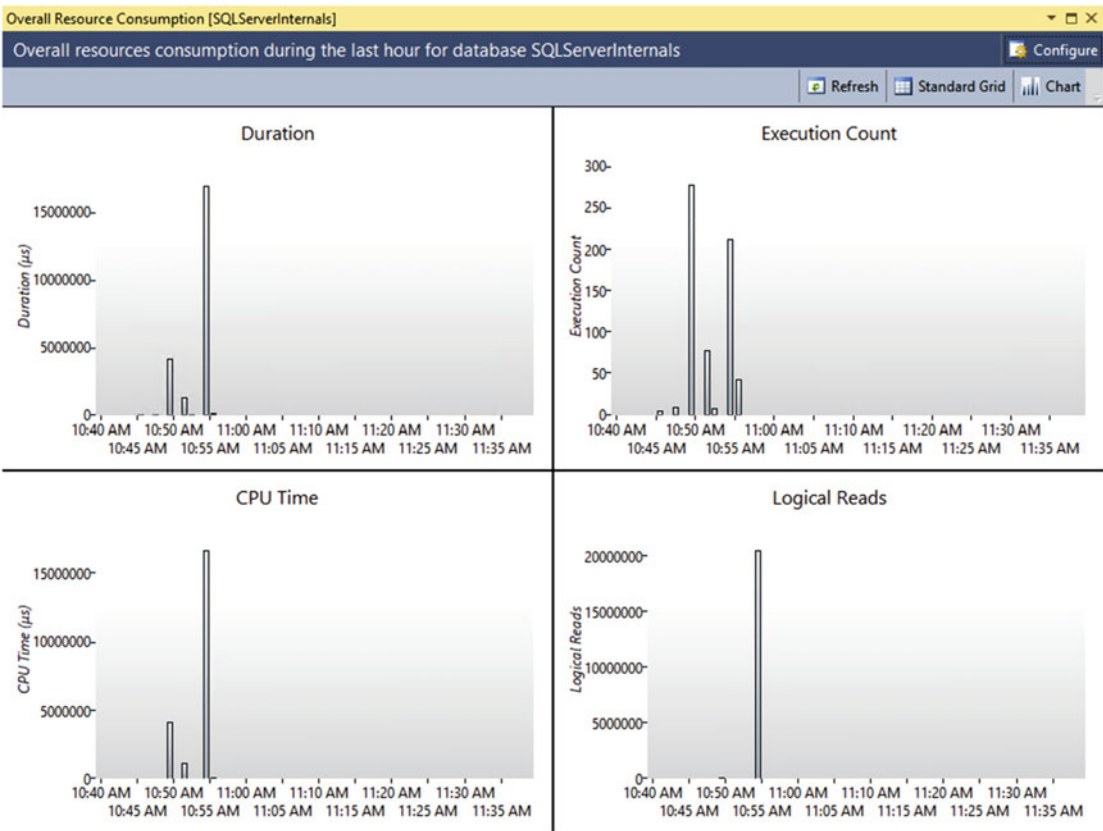
Figure 29-8. Overall Resource Consumption report
