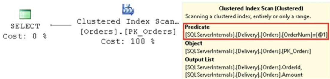
Figure 18-4. Execution plan for the blocked query
