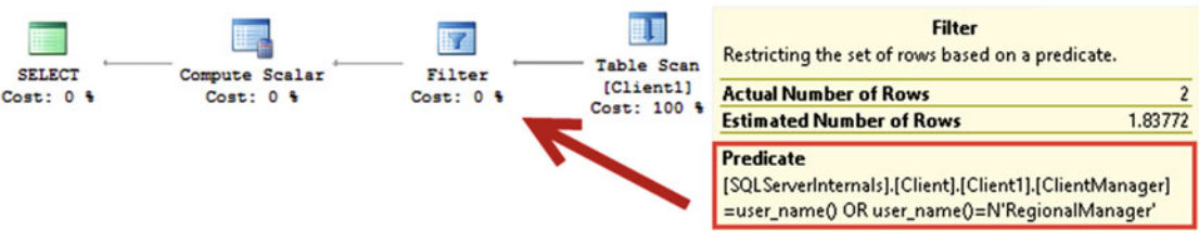
Figure 5-16. Execution plan with row-level security applied
