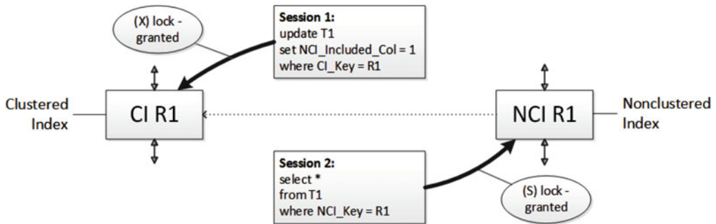
Figure 19-6. Key lookup deadlock, step 1
