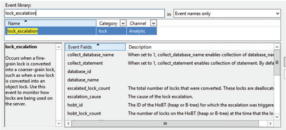
Figure 20-4. Lock_escalation Extended Event
