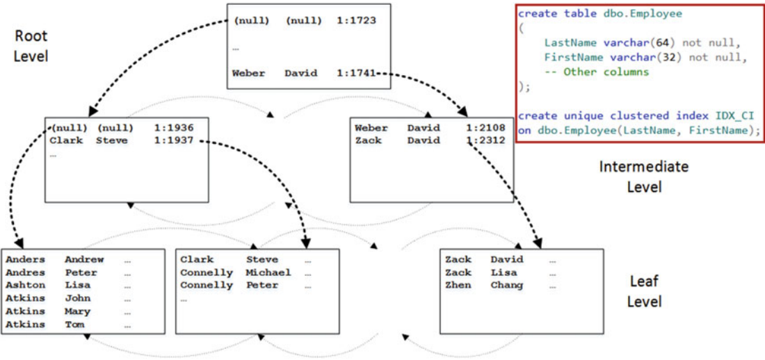
Figure 2-16. Composite index structure
