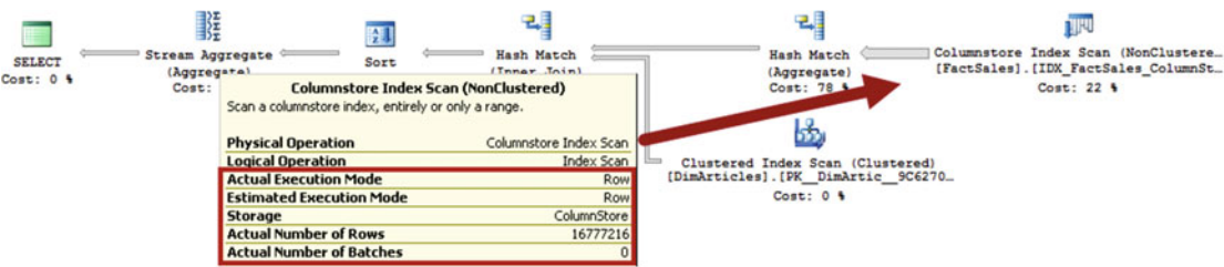
Figure 33-9. Execution plan with a columnstore index scan and MAXDOP=1 (SQL Server 2012 and 2014)
