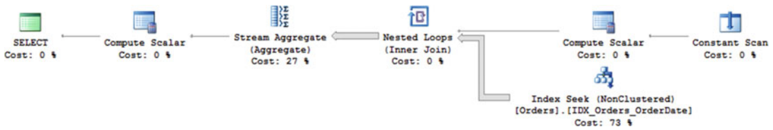
Figure 5-13. Execution plan: Predicate on OrderDate column
