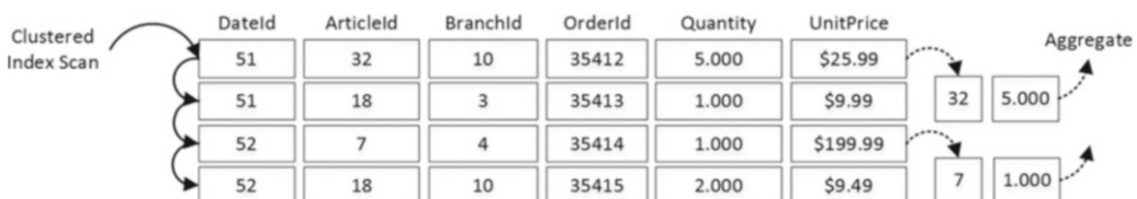
Figure 33-4. Row mode execution
