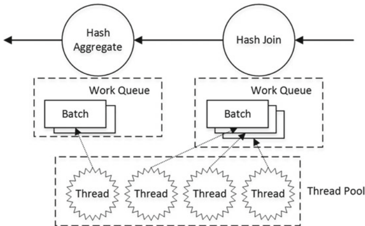
Figure 33-7. Parallelism in batch mode execution
