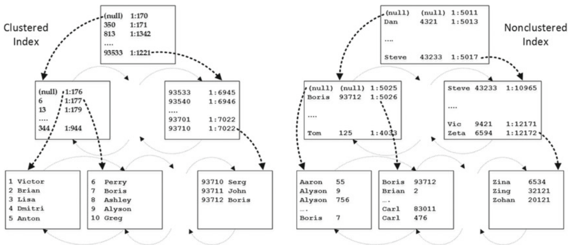
Figure 2-17. Clustered and nonclustered index structures
