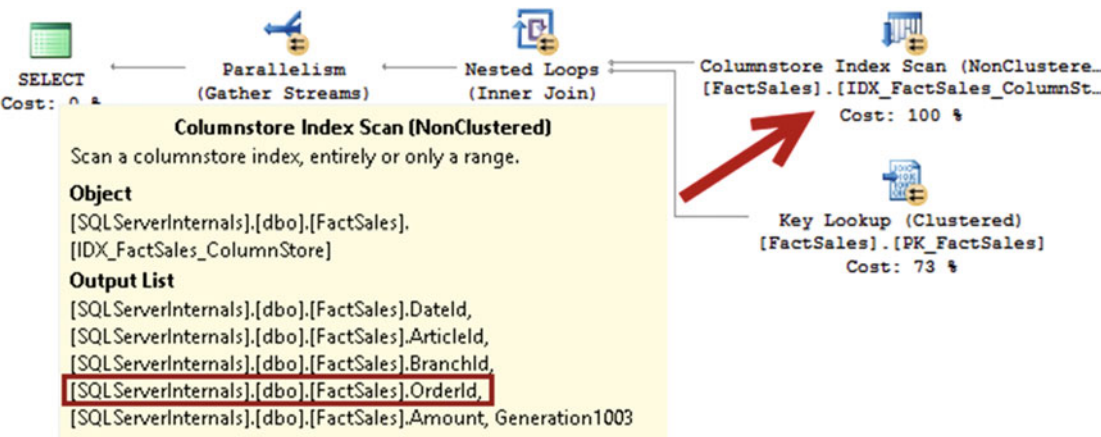
Figure 34-1. Execution plan for this query
