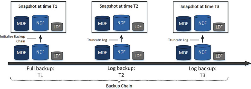
Figure 31-10. File snapshot backups
