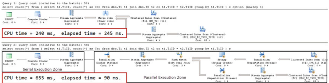
Figure 25-14. Parallel execution: Query plans
