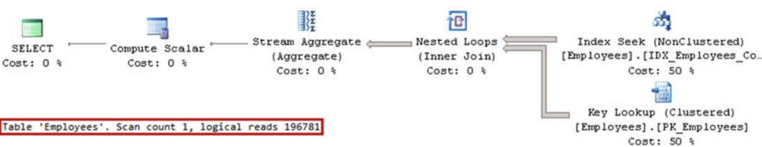
Figure 26-5. Parameter sniffing: OPTIMIZE FOR and data-distribution change
