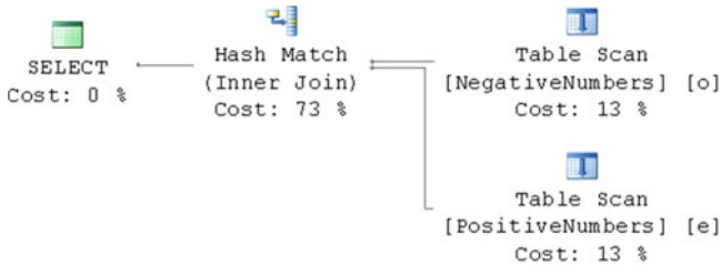
Figure 8-7. Execution plan without check constraints
