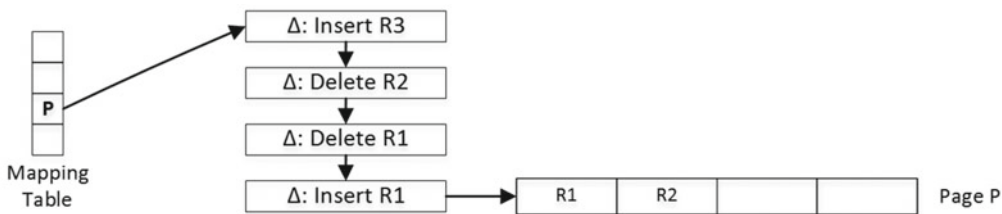
Figure 35-7. Delta records and nonclustered index leaf page
