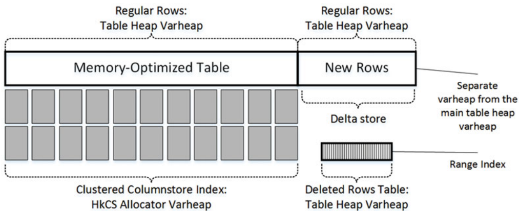
Figure 35-23. Clustered columnstore index on memory-optimized table
