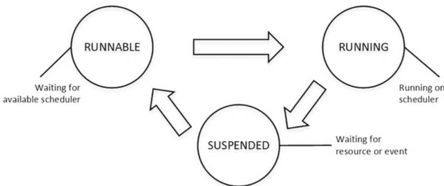
Figure 28-3. Task life cycle
