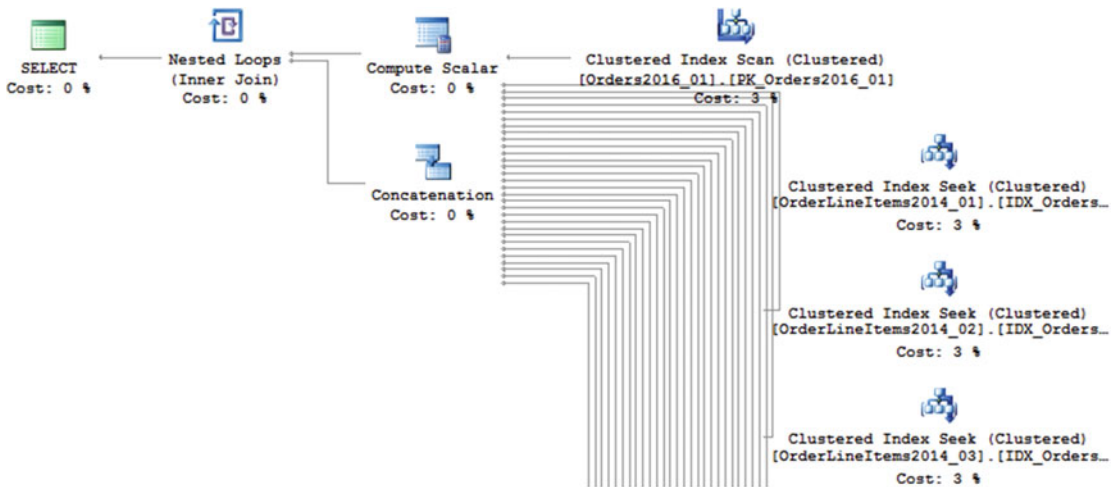
Figure 16-4. Execution plan of a non-optimized query
