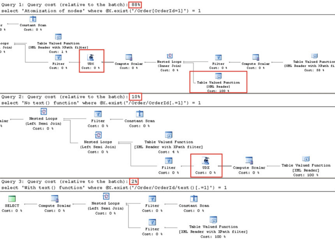
Figure 12-9. Atomization of nodes and type casting
