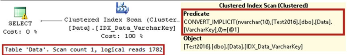
Figure 2-15. SARG predicates and data types: Execution plans with string parameter
