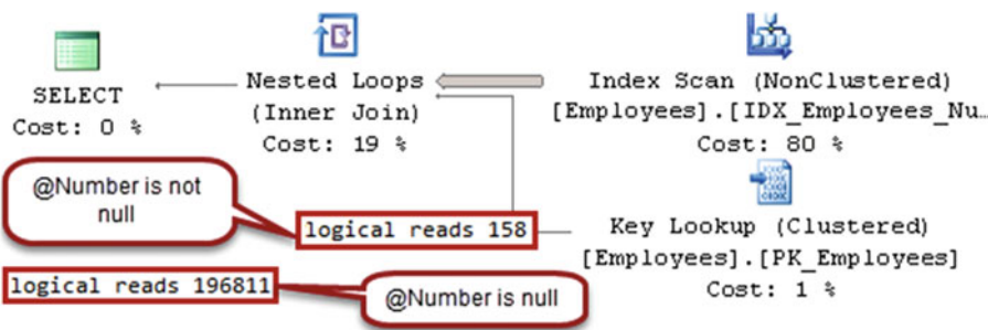
Figure 26-7. Plan reuse: Execution plans for the stored procedure calls
