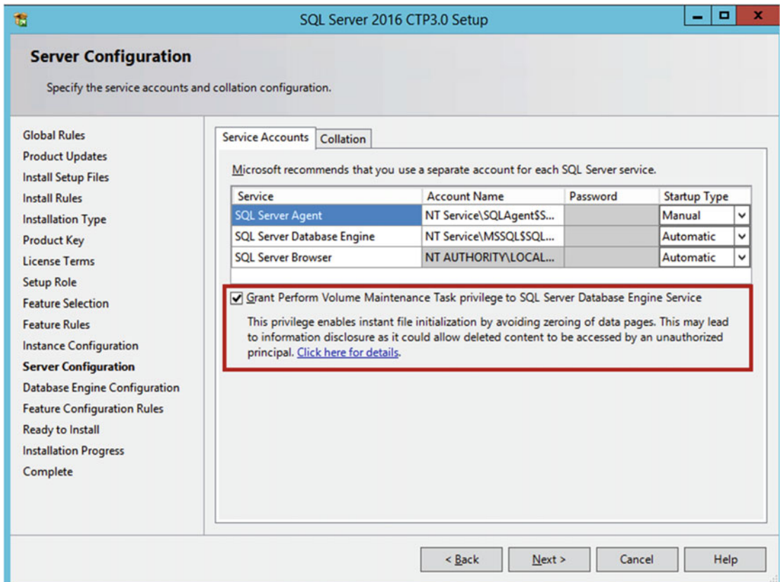
Figure 1-4. Enabling Instant File Initialization in SQL Server 2016 setup
