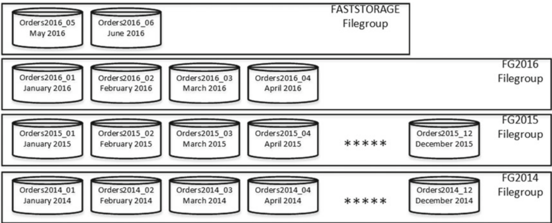
Figure 16-2. Data layout with a partitioned-view approach
