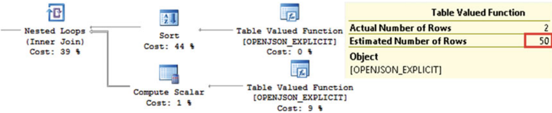
Figure 12-14. OPENJSON: Execution plan of the query
