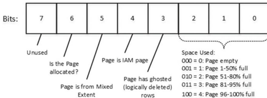
Figure 1-16. Page status byte in PFS page
