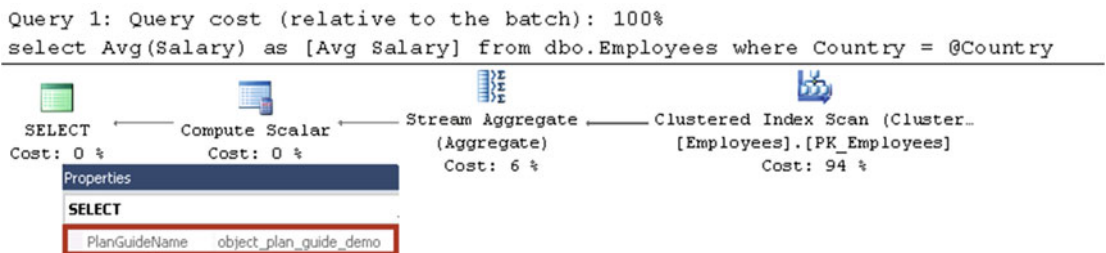
Figure 26-12. Execution plan with Object plan guide
