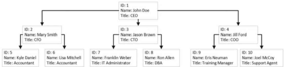
Figure 15-12. Closure table
