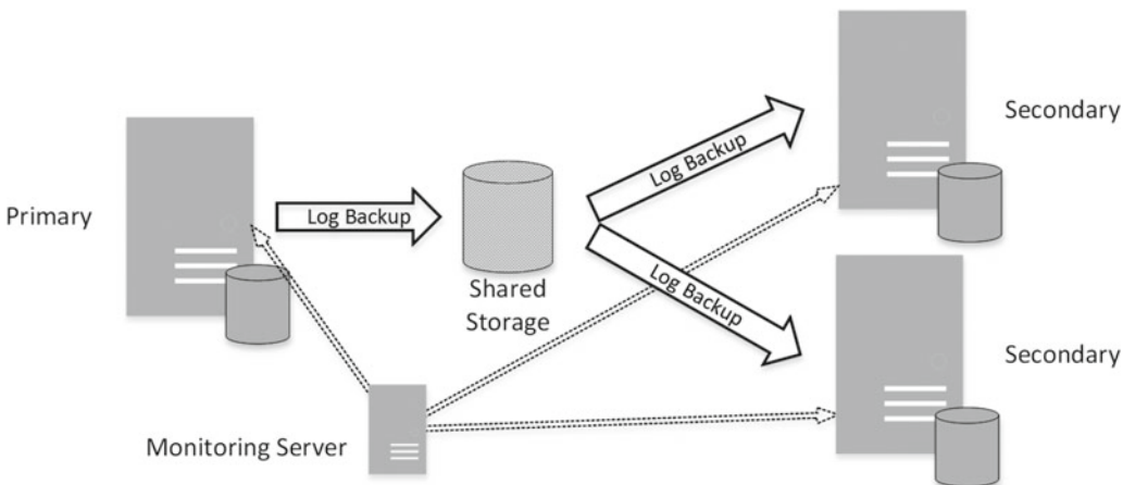
Figure 32-8. Log shipping
