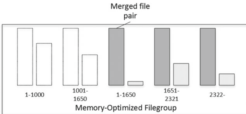
Figure 35-29. Merge process
