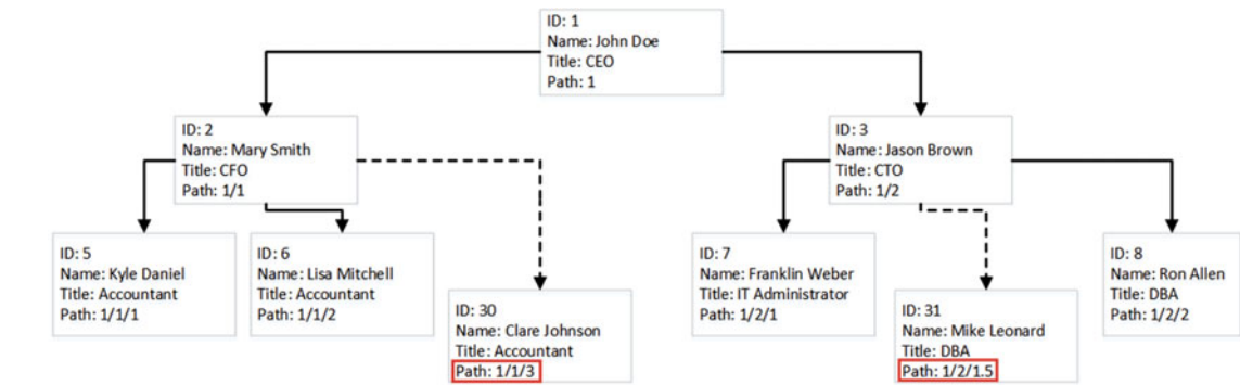
Figure 15-15. Inserting data
