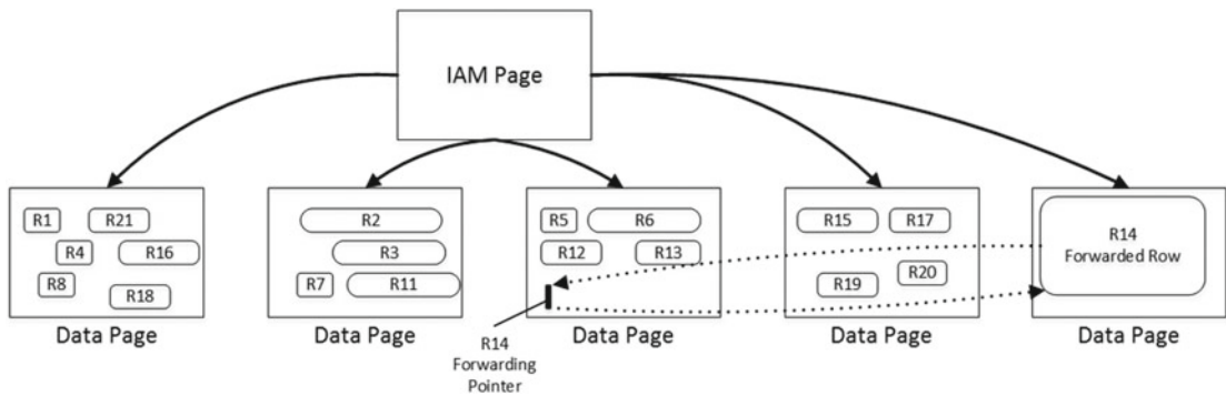
Figure 2-2. Forwarding pointers
