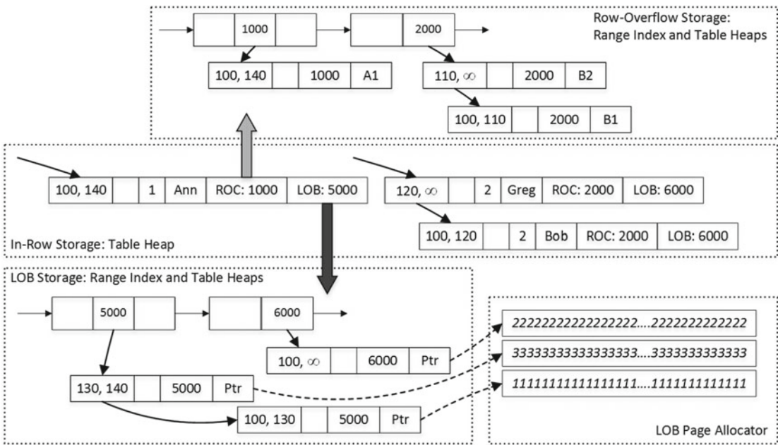
Figure 35-22. In-row and off-row storage
