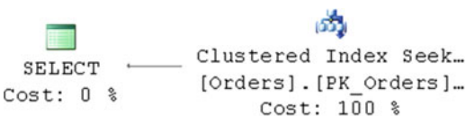
Figure 10-3. Execution plan with left outer join
