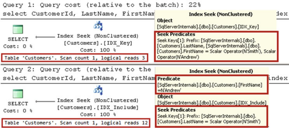
Figure 4-6. Included versus key columns: Selecting by LastName and FirstName
