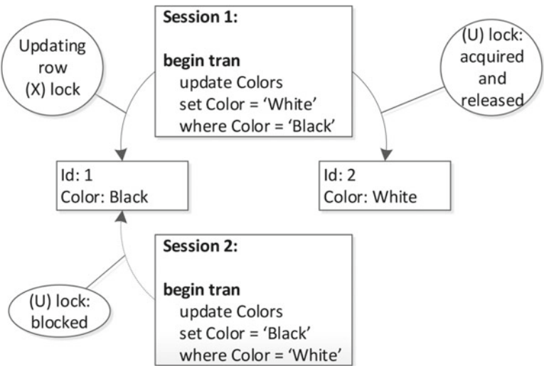
Figure 21-8. Pessimistic locking behavior: Step 1
