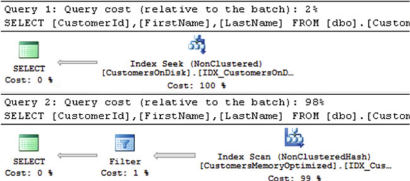
Figure 35-5. Composite hash index: Execution plans where queries use the leftmost index column only (SQL Server 2014)
