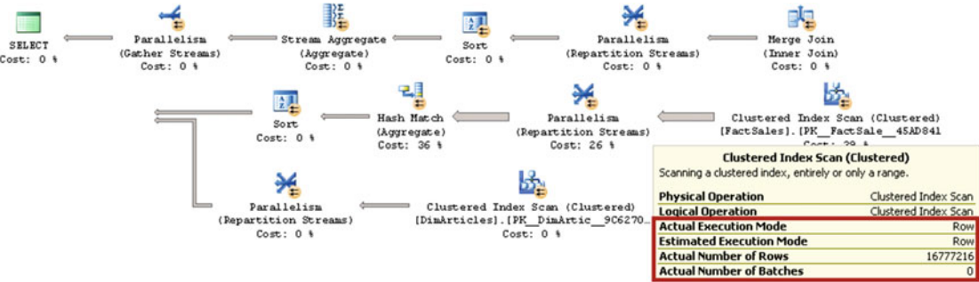
Figure 33-12. Execution plan with clustered index scan in SQL Server 2012
