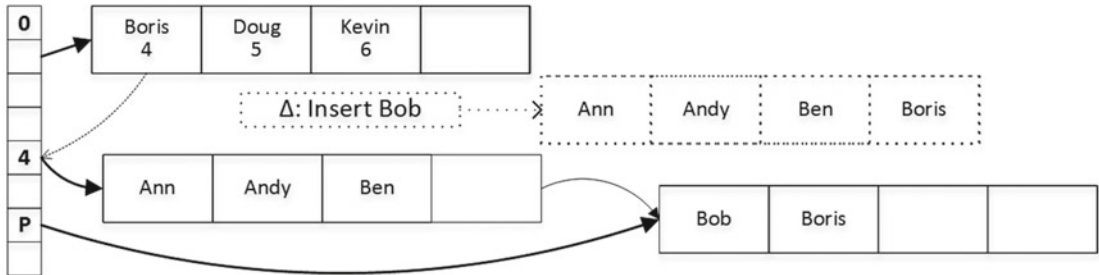
Figure 35-13. Page splitting: First step
