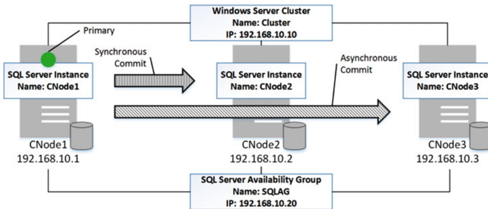
Figure 32-7. AlwaysOn Availability Group
