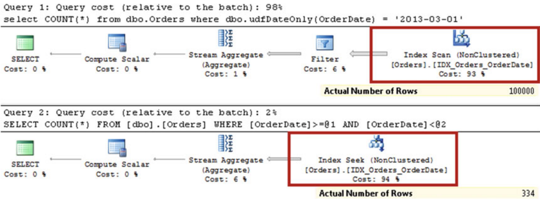
Figure 11-5. Execution plans of the queries with a non-clustered index on the OrderDate column
