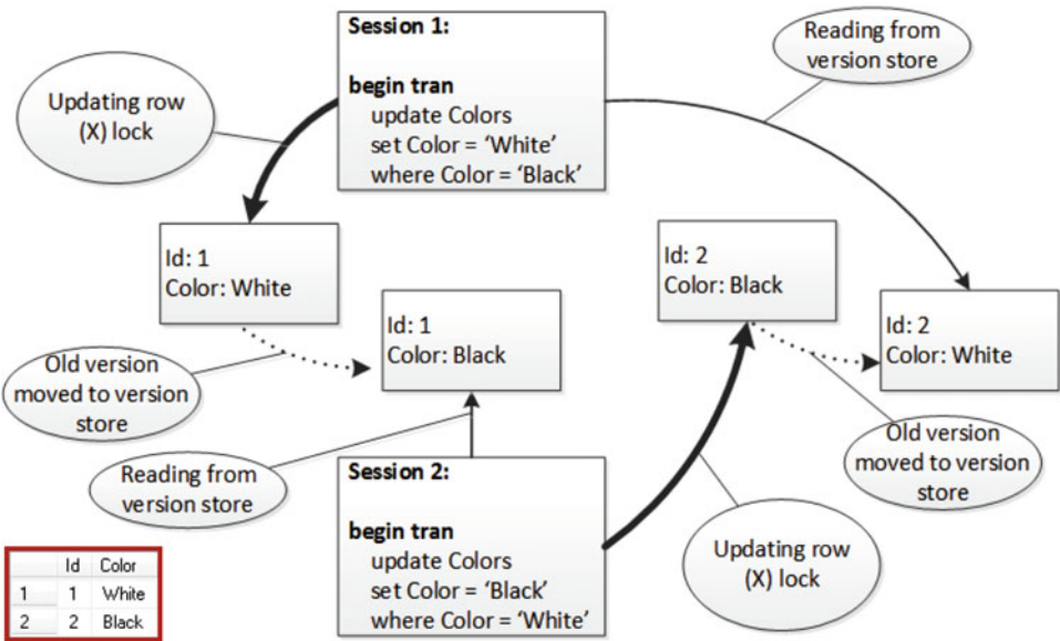
Figure 21-10. Snapshot isolation level locking behavior
