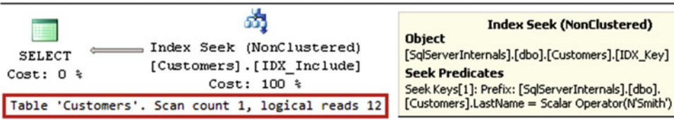
Figure 4-5. Included versus key columns: Selecting by LastName only
