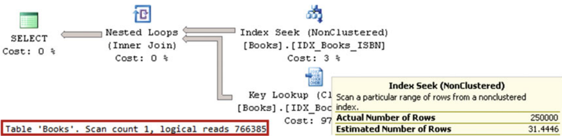
Figure 3-7. Execution plan for the query selecting rows with the 999 prefix
