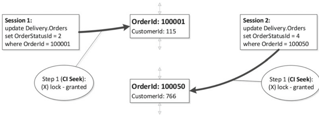
Figure 19-3. Deadlock due to scans, step 1
