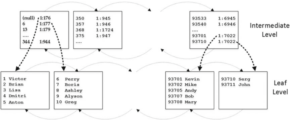
Figure 2-6. Clustered index structure: Intermediate and leaf levels
