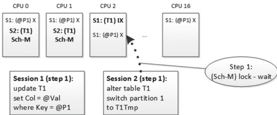
Figure 23-8. Deadlock due to lock partitioning: Step 1
