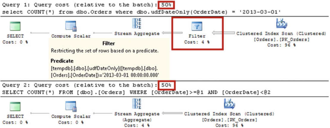
Figure 11-3. Execution plans with and without a scalar user-defined function
