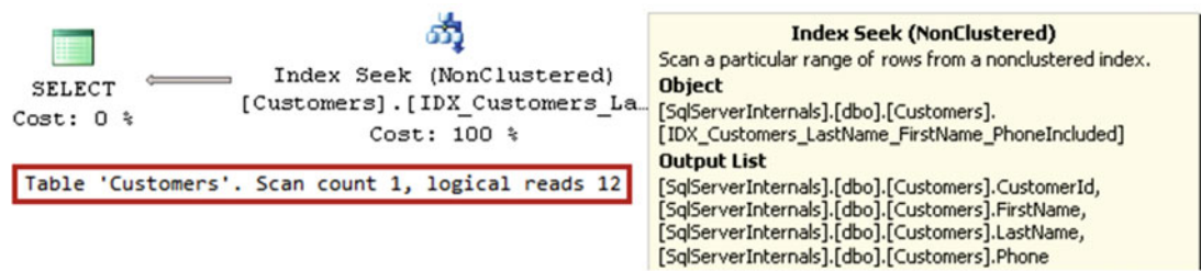
Figure 4-3. Execution plan with covering index
