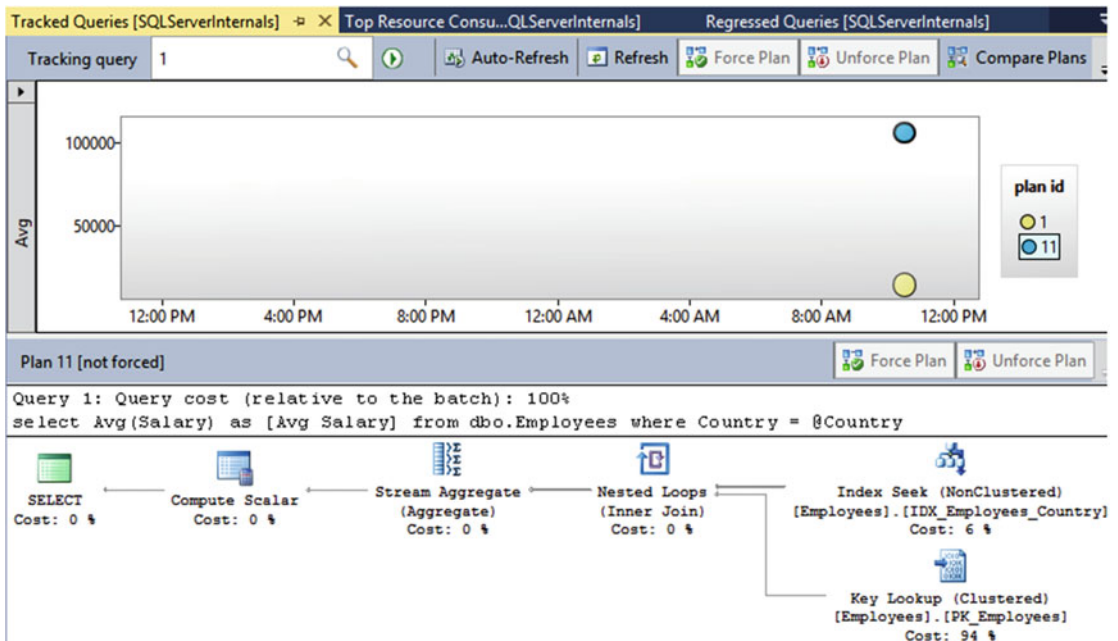
Figure 29-9. Tracked Queries report
