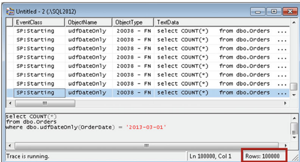
Figure 11-4. SQL trace with SP:Starting event
