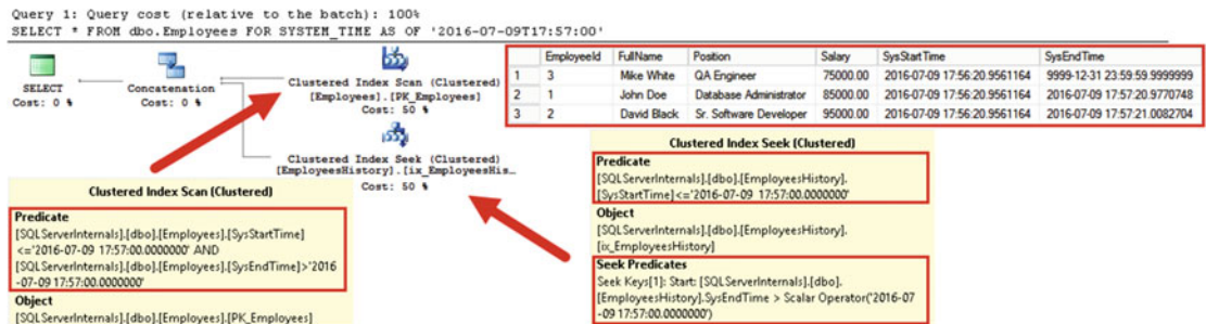
Figure 5-5. Querying temporal table: FOR SYSTEM_TIME AS OF
