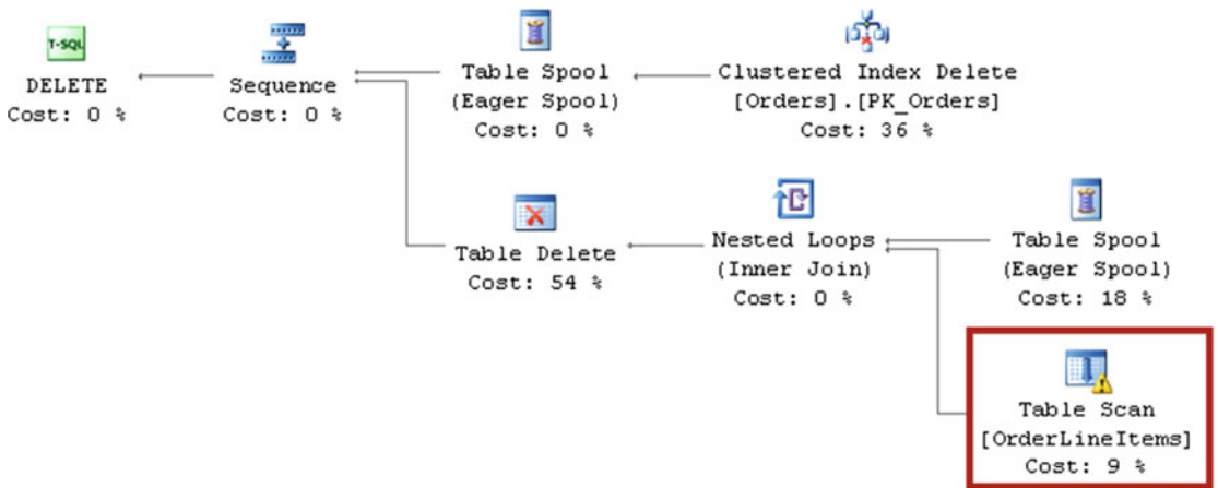
Figure 8-6. Deleting the row from the referenced table without an index specified on the referencing column
