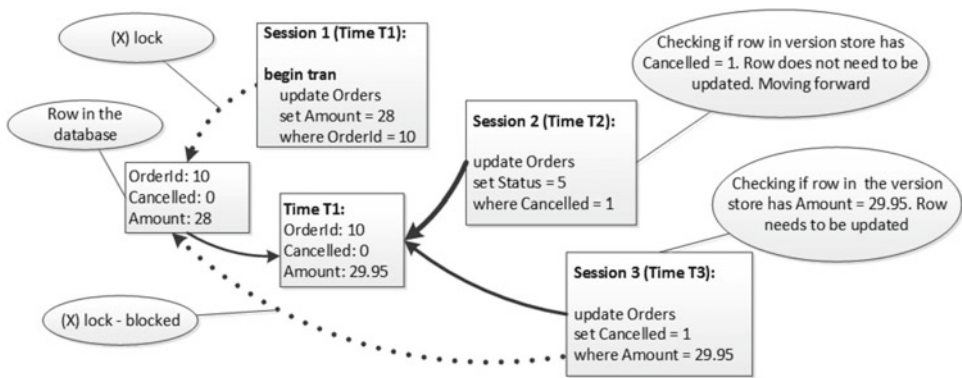
Figure 21-5. Snapshot isolation level and writer's behavior (1)
