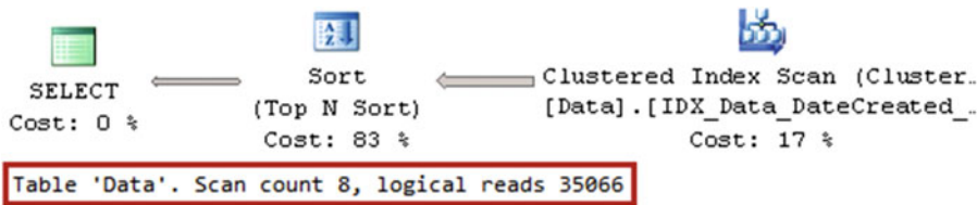
Figure 16-14. Execution plan with partitioned table
