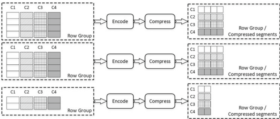
Figure 33-17. Building a columnstore index
