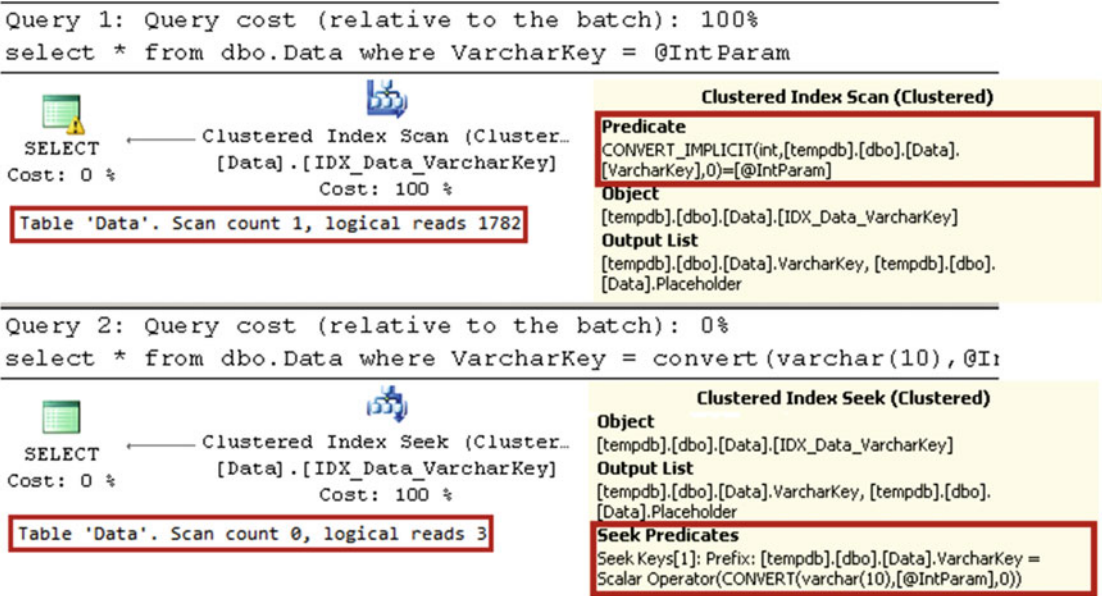
Figure 2-14. SARG predicates and data types: Execution plans with integer parameter
