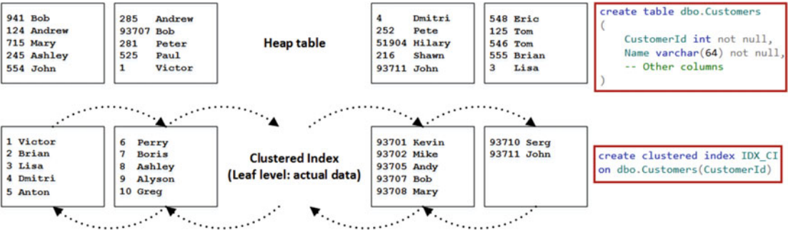
Figure 2-5. Clustered index structure: Leaf level
