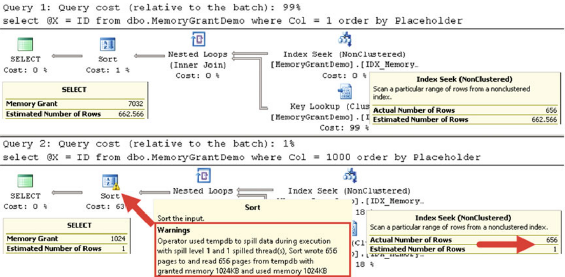
Figure 3-10. Cardinality estimation and memory grants: Execution plans
