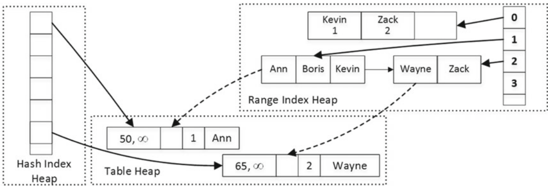
Figure 35-20. Table memory consumers
