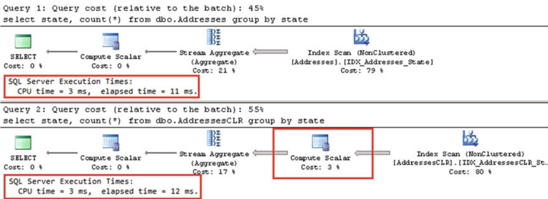
Figure 15-4. UDT performance: Persisted calculated column
