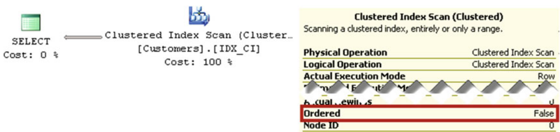
Figure 2-11. Allocation order scan execution plan
