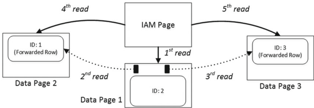
Figure 2-4. Forwarding pointers and I/O: Reading data when forwarding pointers exist
