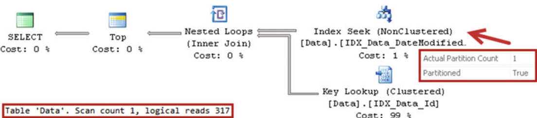
Figure 16-16. Execution plan for the query: Selecting data from a single partition
