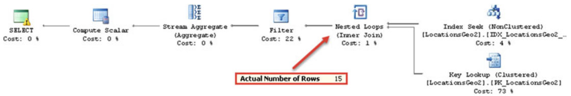
Figure 15-10. Customer-based POI lookup: Execution plan (bounding-box approach)
