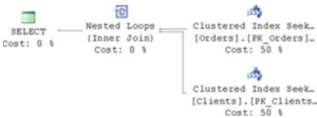
Figure 10-2. Execution plan when selecting columns that belong to the Orders table only
