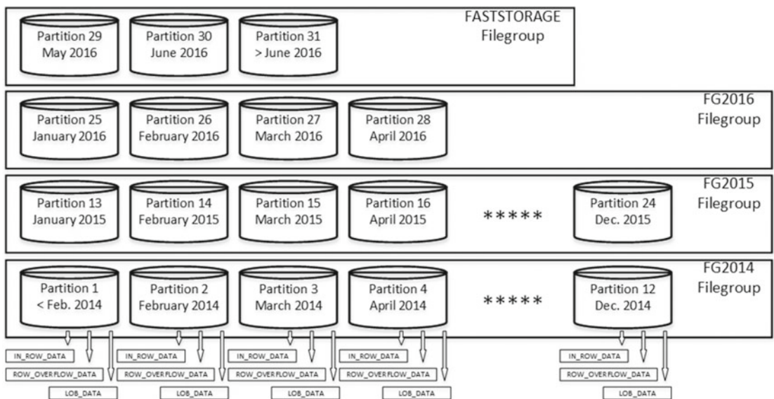
Figure 16-1. Data layout of the dbo.OrdersPT table
