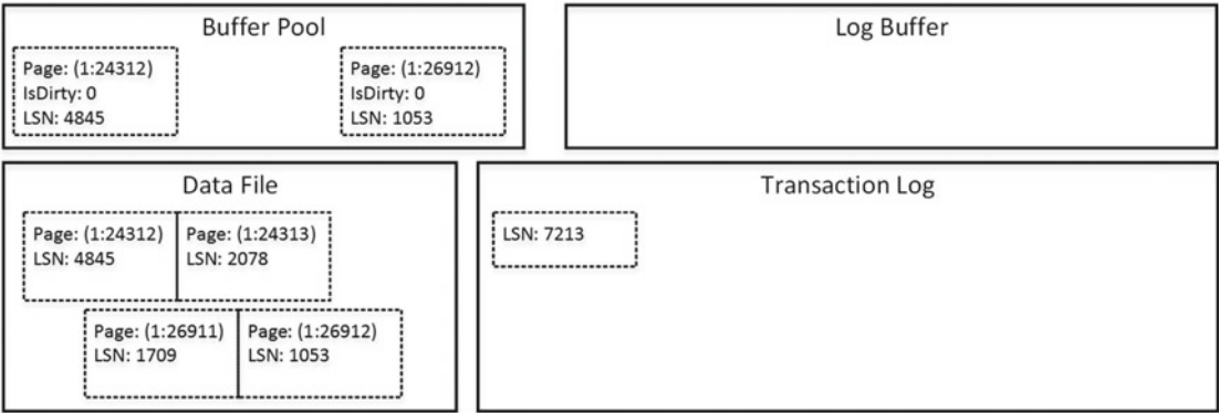
Figure 30-1. Data modifications: Initial state
