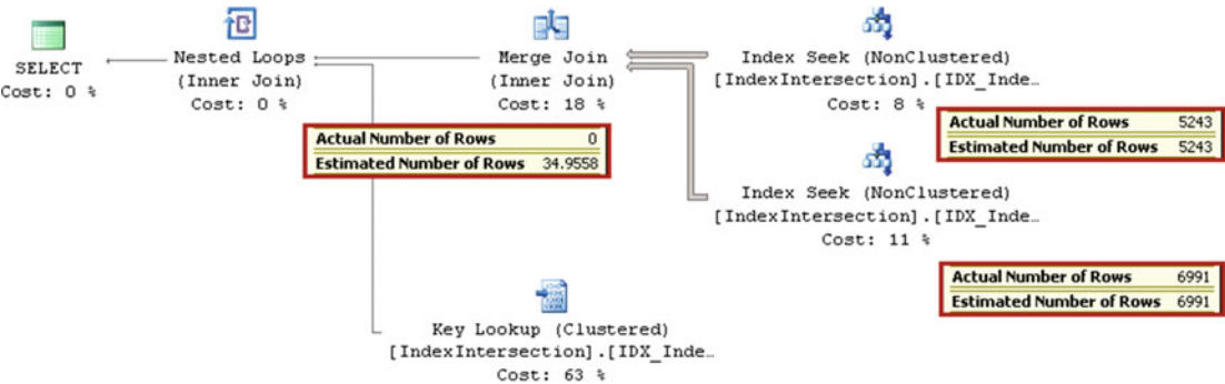
Figure 7-5. Multiple nonclustered indexes: Execution plan with index intersection
