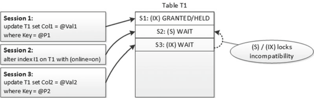
Figure 23-10. Blocking during the initial stage of an index rebuild
