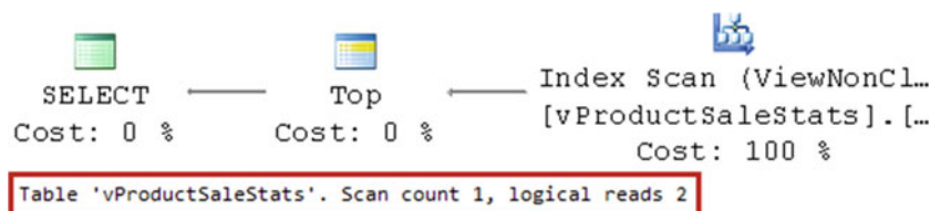
Figure 10-7. Execution plan of a query that selects the top 10 most popular products utilizing an indexed view
