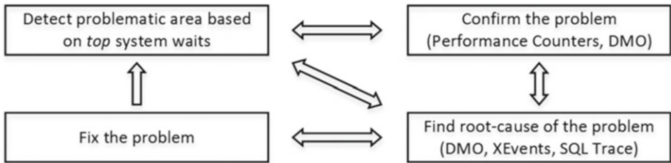
Figure 28-5. Wait statistics analysis troubleshooting cycle
