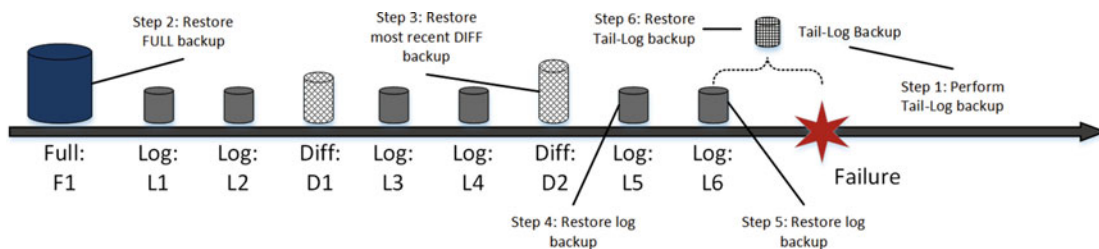
Figure 31-4. Recovery sequence
