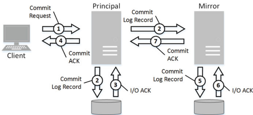
Figure 32-6. Asynchronous commit
