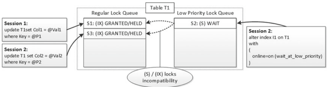
Figure 23-11. Low-priority locks
