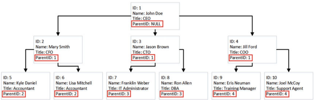
Figure 15-11. Adjacency list
