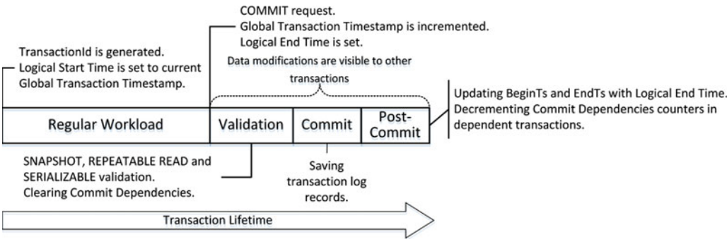
Figure 36-1. Transaction lifetime
