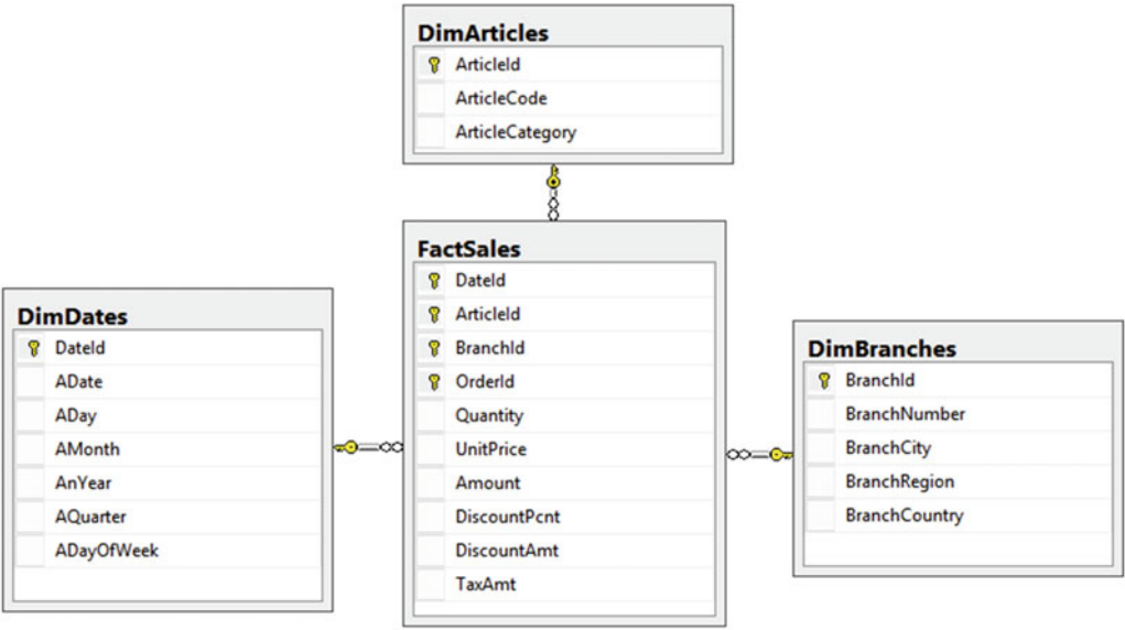
Figure 33-1. Star schema
