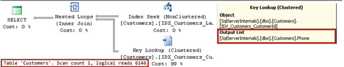
Figure 4-2. Execution plans for the queries
