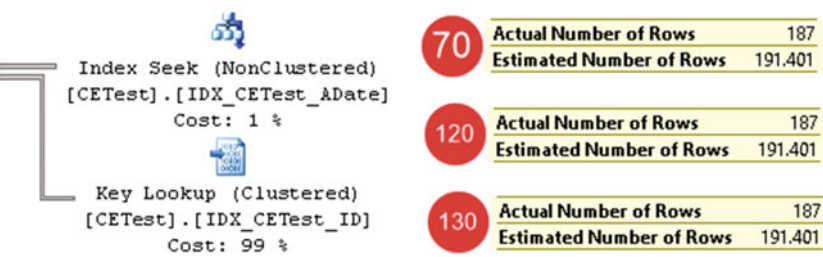
Figure 3-16. Outdated statistics: Cardinality estimations for a value that is a key in the histogram step
