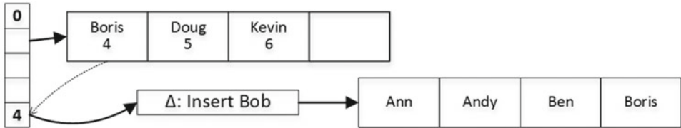
Figure 35-12. Page splitting: Initial state
