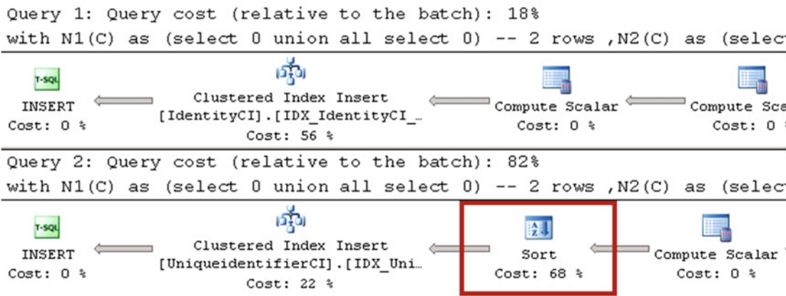
Figure 7-3. Inserting data into the tables: Execution plans
