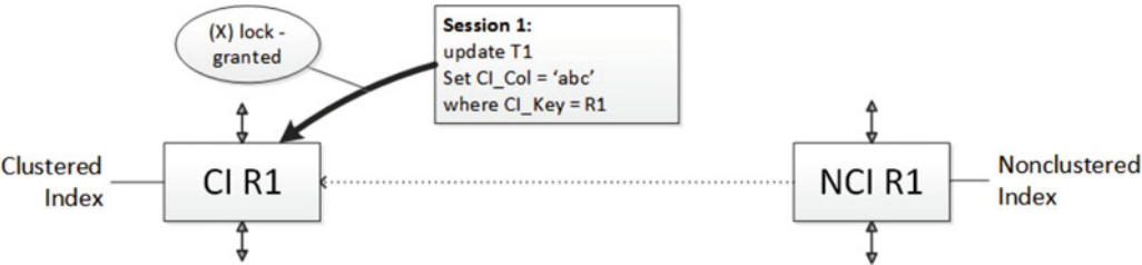
Figure 19-8. Deadlock due to multiple updates of the same row, step 1
