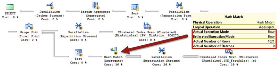
Figure 33-14. Execution plan with clustered index scan in SQL Server 2016 with a database compatibility level of 130
