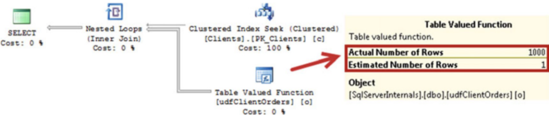
Figure 11-8. Execution plan of query with multi-statement table-valued function (legacy cardinality estimator)
