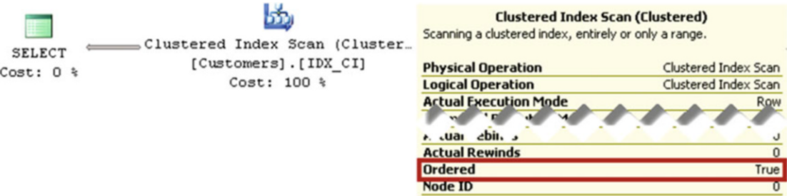
Figure 2-9. Ordered index scan execution plan
