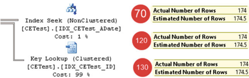
Figure 3-14. Up-to-date statistics: Cardinality estimations for a value that is not a key in the histogram step.
