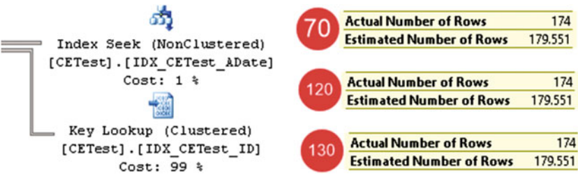
Figure 3-15. Up-to-date statistics: Cardinality estimations for an unknown value
