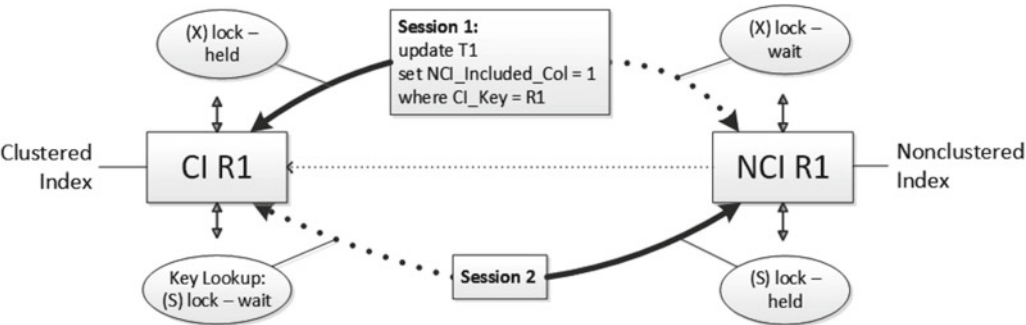
Figure 19-10. Deadlock due to multiple updates of the same row, step 3
