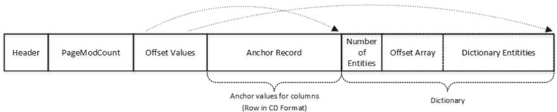
Figure 4-19. Compression information record format
