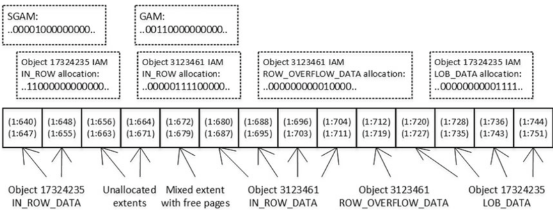
Figure 1-15. Allocation map pages
