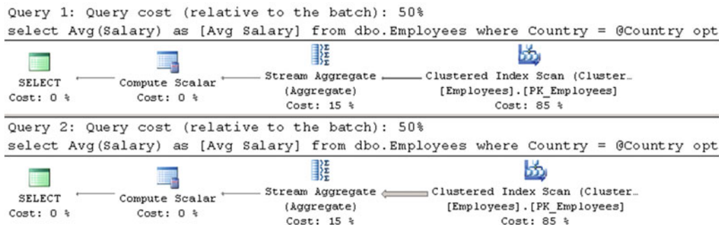
Figure 26-4. Parameter Sniffing: OPTIMIZE FOR hint
