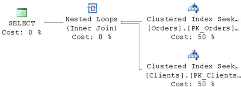
Figure 10-1. Execution plan when selecting all columns from the view
