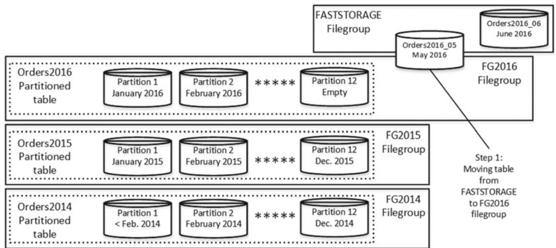
Figure 16-11. Tiered storage in action: Moving the dbo.Orders2016_05 table
