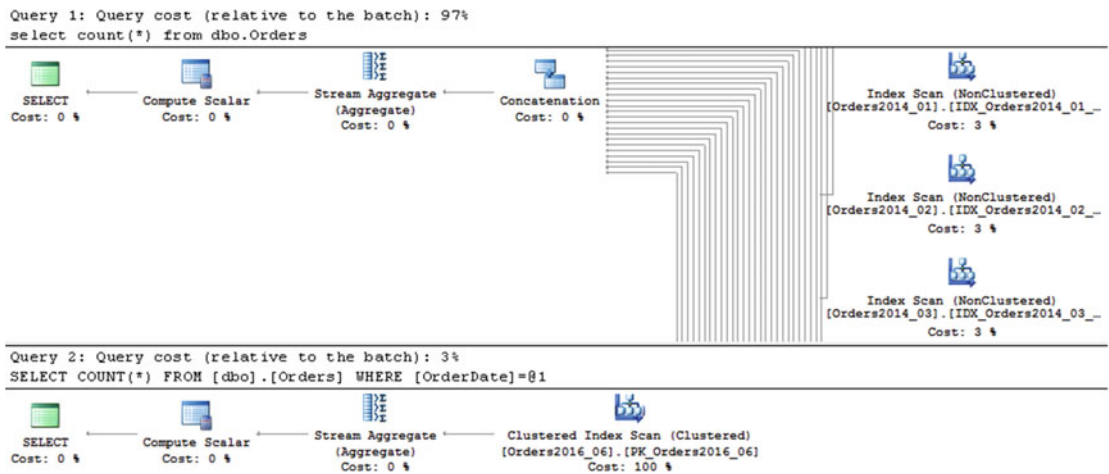
Figure 16-3. Execution plans of the queries against a partitioned view
