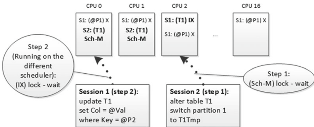
Figure 23-9. Deadlock due to lock partitioning: Step 2
