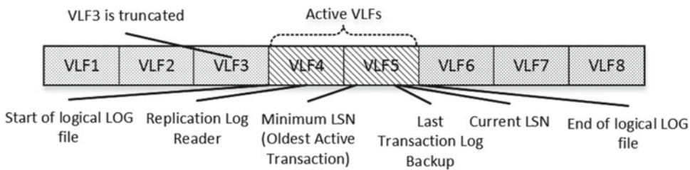
Figure 30-14. FULL and BULK LOGGED recovery models: Log truncation
