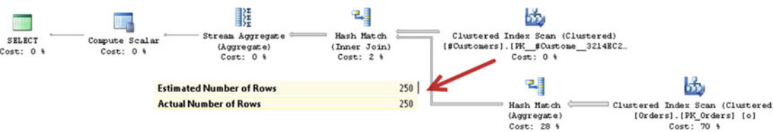
Figure 13-2. Execution plan for a query that uses temporary table
