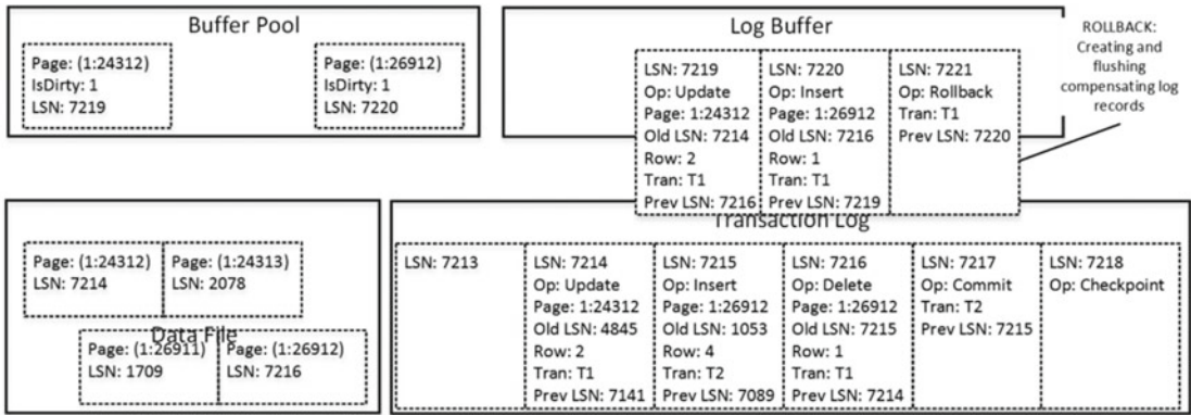
Figure 30-6. Data modifications: ROLLBACK
