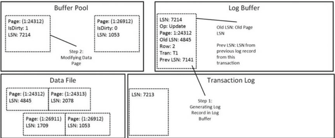
Figure 30-2. Data modifications: T1 updates one of the rows
