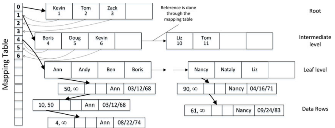
Figure 35-6. Nonclustered index
