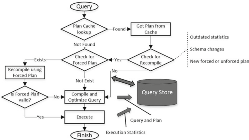
Figure 29-3. Query-processing pipeline
