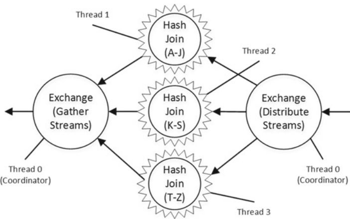
Figure 33-6. Parallelism in row mode execution
