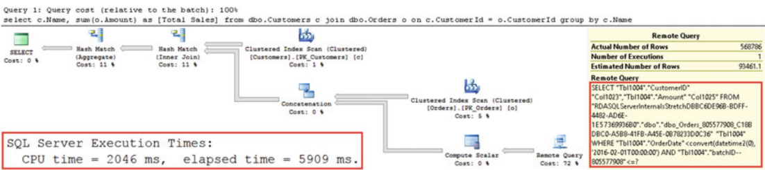
Figure 5-11. Execution plan: Total sales on per-customer basis
