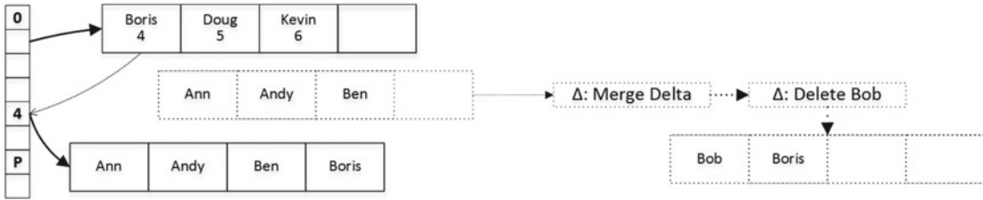
Figure 35-17. Page merging: Third (final) step
