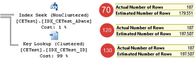
Figure 3-18. Outdated statistics: Cardinality estimations for an unknown value
