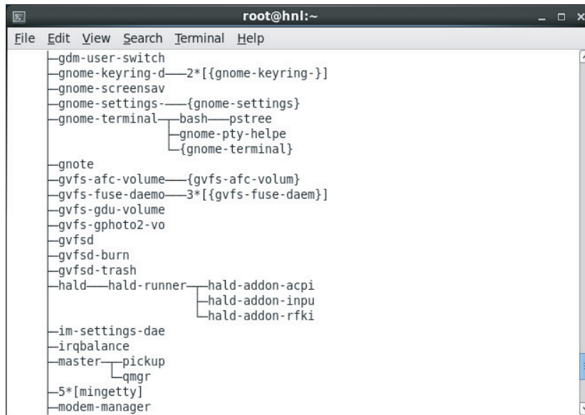
FIGURE 18.1 Use pstree to show that commands are run as a subshell.
