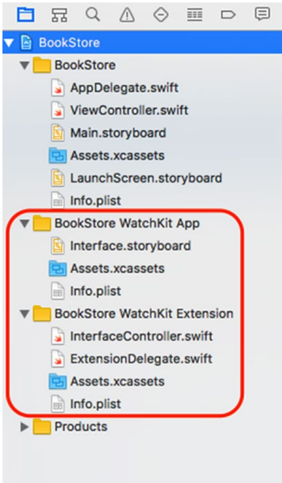
Figure 15-3. New targets
