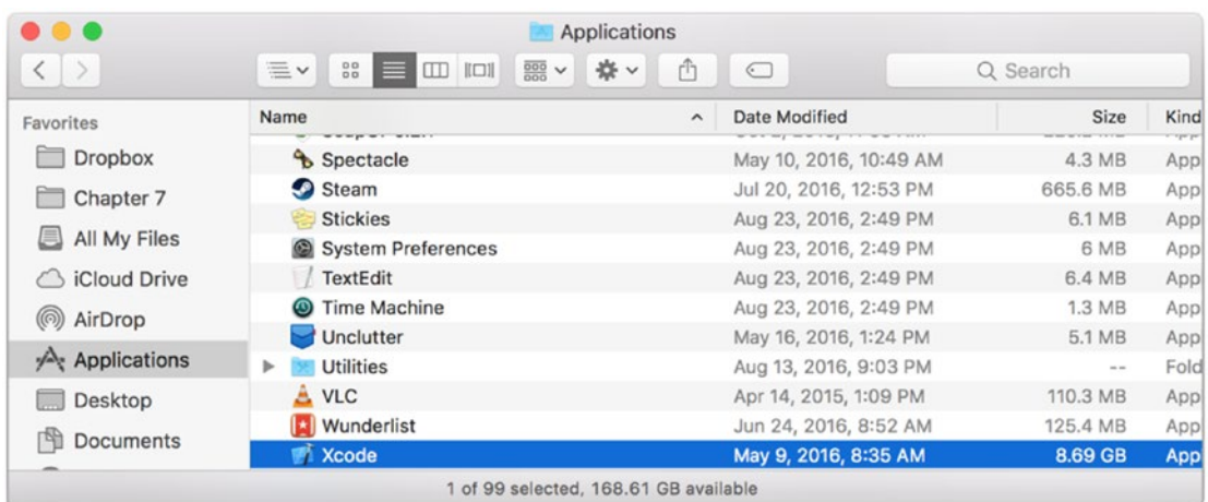
Figure 9-1. Launching Xcode
