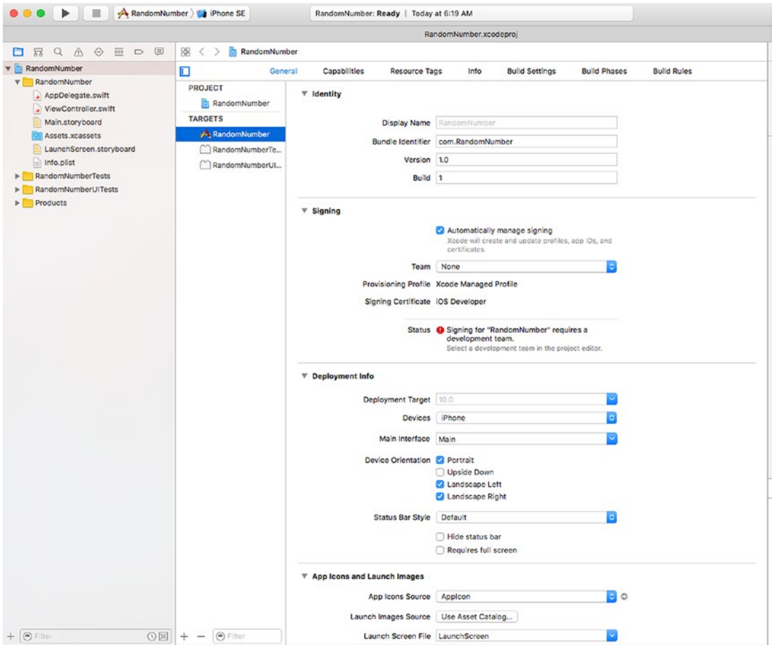
Figure 10-7. Source files
