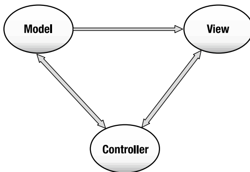
Figure 10-2. MVC paradigm
