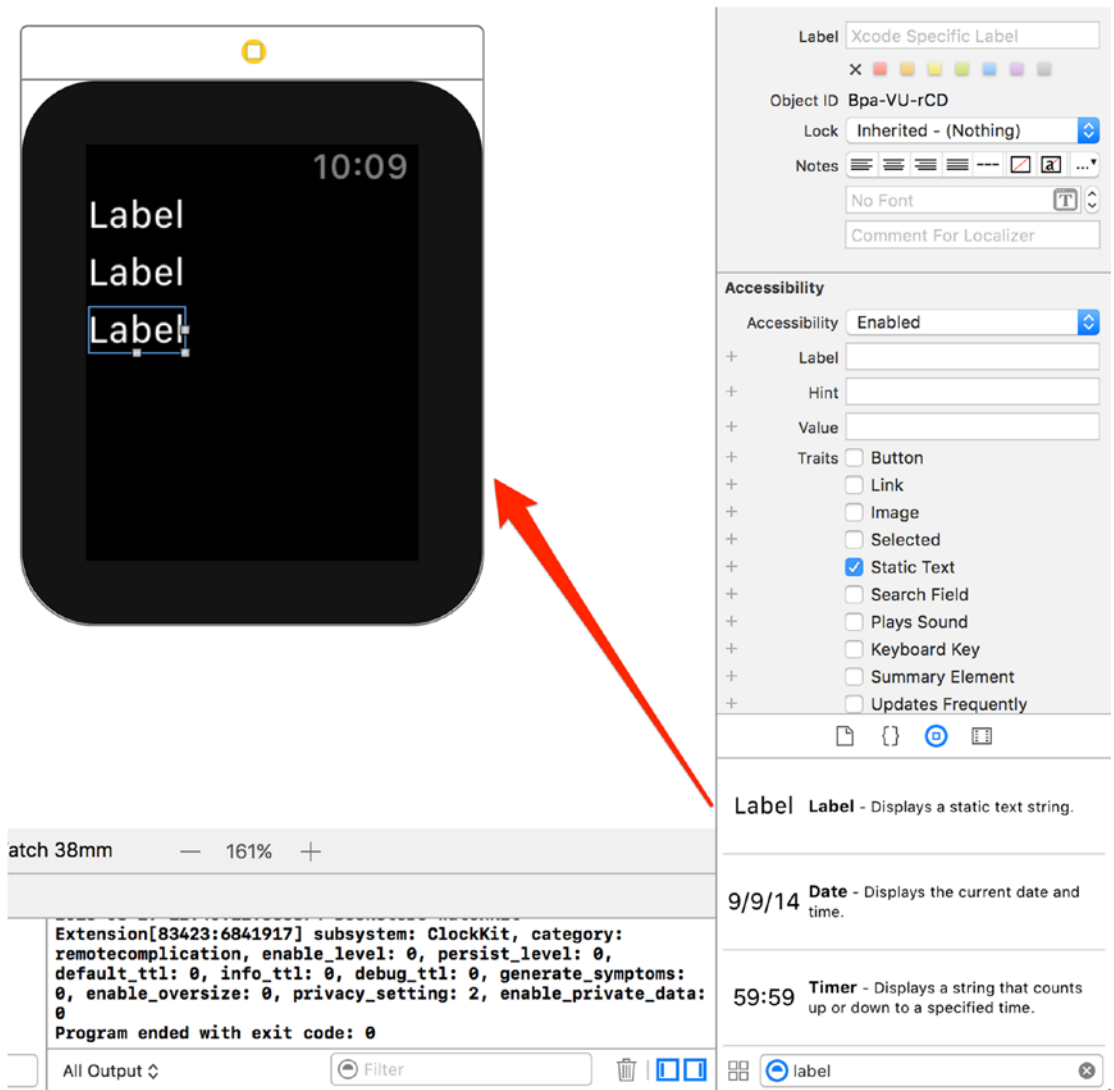
Figure 15-26. New labels
