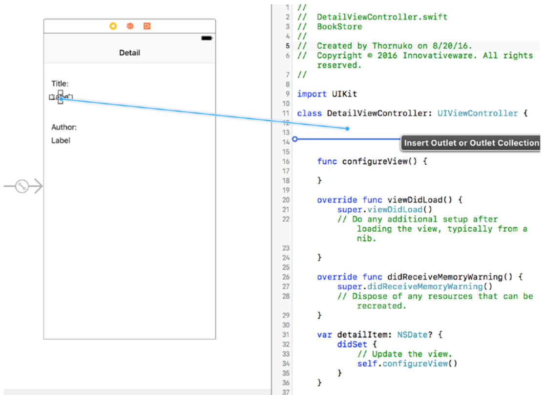
Figure 8-10. Creating variables
