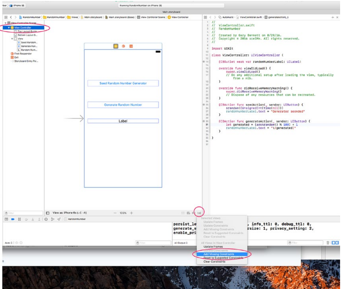
Figure 10-23. Auto Layout
