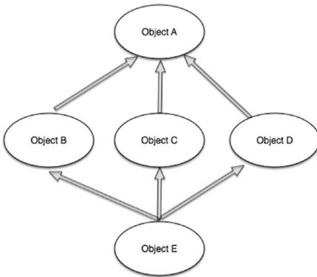
Figure 12-2. Multiple inheritance
