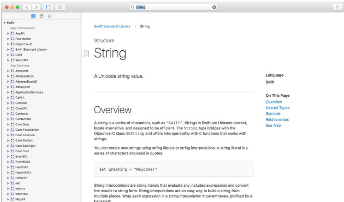
Figure 7-25. Xcode documentation
