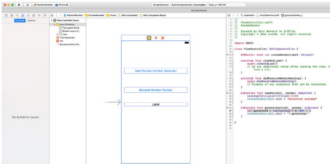
Figure 10-1. Interface Builder
