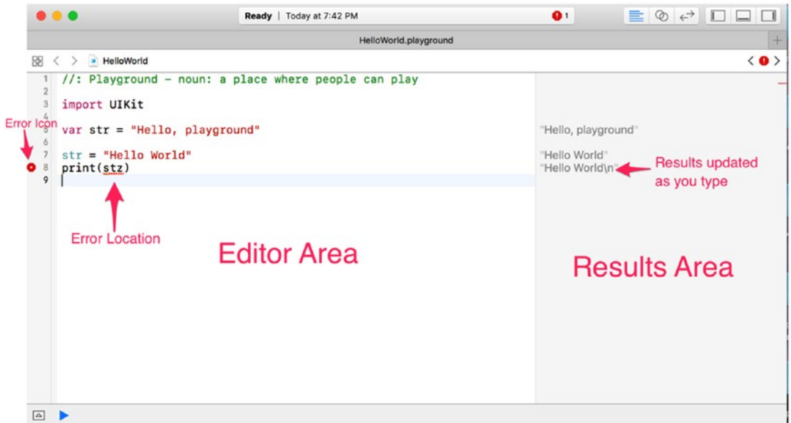
Figure 2-9. The playground with a syntax error caught by the Swift compiler
