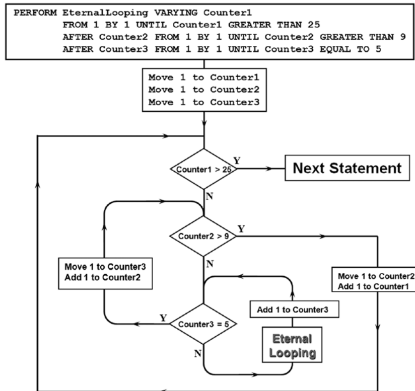
Figure 12-17. Flowchart showing how the three-counter PERFORM...VARYING works
