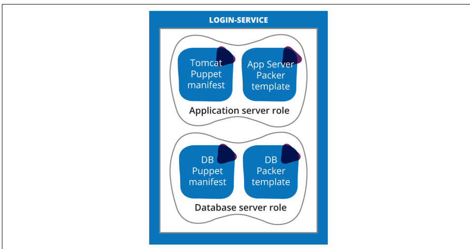
Figure 11-4. LoginService architecture
