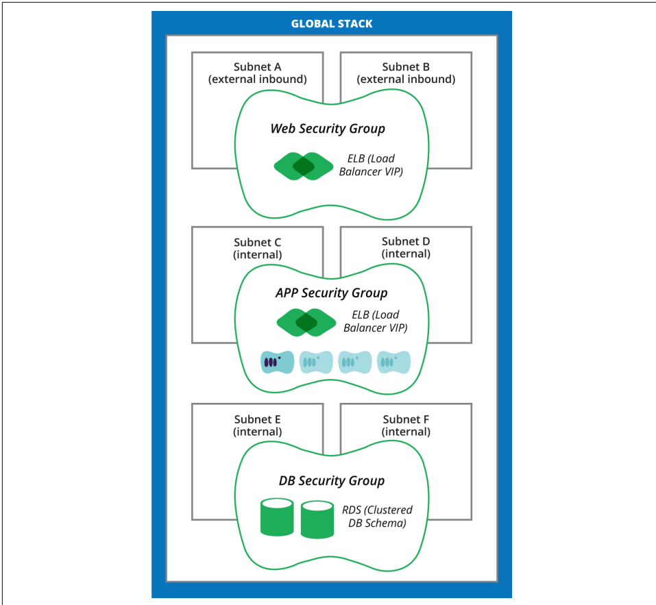
Figure 9-7. Microservice application stack
