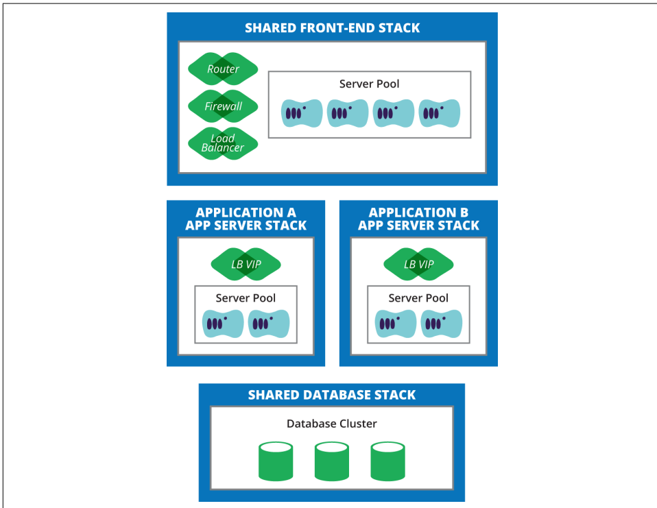
Figure 9-4. Two application environments sharing stacks
