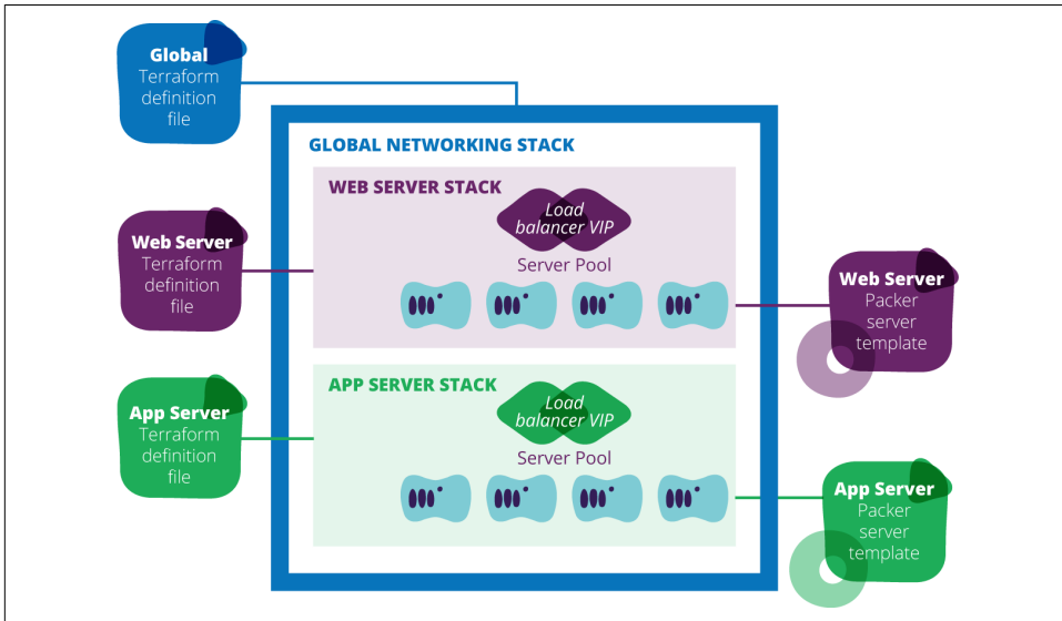
Figure 12-4. An example environment with its components
