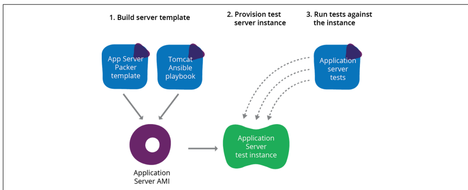
Figure 11-7. Flow for testing the LoginService application server
