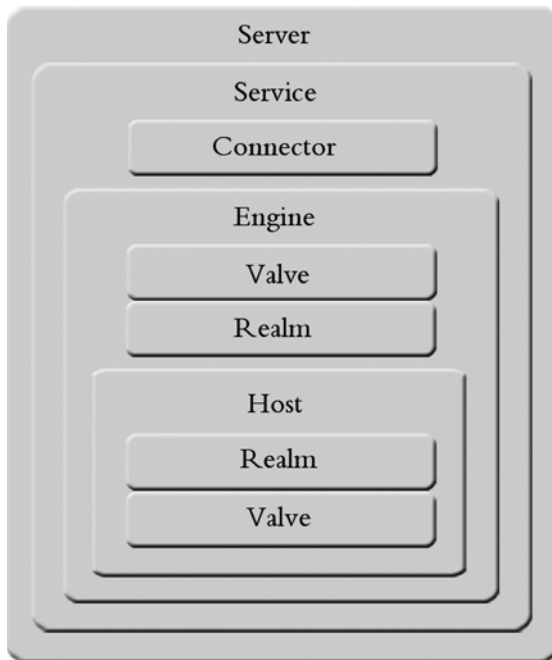
Figure 5.3 Different components in the server.xml file can be nested inside of one another.
