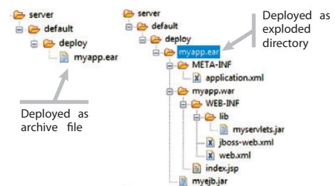
Figure 3.1 Deploying an archive file vs. an exploded directory
