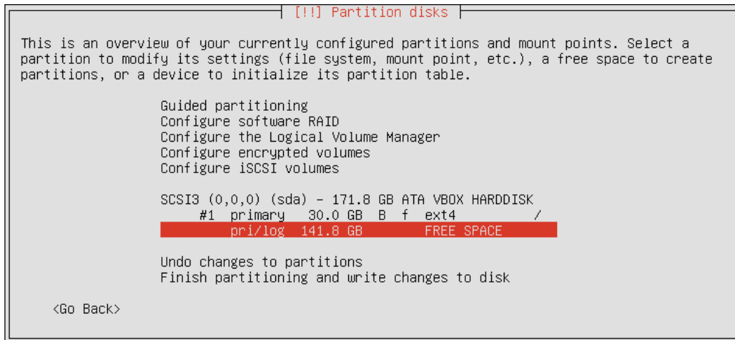
Preparing to create a second partition
