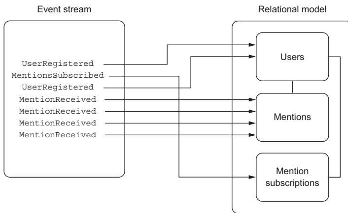
Figure 7.4 Mapping the Event Stream to the relational model with the CQRSEventHandler
