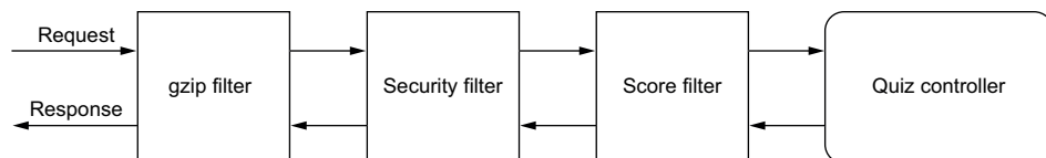
Figure 4.6 Filter chain that alters the default behavior on requests or results
