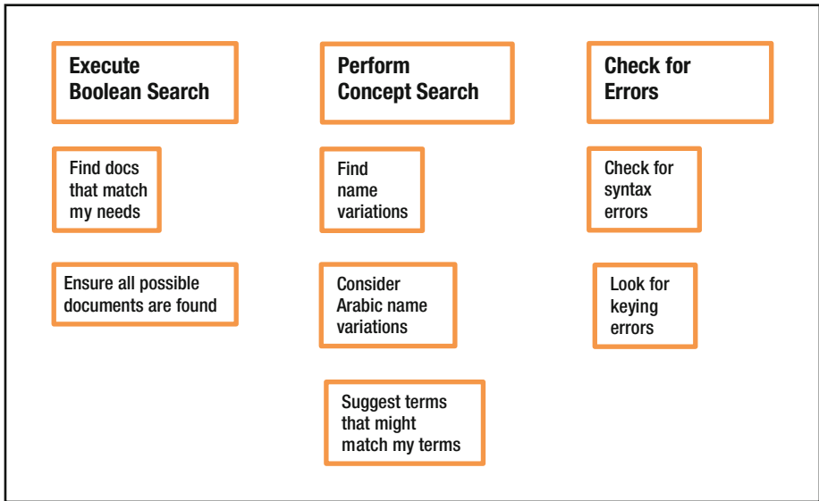
Figure 12-5. Affinity diagram 2
