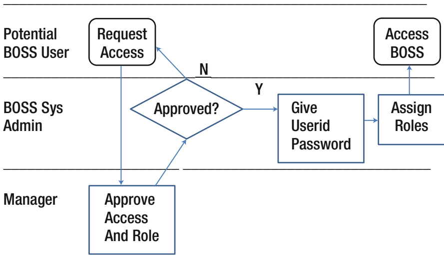
Figure 12-1. Swim lanes
