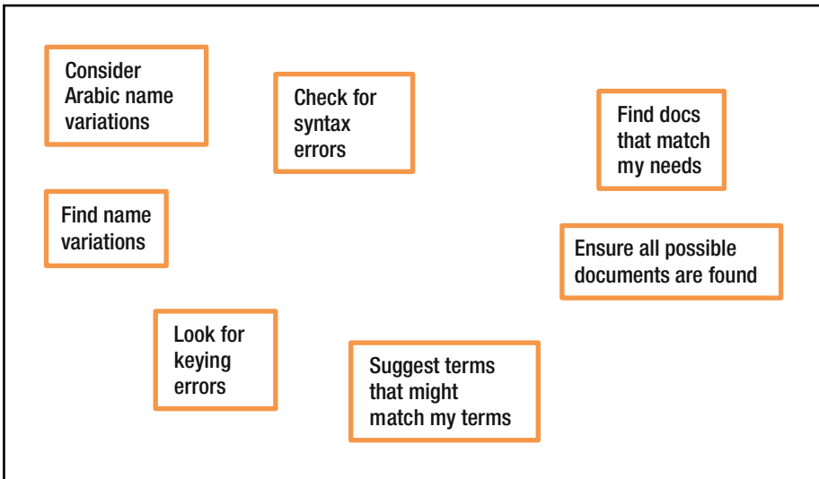
Figure 12-4. Affinity diagram 1
