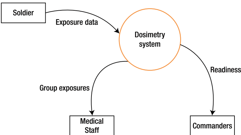
Figure 12-2. Context diagram
