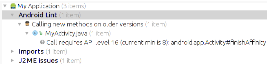
Figure 831: Android Studio Inspection Results
