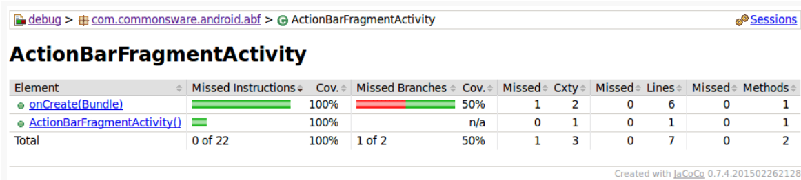
Figure 303: Jacoco Coverage Report, Class Level
