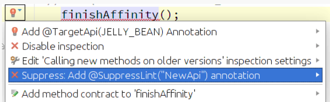
Figure 832: Android Studio Lint Fix Suggestions
