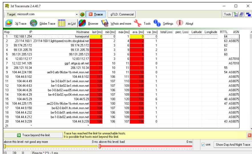
FIGURE 5-28: Why is the Internet so slow? 3d Traceroute pinpoints pileups.
