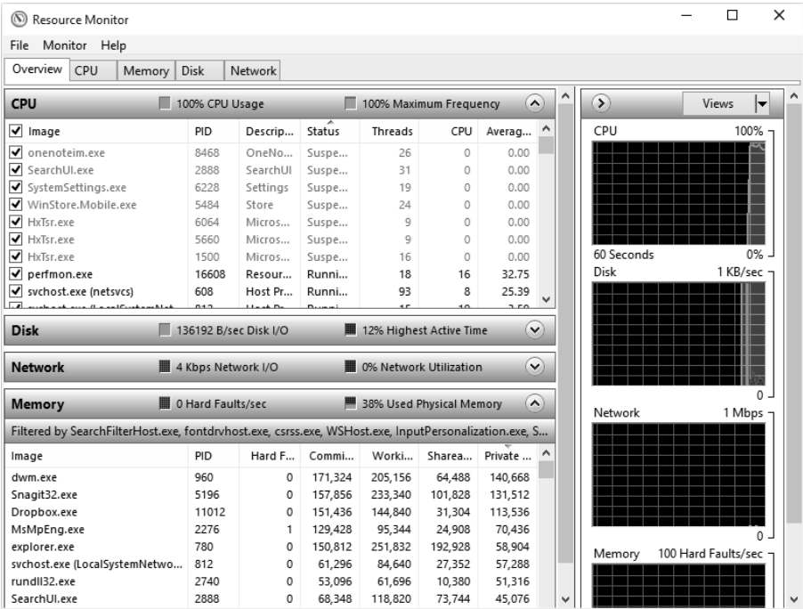
FIGURE 36.13 Resource Monitor.
