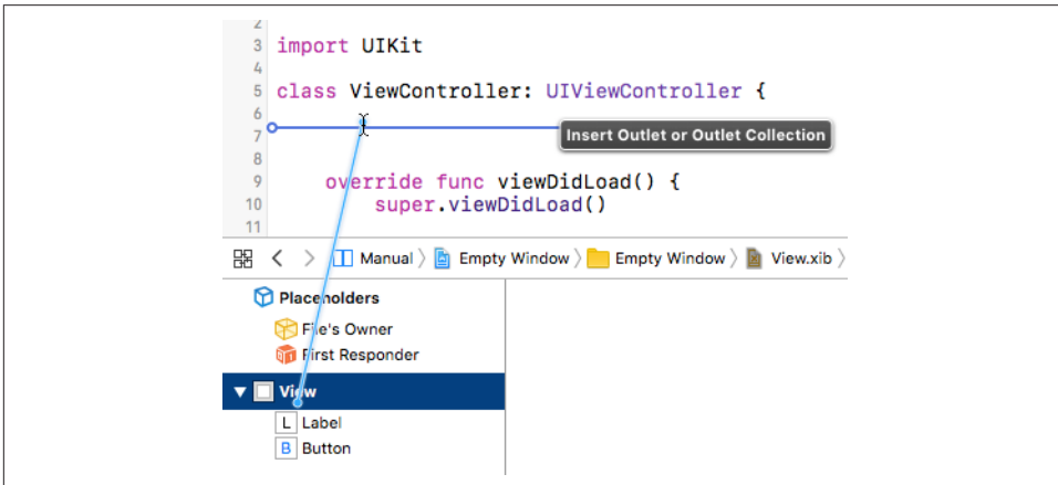
Figure 7-14. Creating an outlet by dragging from nib editor to code
