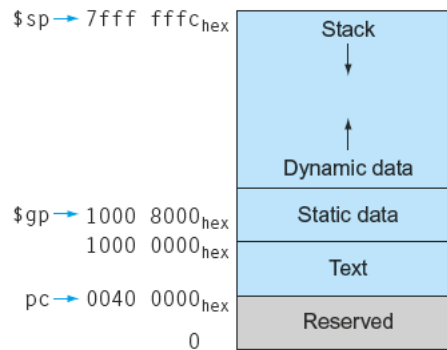
FIGURE 2.13 The MIPS memory allocation for program and data. These addresses are only a software convention, and not part of the MIPS architecture. The stack pointer is initialized to 7\text{fff}\text{fffc}_{\text{hex}} and grows down toward the data segment. At the other end, the program code (“text”) starts at 0040\text{ }0000_{\text{hex}} . The static data starts at 1000\text{ }0000_{\text{hex}} . Dynamic data, allocated by malloc in C and by new in Java, is next. It grows up toward the stack in an area called the heap. The global pointer, $gp , is set to an address to make it easy to access data. It is initialized to 1000\text{ }8000_{\text{hex}} so that it can access from 1000\text{ }0000_{\text{hex}} to 1000\text{ }ffff_{\text{hex}} using the positive and negative 16-bit offsets from $gp . This information is also found in Column 4 of the MIPS Reference Data Card at the front of this book.
