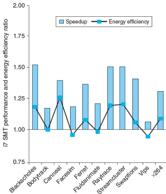
FIGURE 6.6 The speed-up from using multithreading on one core on an 17 processor averages 1.31 for the PARSEC benchmarks (see Section 6.9 ) and the energy efficiency improvement is 1.07. This data was collected and analyzed by Esmaeilzadeh et. al. [2011].
