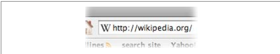
Figure 10-14. Wikipedia favicon
