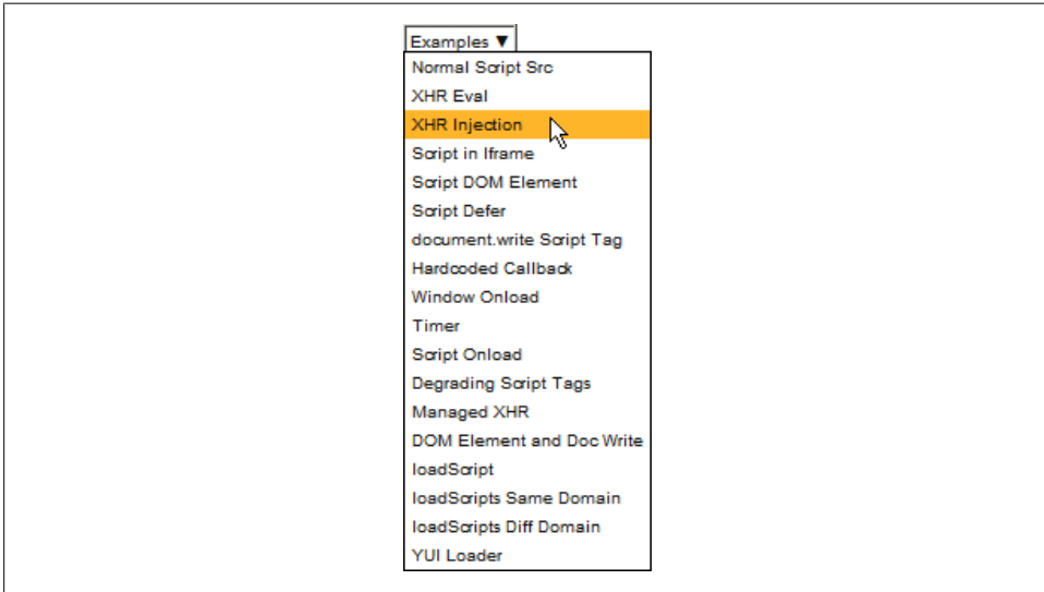
Figure 5-1. menu.js example
