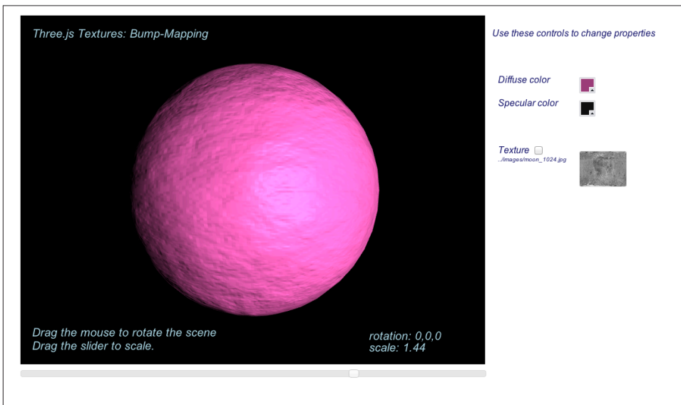
Figure 4-9. Bump mapping
