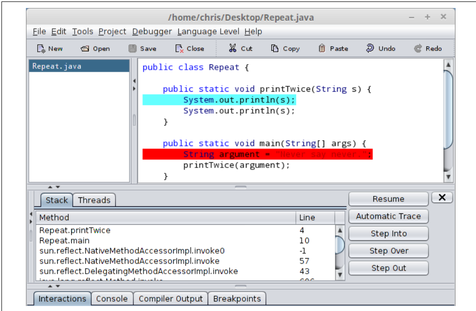
Figure A-5. Screenshot of the DrJava debugger. Execution is currently paused on the first line of printTwice . There is a breakpoint on the first line of main .
